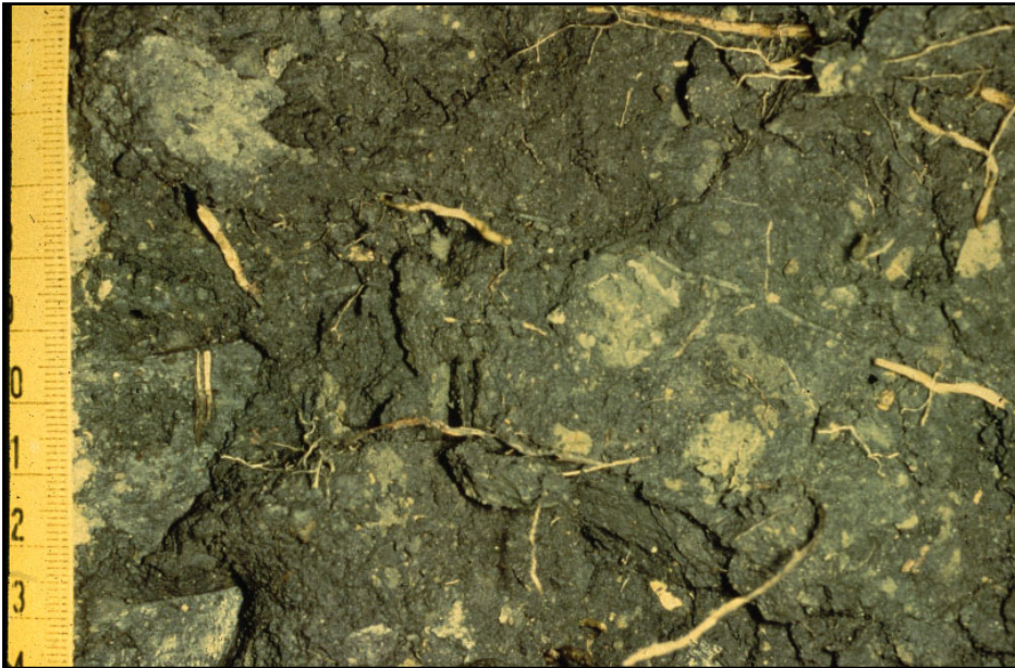
Figure 3-22. Depletions are the lighter areas (high value and low chroma) within the dark matrix of the surface layer. Scale is in inches.
