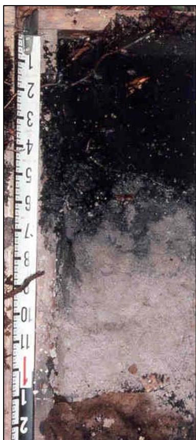
Figure 3-16. In this soil, the splotchy pattern below the dark surface is due to mobilization and translocation of organic matter. Scale in inches.
