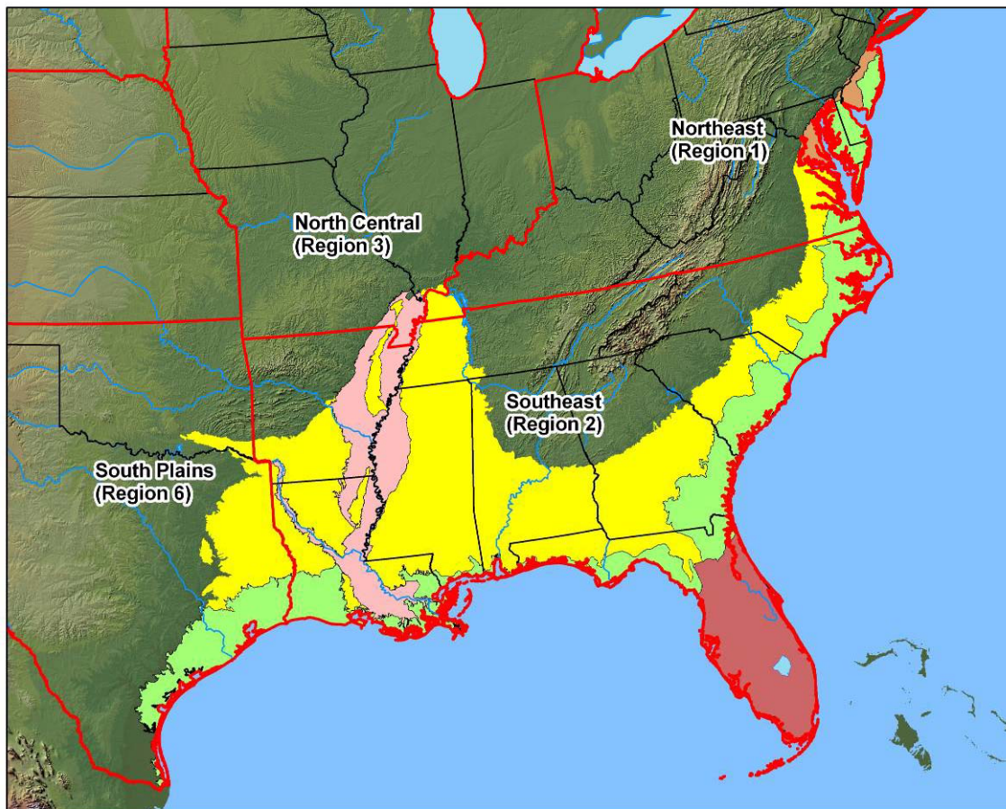
Figure 2-1. Plant list regional boundaries (red lines) currently used by the U.S. Fish and Wildlife Service, National Wetlands Inventory, in the Atlantic and Gulf Coastal Plain Region.
