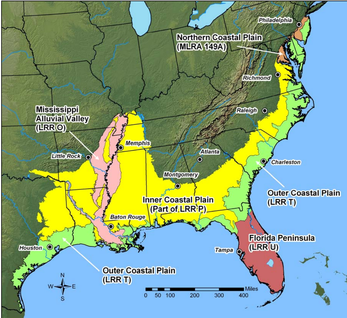
Figure 1. Approximate boundaries of the Atlantic and Gulf Coastal Plain Region. This supplement is applicable throughout the highlighted areas, although some indicators may be restricted to specific subregions or smaller areas. See text for details.
