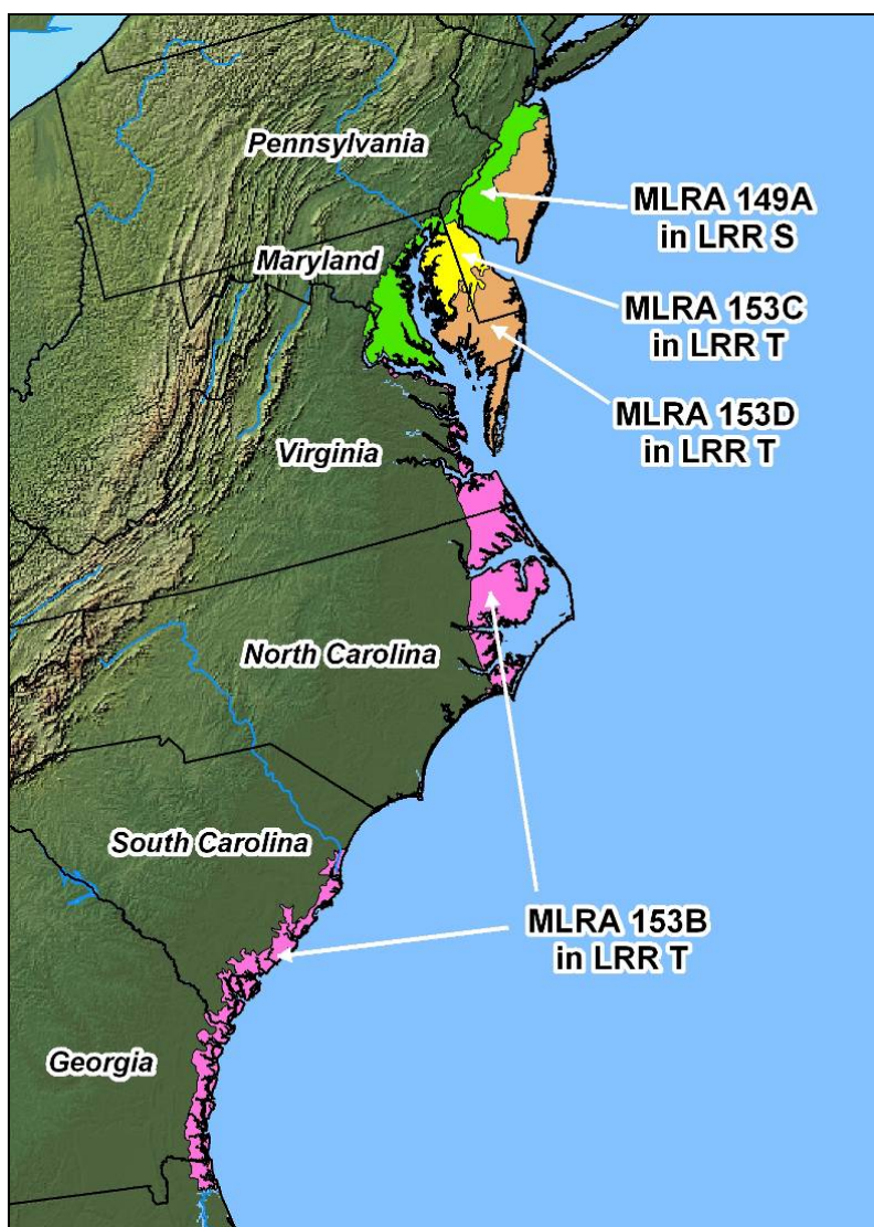
Figure 3-29. Locations of MLRAs 149A, 153B, 153C, and 153D.
