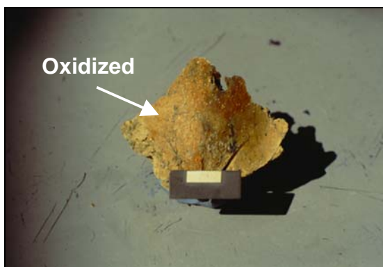
Figure 5-9. The same soil as in Figure 5-8 after exposure to the air and oxidation has occurred.
