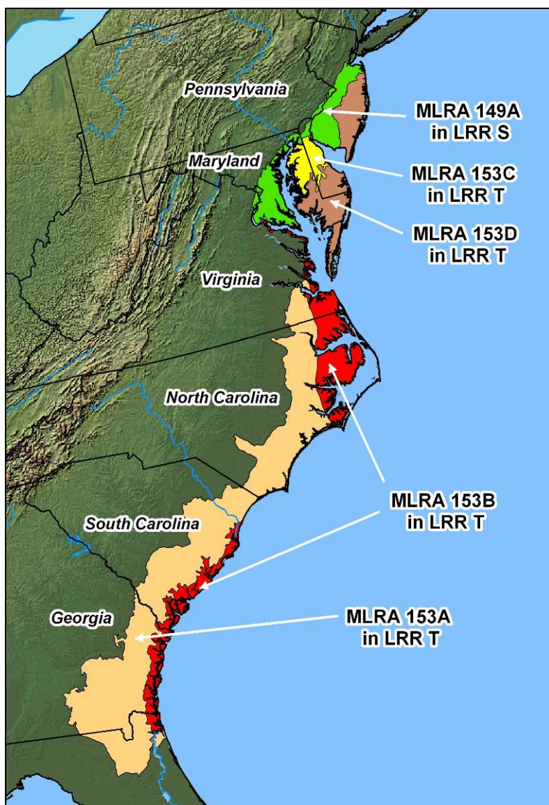
Figure 5-5. Locations of MLRAs 149A, 153A, 153B, 153C, and 153D.
