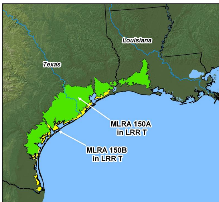
Figure 3-28. Location of MLRAs 150A and 150B.
