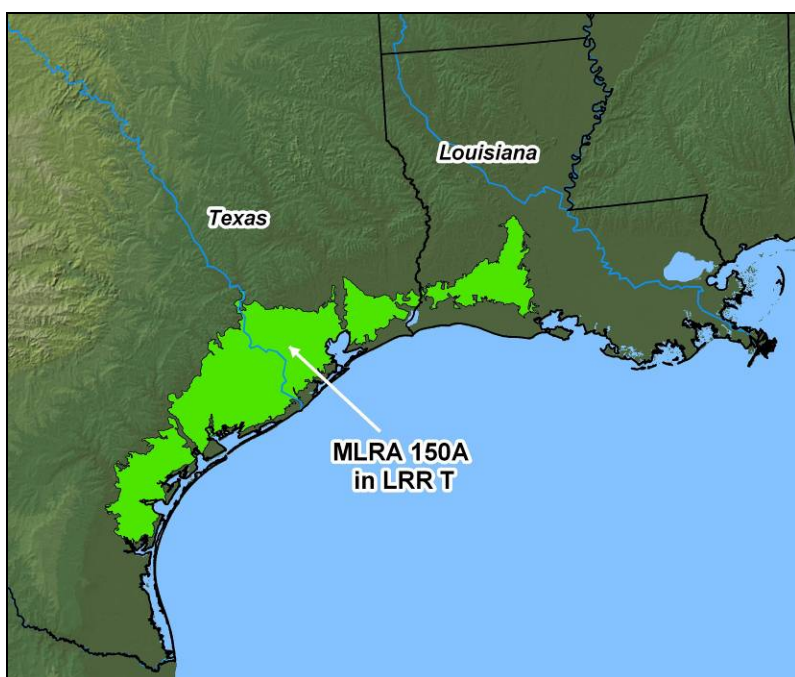
Figure 3-11. Location of MLRA 150A.
