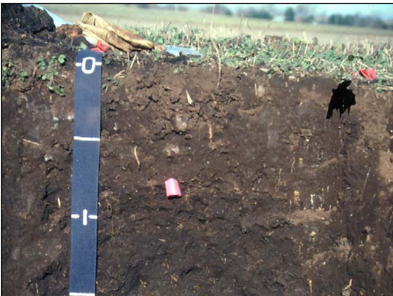
Figure 5-3. Black parent materials can mask redoximorphic features.
