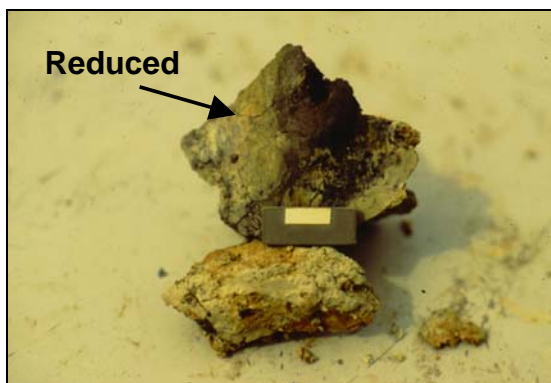
Figure 5-8. This soil exhibits colors associated with reducing conditions. Scale is 1 cm.
