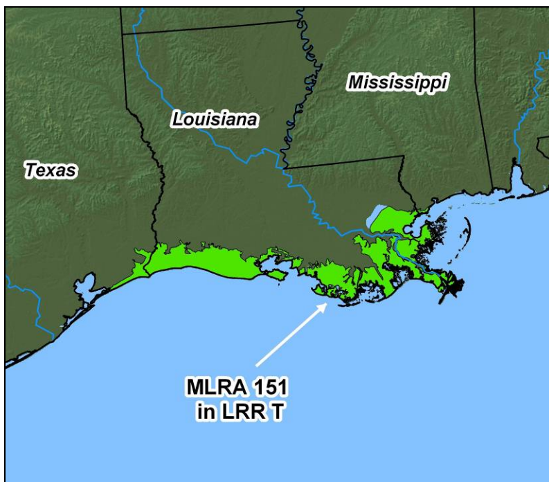
Figure 3-25. Location of MLRA 151 in LRR T.
