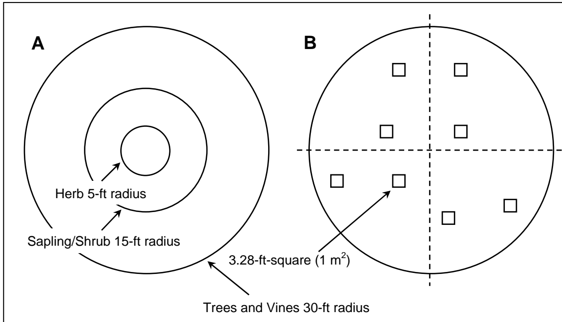
Figure 2. Suggested plot arrangements for vegetation sampling. (A) Single plots in graduated sizes. (B) Nested 3.28- by 3.28-ft square ( 1\text{ m}^2 ) plots for herbs within the 30-ft radius plot.
