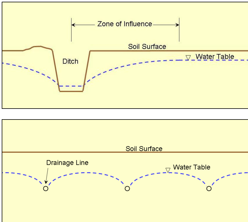
Figure 61. Effects of ditches (upper) and parallel subsurface drainage lines (lower) on the water table.
