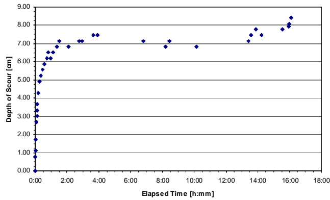
Figure C50. Scour depth vs. time.
