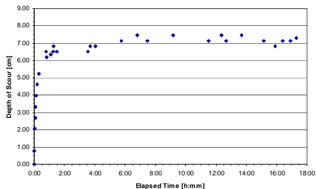
Figure C43. Scour depth vs. time.
