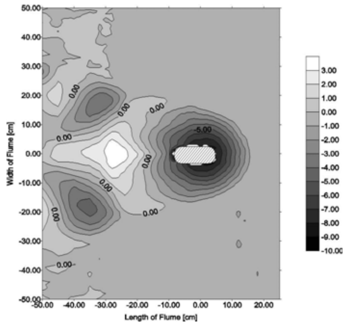
Figure C27. Contour plot; flow from right to left.
