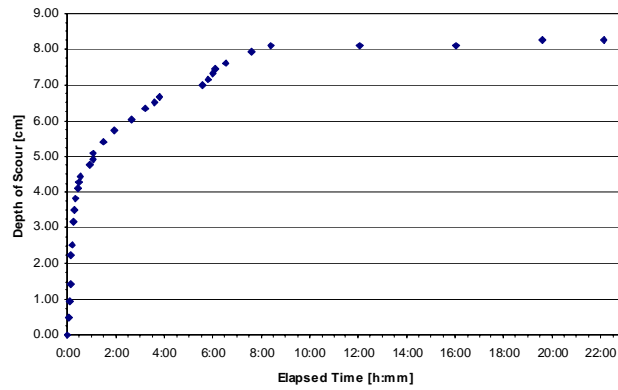
Figure B8. Scour depth vs. time.
