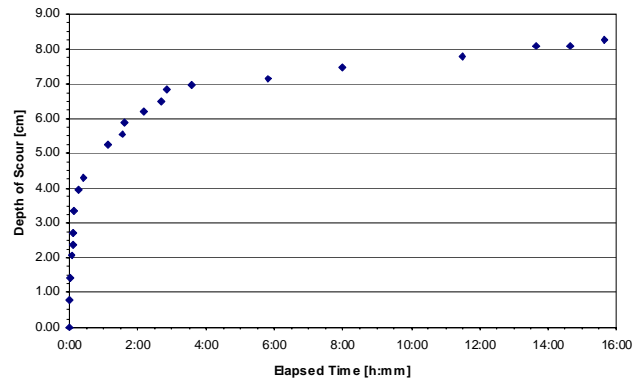
Figure C29. Scour depth vs. time.
