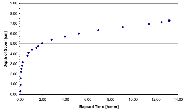
Figure A35. Scour depth vs. time.
