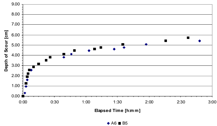
Figure 42. Scour depth vs. time (first 3 hours) for Tests A6 and B5, V_{avg} = 0.700 ft/s (21.34 cm/s).
