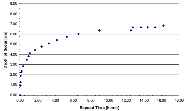
Figure A28. Scour depth vs. time.
