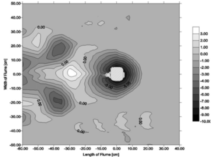
Figure A26. Contour plot; flow from right to left.
