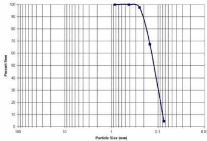
Figure 7. Grain size distribution for flume sediment.
