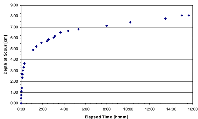
Figure C36. Scour depth vs. time.
