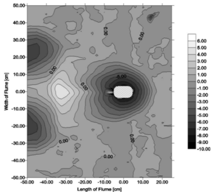
Figure B13. Contour plot; flow from right to left.
