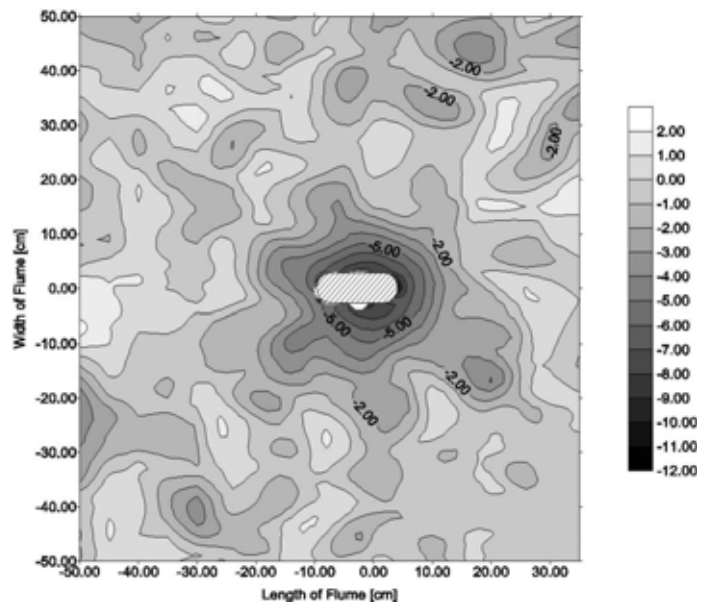
Figure C20. Contour plot; flow from right to left.
