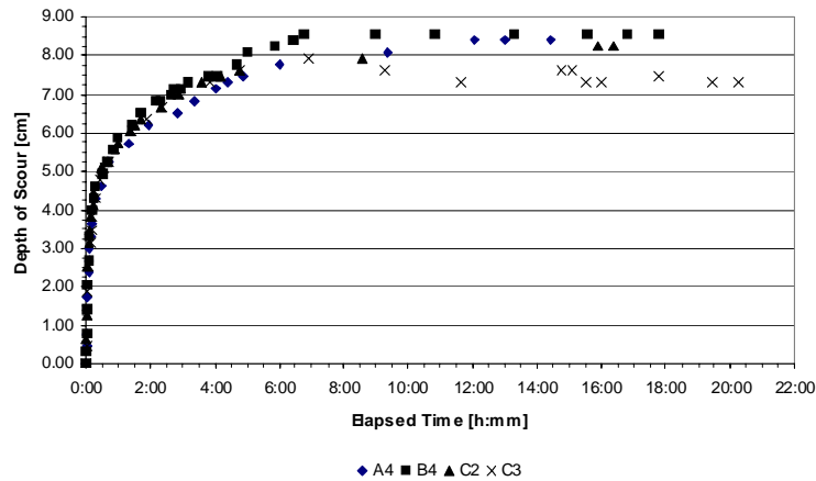
Figure 47. Scour depth vs. time for Tests A4, B4, C2, and C3, V_{avg} = 0.836 ft/s (25.48 cm/s).
