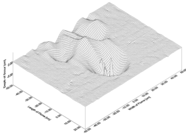
Figure B35. Surface plot; flow is from lower right to upper left.
