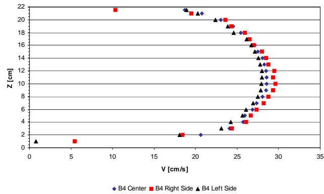
Figure B24. Velocity profiles.
