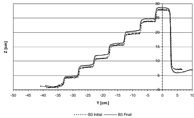
Figure B18. Calibration.
