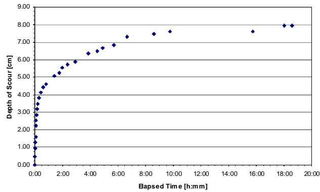
Figure C1. Scour depth vs. time.
