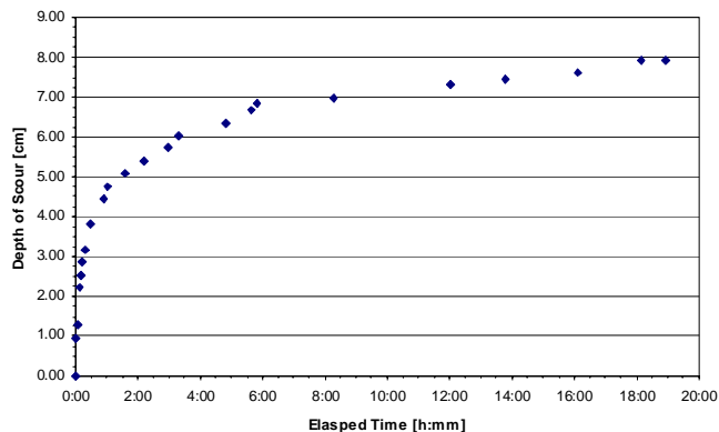
Figure C22. Scour depth vs. time.
