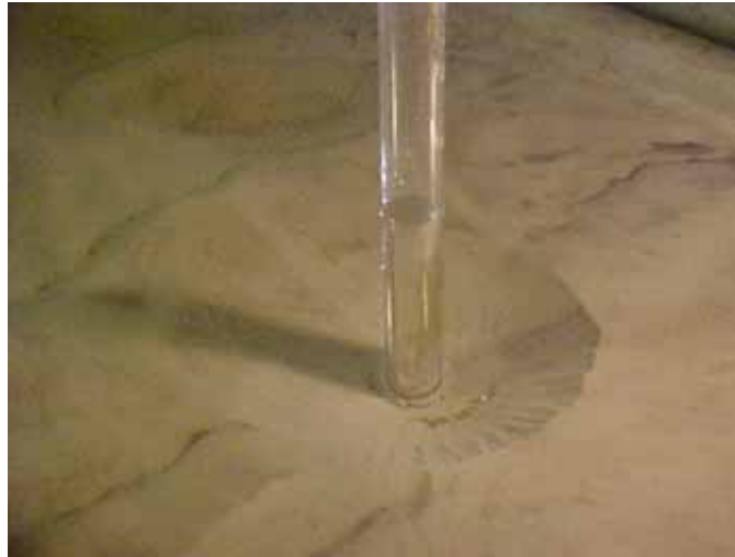
Figure C5. Final photo of scour hole; flow from right to left.
