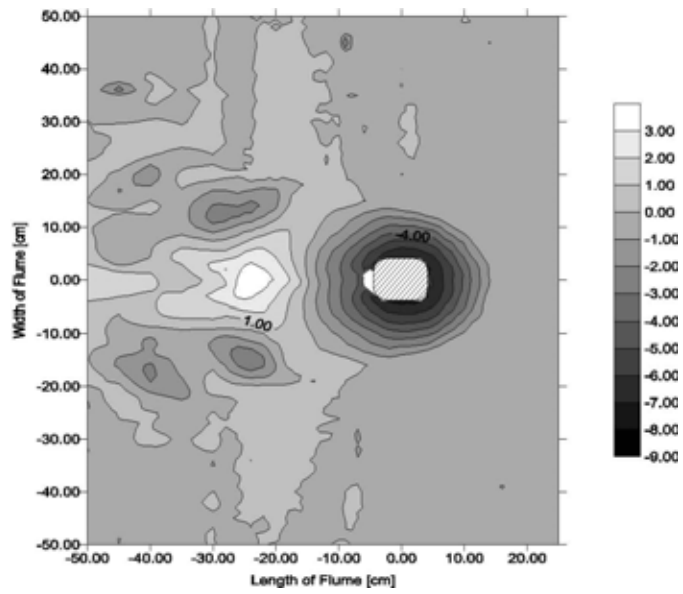
Figure A40. Contour plot; flow from right to left.
