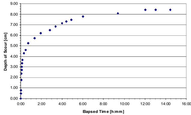
Figure A21. Scour depth vs. time.
