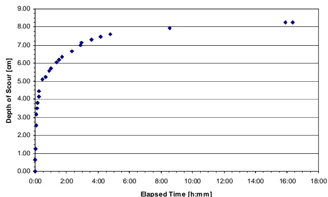
Figure C8. Scour depth vs. time.
