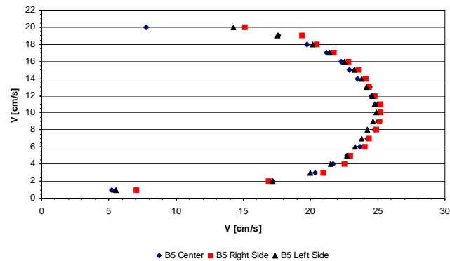
Figure B31. Velocity profiles.
