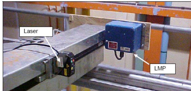
Figure 23. Laser distance measuring system with the attached LMP.
