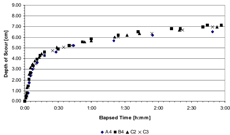
Figure 48. Scour depth vs. time (first 3 hours) for Tests A4, B4, C2, and C3, V_{avg} = 0.836 ft/s (25.48 cm/s).
