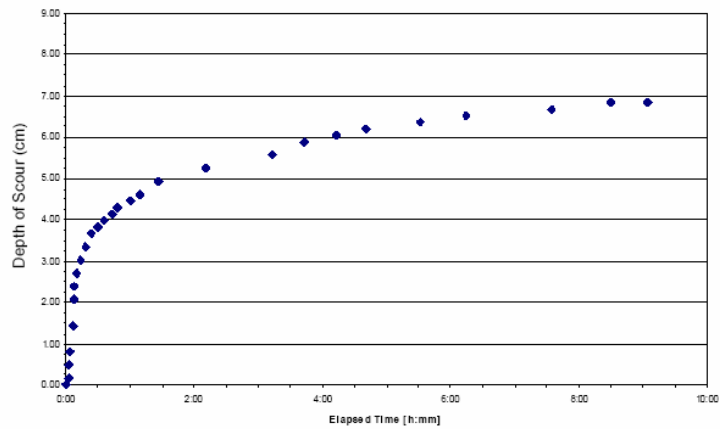
Figure A14. Scour depth vs. time.
