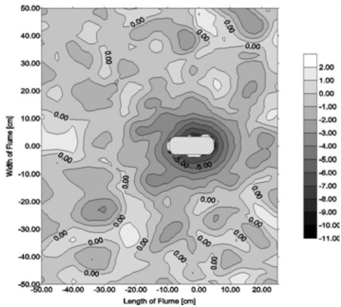
Figure C48. Contour plot; flow from right to left.
