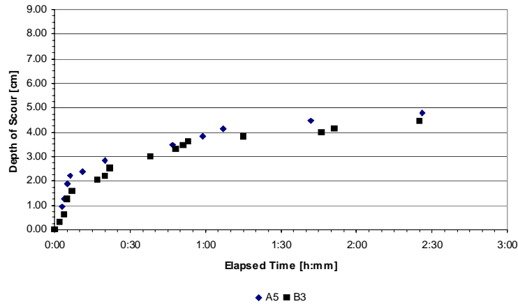
Figure 40. Scour depth vs. time (first 3 hours) for Tests A5 and B3, V_{avg} = 0.650 ft/s (19.8 cm/s).
