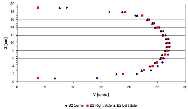
Figure B10. Velocity profiles.
