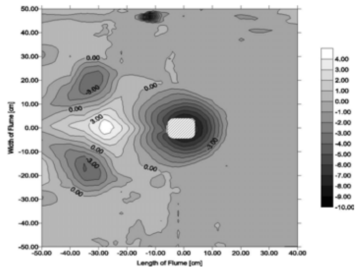
Figure A12. Contour plot; flow from right to left.
