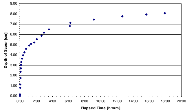
Figure A7. Scour depth vs. time.
