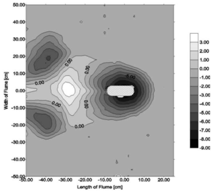
Figure C34. Contour plot; flow from right to left.
