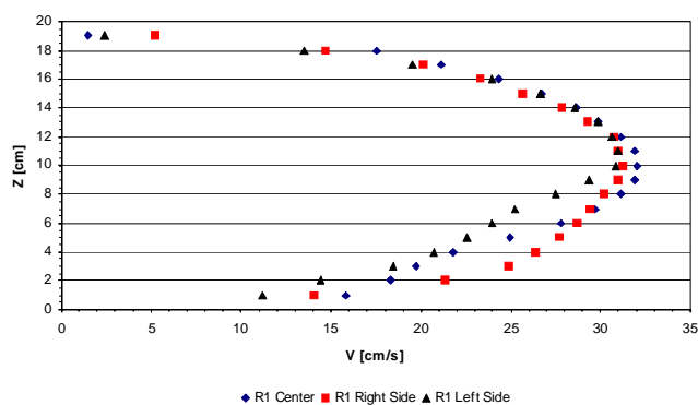
Figure B38. Velocity profiles.
