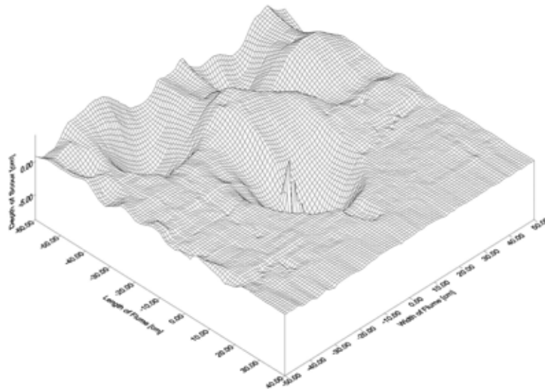
Figure B28. Surface plot; flow is from lower right to upper left.
