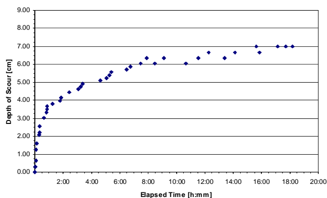
Figure B15. Scour depth vs. time.
