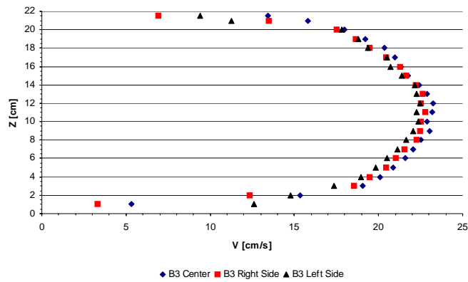
Figure B17. Velocity profiles.
