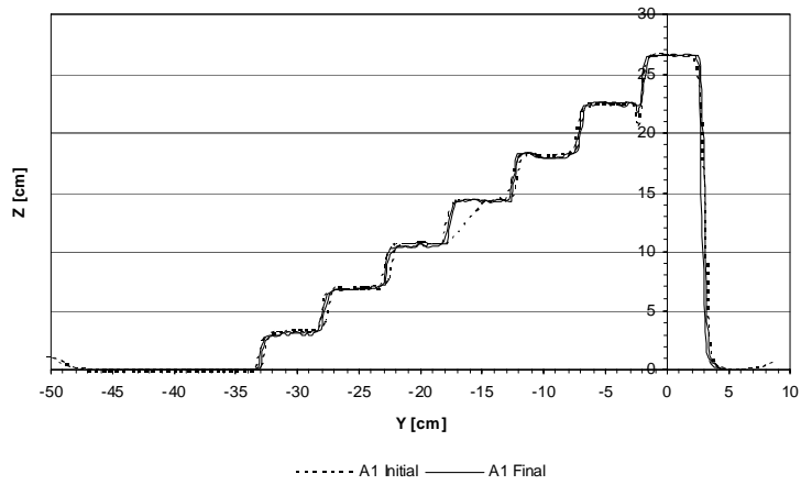
Figure A3. Calibration.
