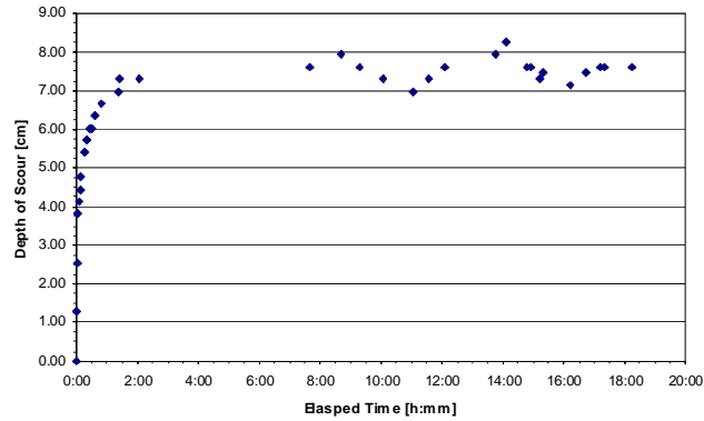
Figure B36. Scour depth vs. time.
