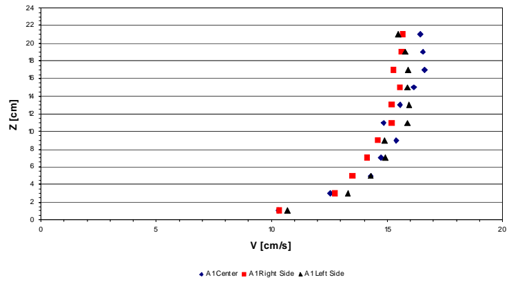
Figure A2. Velocity profiles.
