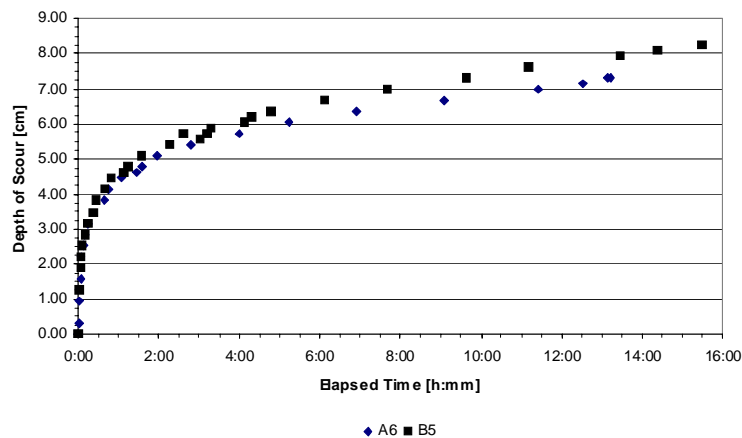
Figure 41. Scour depth vs. time for Tests A6 and B5, V_{avg} = 0.700 ft/s (21.34 cm/s).
