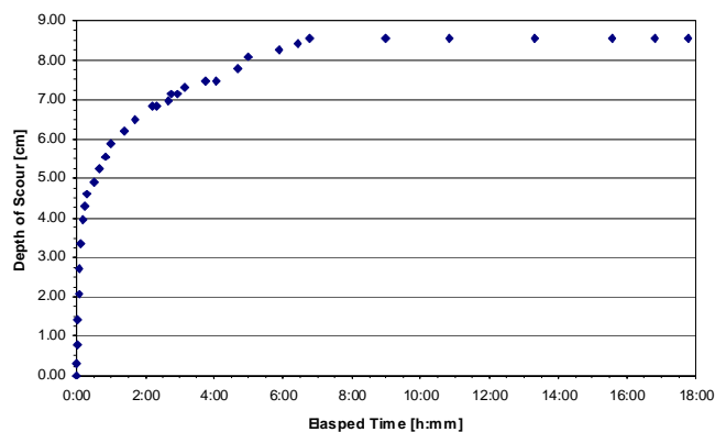
Figure B22. Scour depth vs. time.
