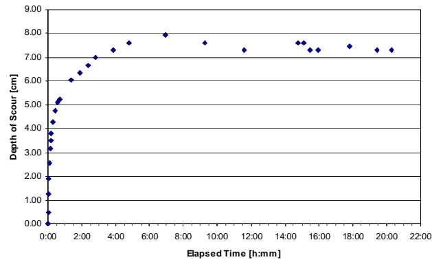
Figure C15. Scour depth vs. time.
