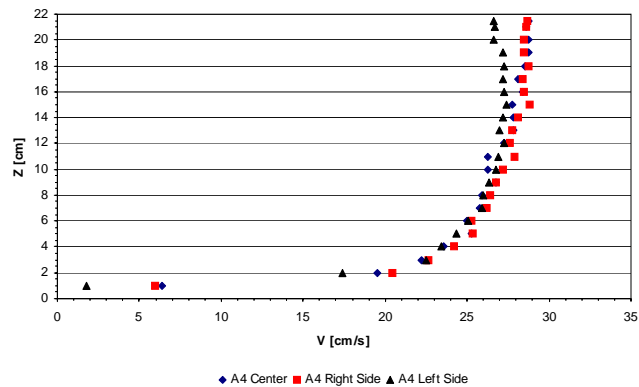
Figure A23. Velocity profiles.
