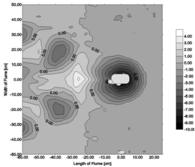
Figure C6. Contour plot; flow from right to left.
