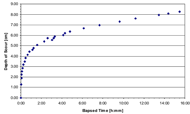
Figure B29. Scour depth vs. time.
