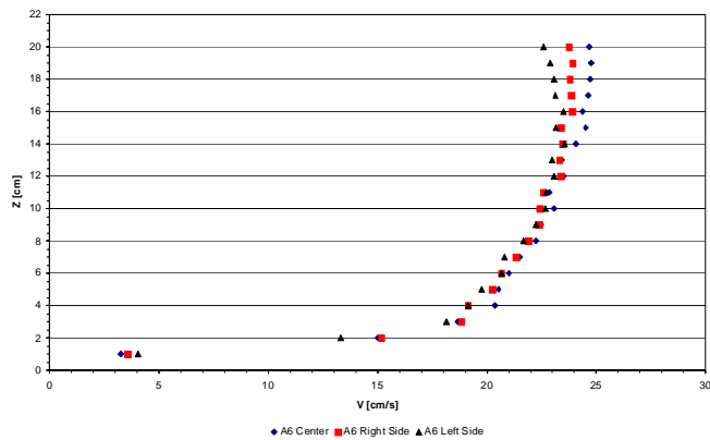
Figure A37. Velocity profile.
