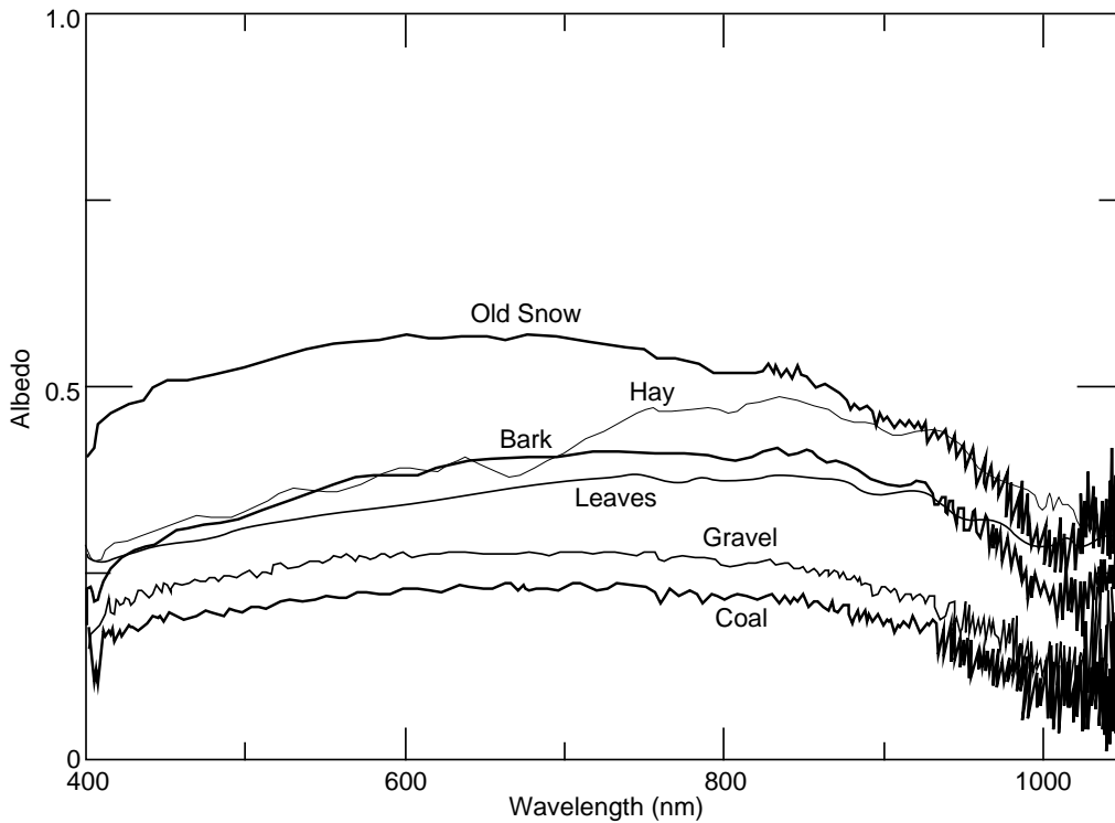
Figure 4. Albedo measurements of the dusted surfaces (March 1994).
