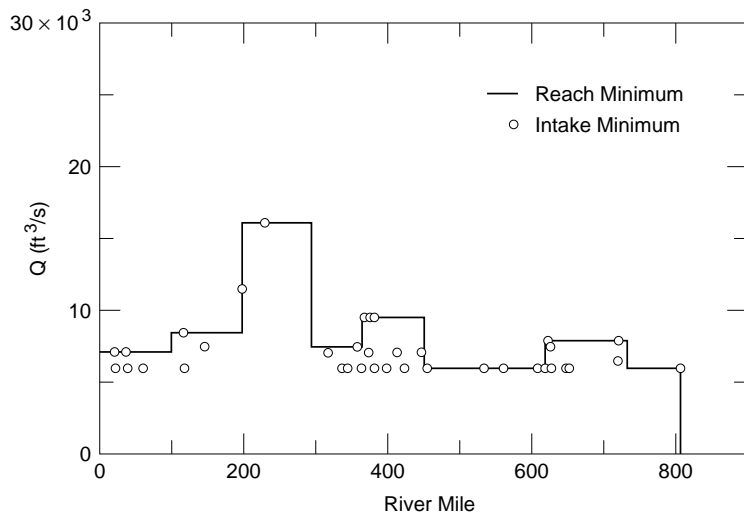
Figure 21. Minimum required discharges for water supply.
