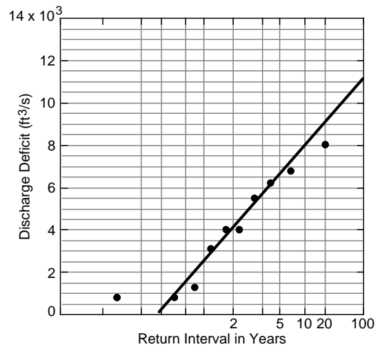
Figure 12. 1-15 January probabilities.
