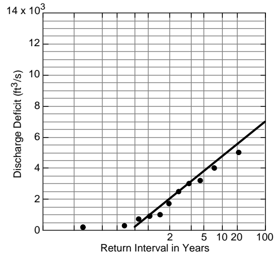
Figure 13. 16-31 January probabilities.
