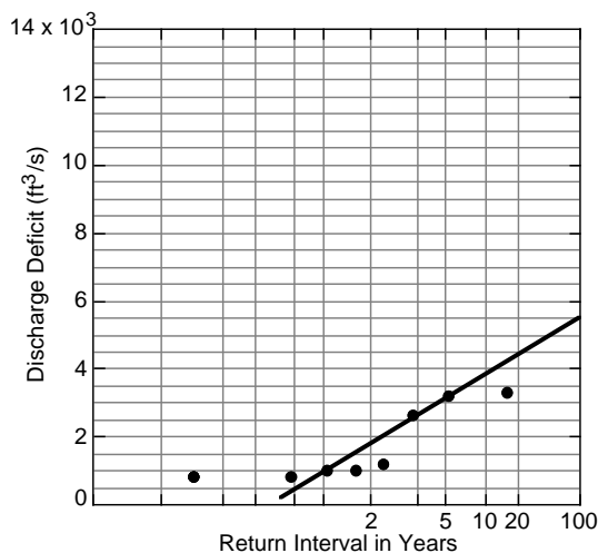
Figure 14. 1–15 February probabilities.
