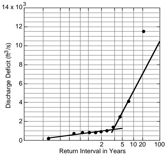
Figure 11. 16-31 December probabilities.
