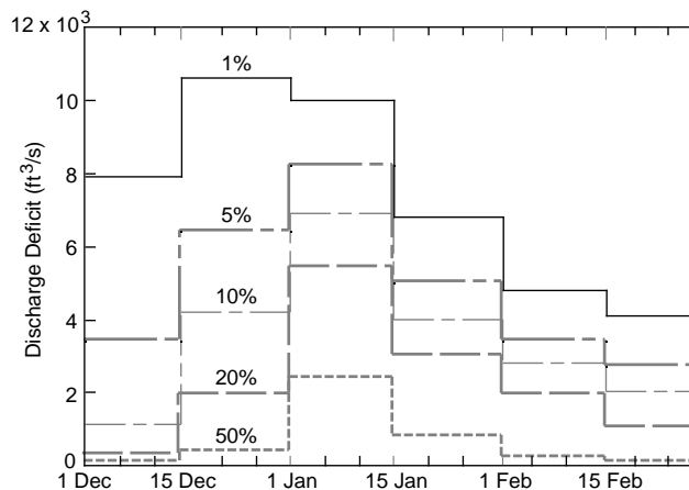
Figure 15. Probability of discharge deficit by time period.
