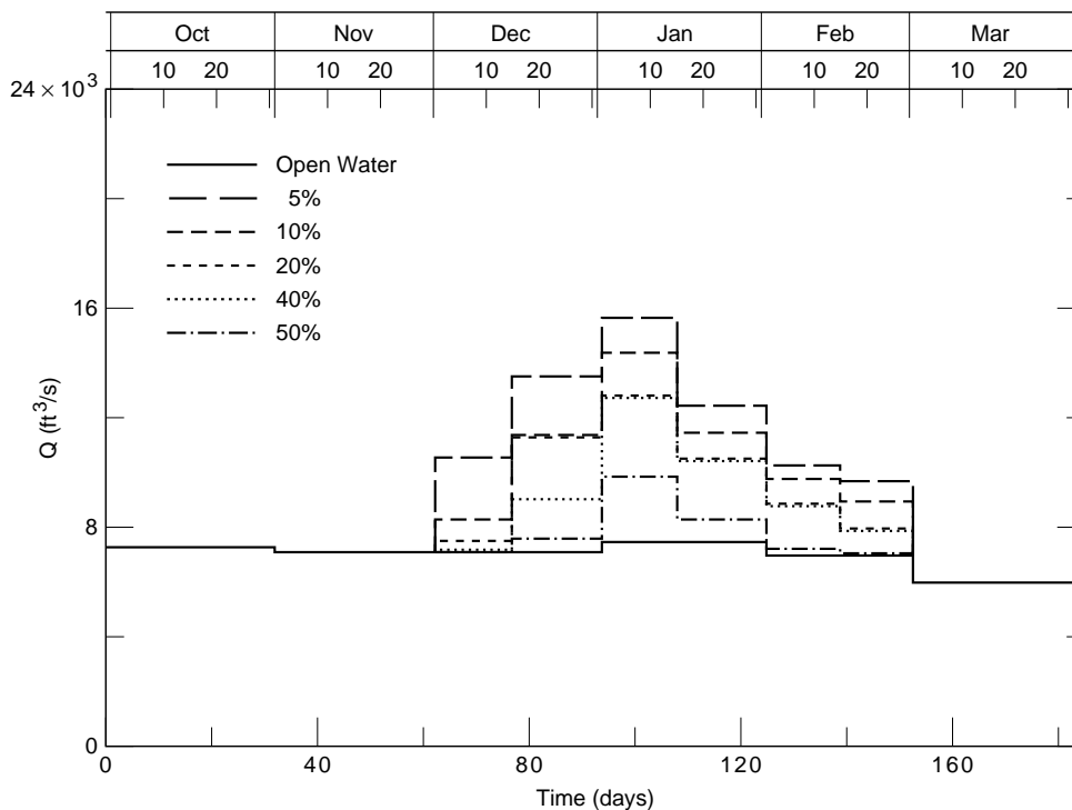
Figure 24. Minimum release from Gavins Point Dam (ice-impacted flows).
