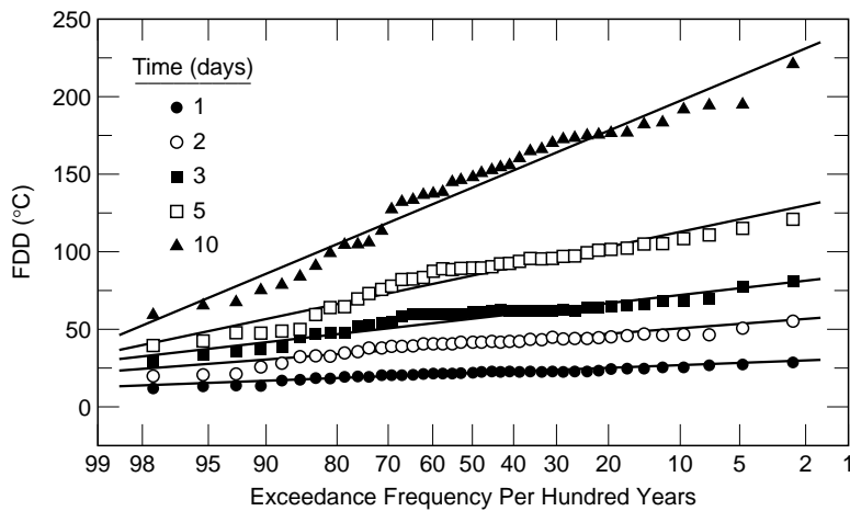
a. Freezing-degree-days exceedance frequency distribution.
