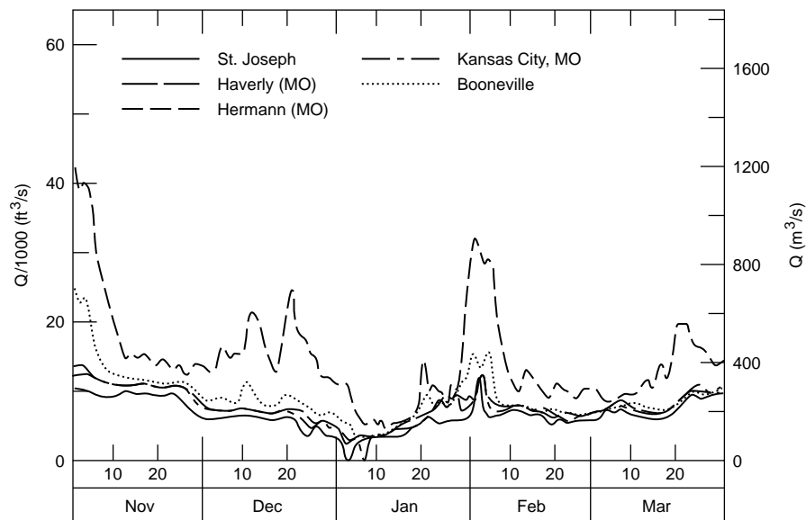
Figure 3 (cont'd). River discharge for winter of water year 1968.
