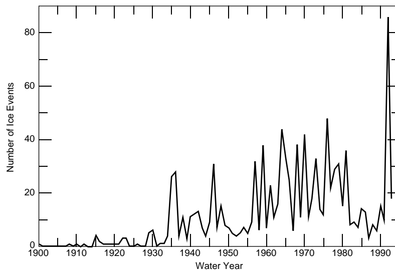
Figure 12. Number of ice events recorded annually for New Hampshire and Vermont (from White 1995).
