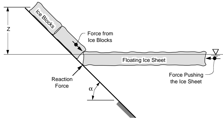
Figure 5. Sketch of forces acting during ice interaction with a sloping surface, where \alpha is slope angle from the horizontal and z is the height of pushed-up ice blocks.
