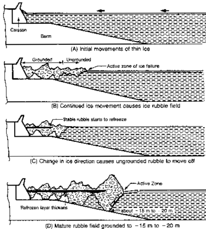
Figure 4. Typical ice action on caisson/berm structures (after Croasdale et al. 1988).
