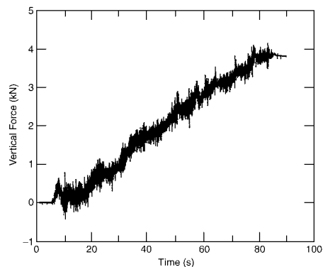
Figure 22. Typical plot of the vertical component of the force acting on the riprap.
