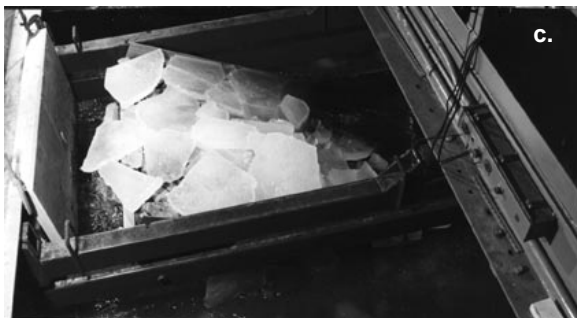
Figure 20. Sequence of ride-up and pileup events for test 20, in which the ice thickness was 53 mm (2.1 in.), and the bank slope was 27^\circ (1V:2H).
