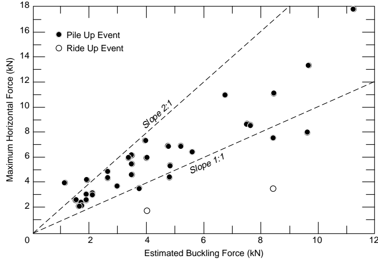
Figure 23. Plot of maximum force recorded during each test vs. b\rho_w g L^2 , where b is the width of ice sheet, \rho_w g is the specific weight of water, and L is the characteristic length of floating ice sheet.
