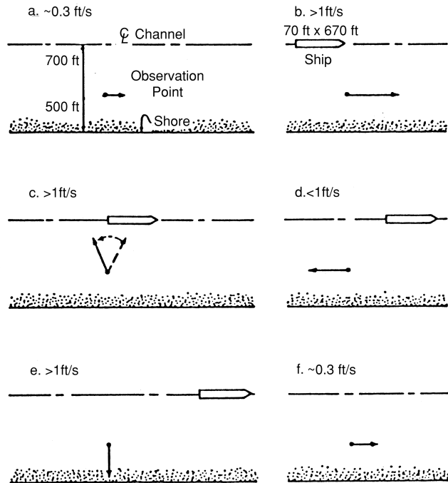
Figure 4. Ship-induced water movements. (From Wuebben et al. 1978a.)
