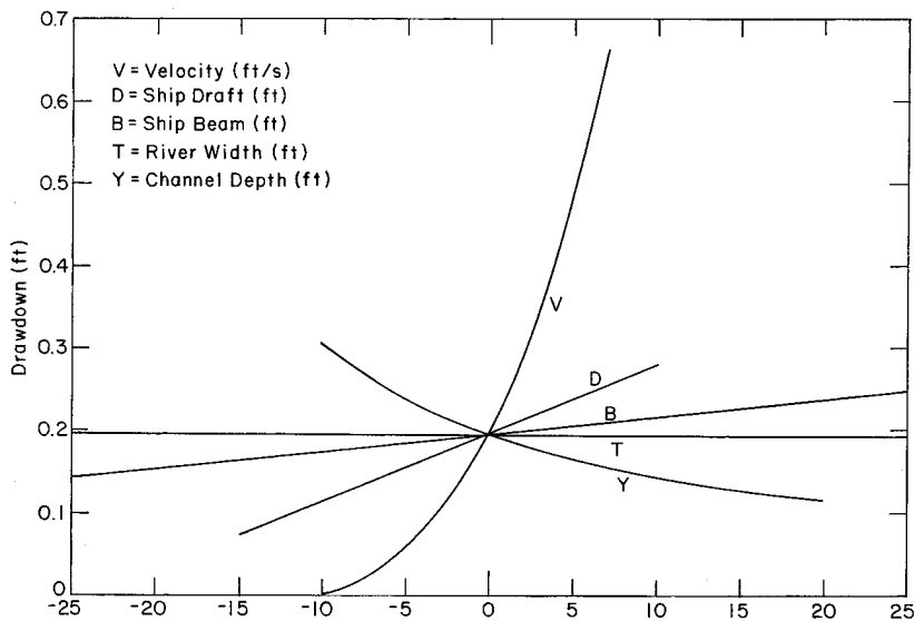
Figure 5. Effects on drawdown due to changes in variables from a basic case.
