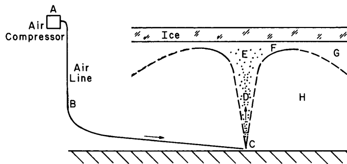
Figure 18. Schematic of a bubbler system.
