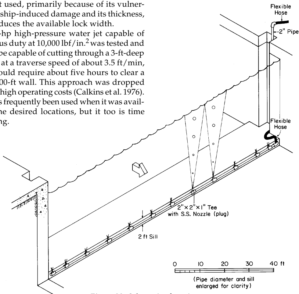
Figure 22. Schematic of an air screen.
