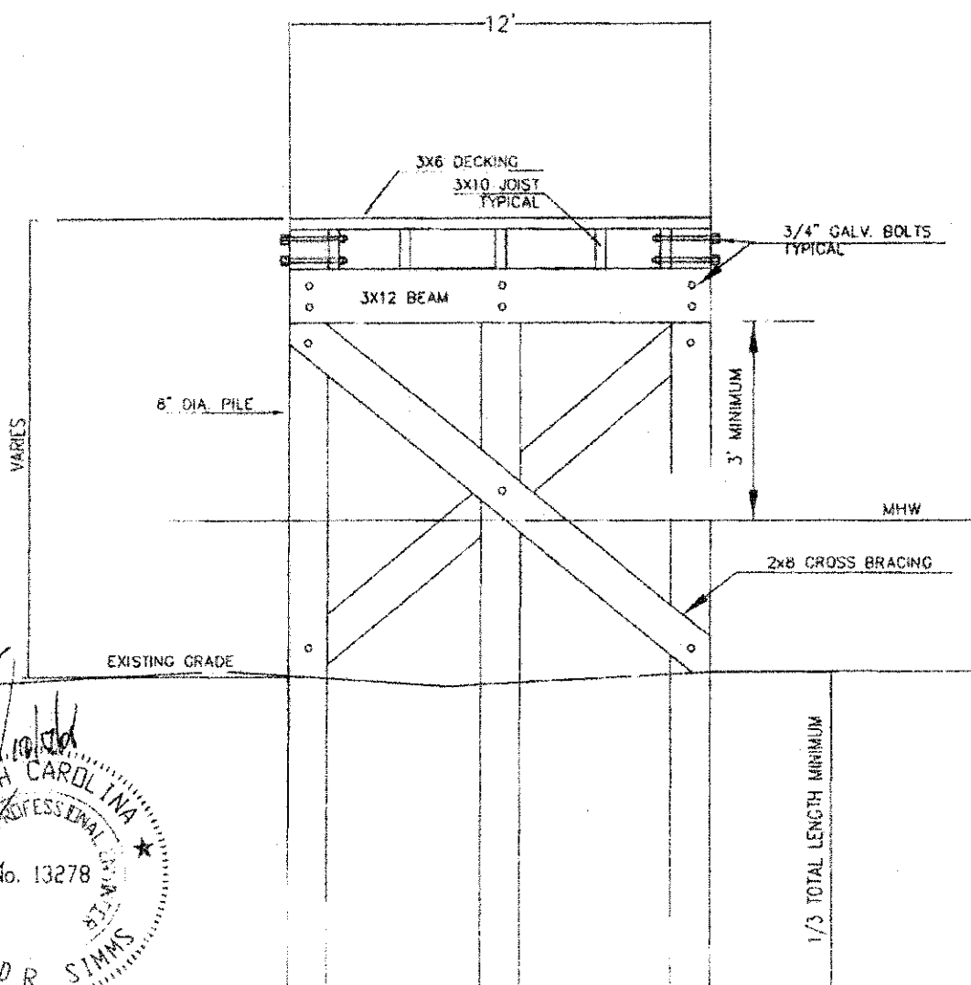
PIER HEAD CROSS SECTION
