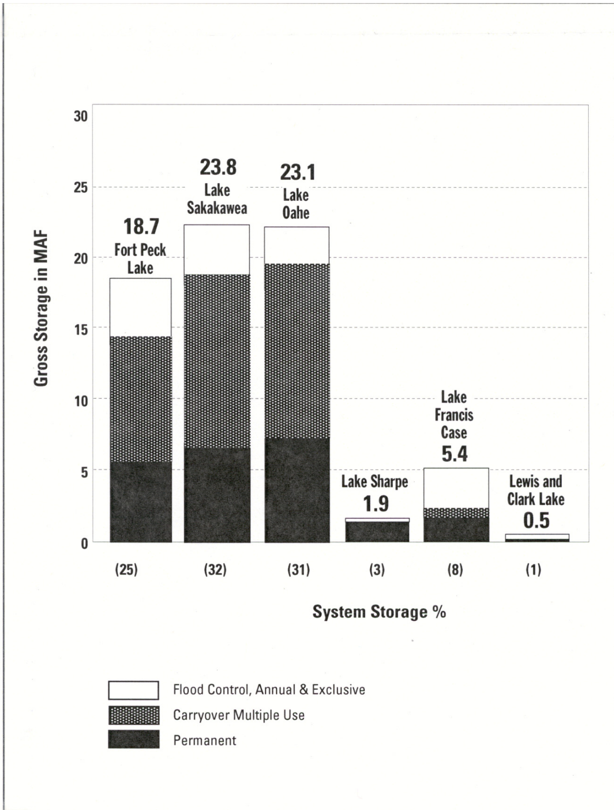
Figure 2.1-2. Missouri River Mainstem Reservoir System storage by mainstem lake (as established in the current Master Manual).
