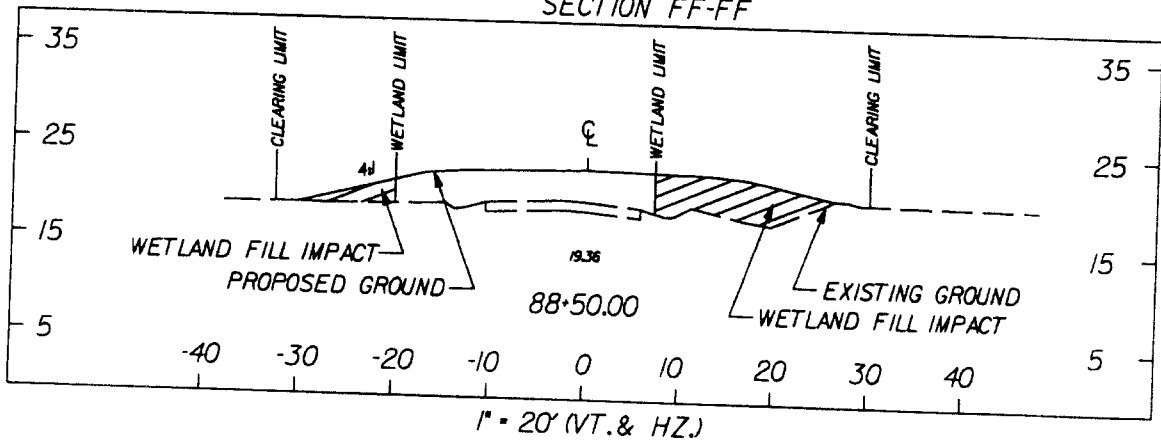
SECTION FF-FF
