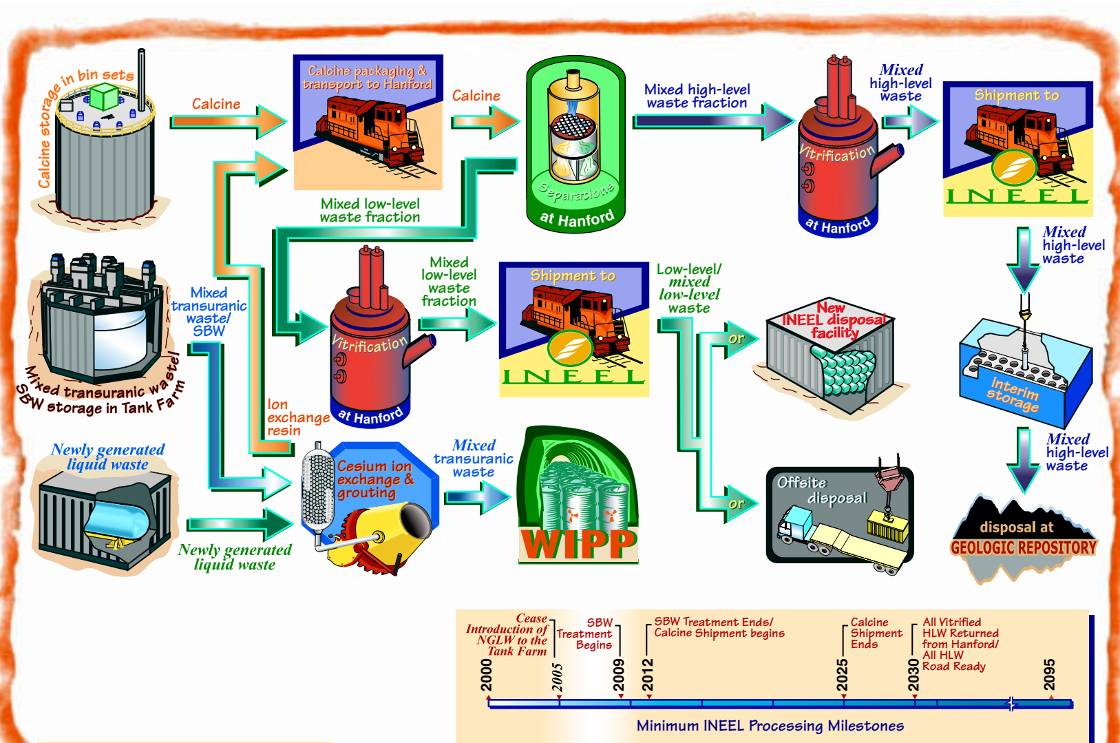
FIGURE S-11. Minimum INEEL Processing Alternative.
