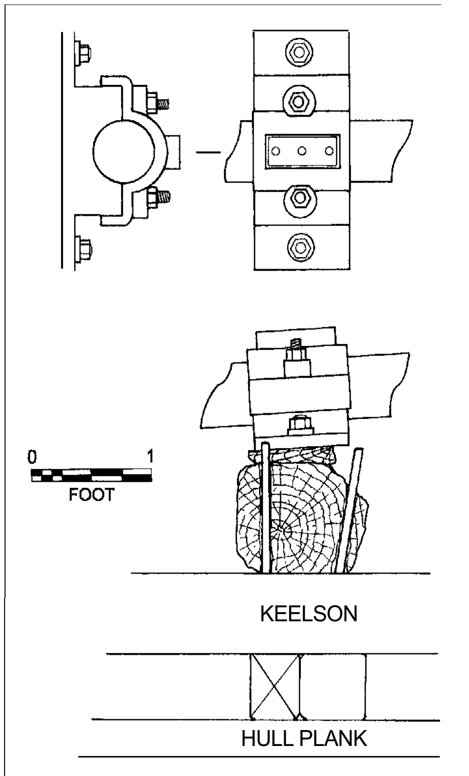
Figure 5.36. Plan, elevation and end view of forward propeller shaft bearing. Drawing by Jim Bradford.
