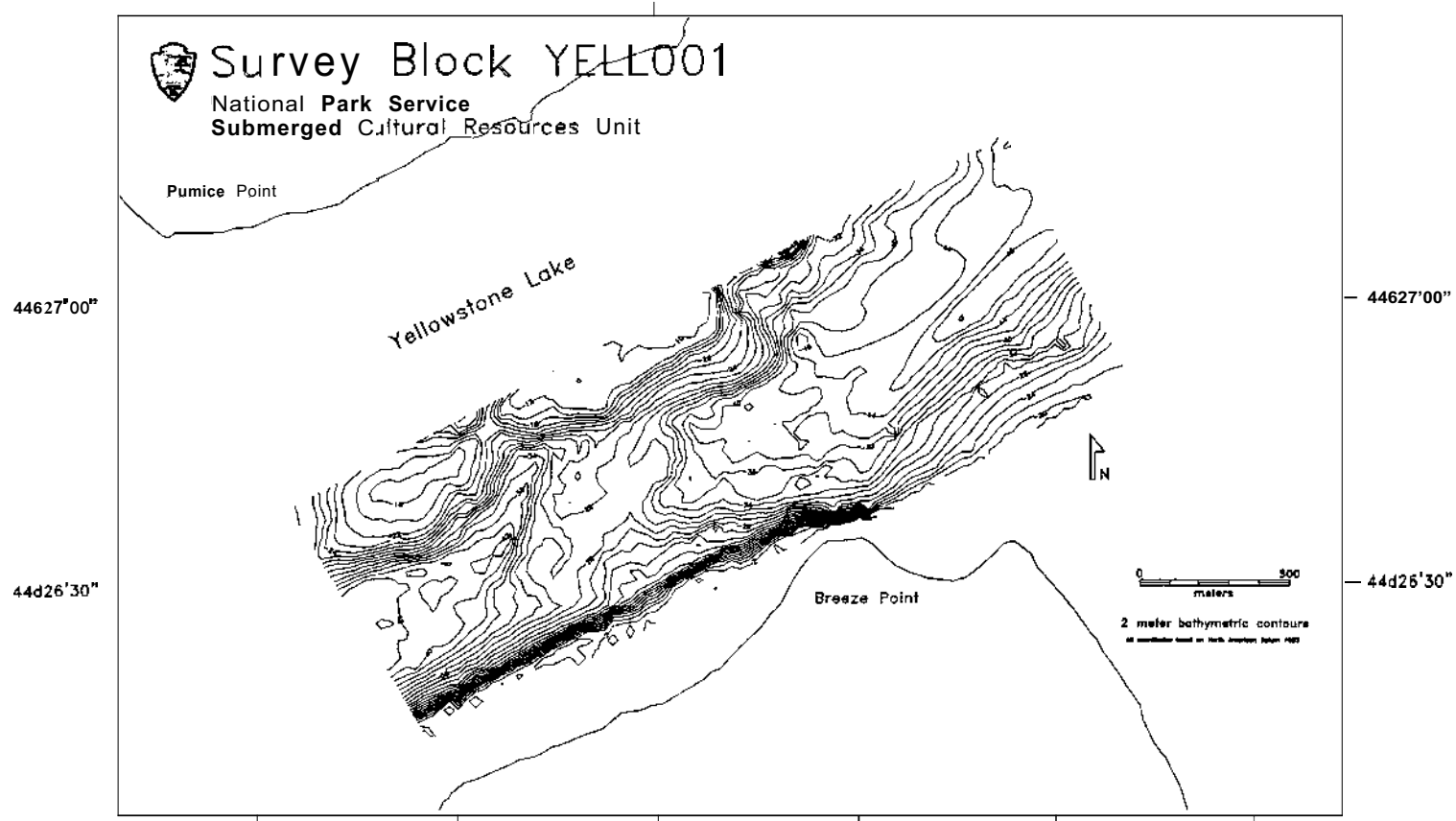
Figure 18. Two meter bathymetric contours, survey block YELL001.
