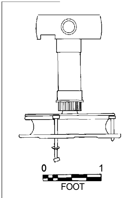
Figure 5.46. Scale drawing of E. C. Waters' capstan. Drawing by Matt Russell.
