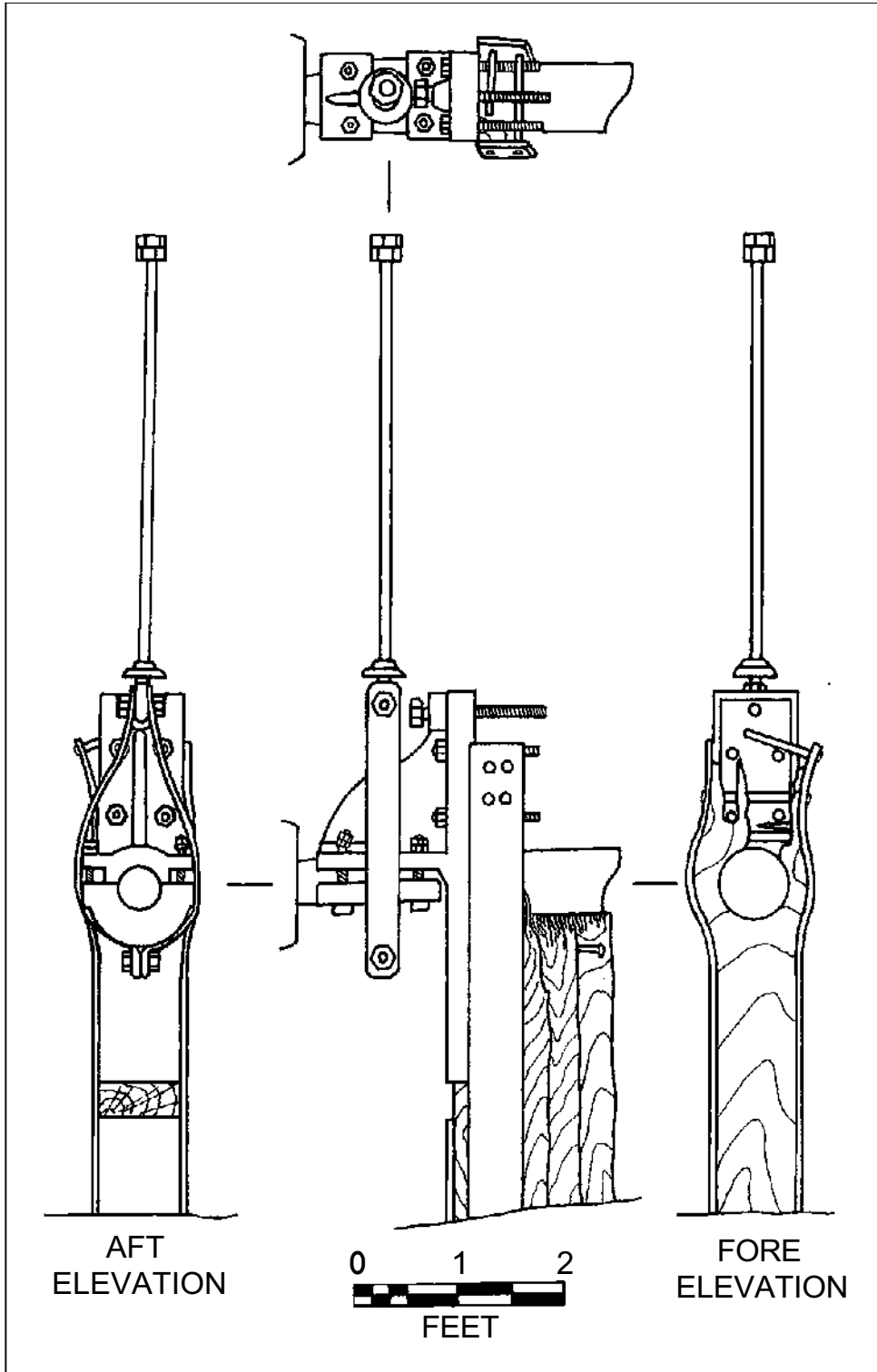
Figure 5.40. Plan, starboard elevation, fore and aft views of adjustable stem bearing assembly. Drawing by Jim Bradford.
