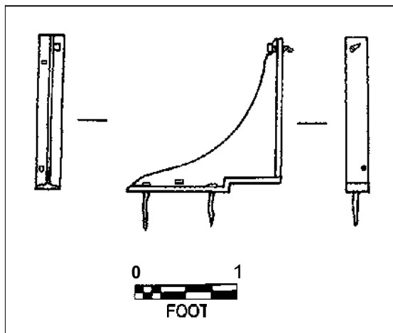
Figure 5.32. Side and end views of boiler saddle. Drawing by Jim Bradford.
