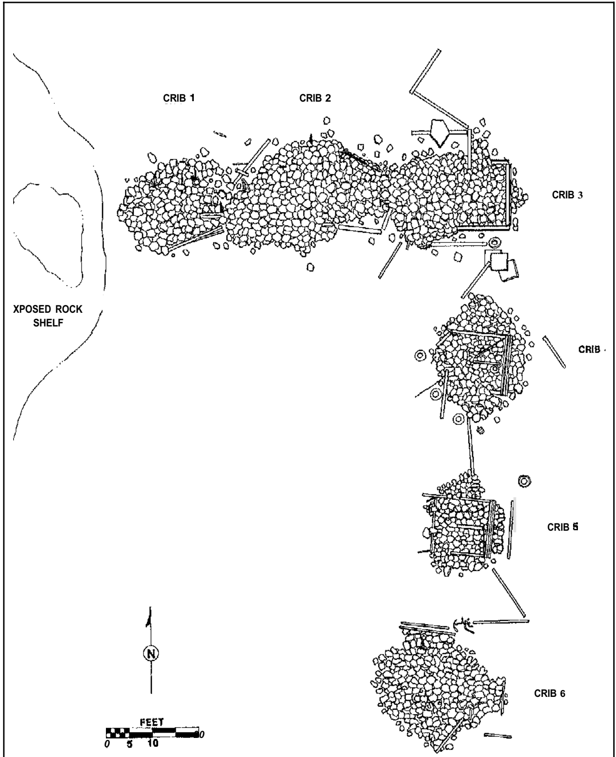
Figure 5.7. Plan view site map of the West Thumb dock cribs. Drawing by Jim Bradford and Matt Russell.
