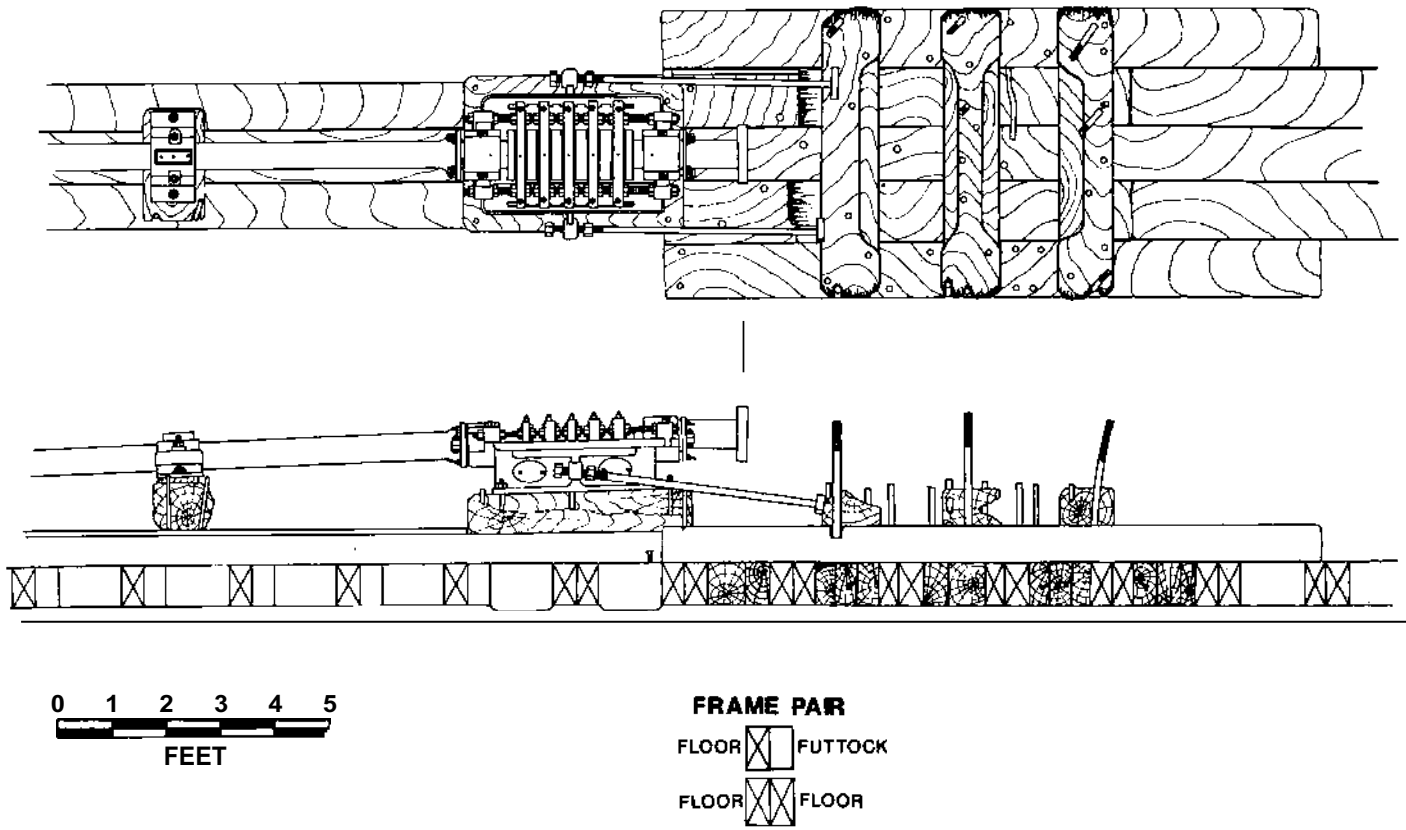
Figure 5.31. Plan and elevation of engine bed and thrust bearing showing additional frames to support engine weight. Drawing by Jim Bradford.
