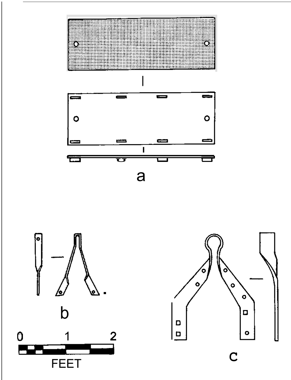
Figure 5.51. Plan and profile views of flat metal plate (a), "V"-shaped brace (b) and boat davit brace (c). Drawing by Jim Bradford.
