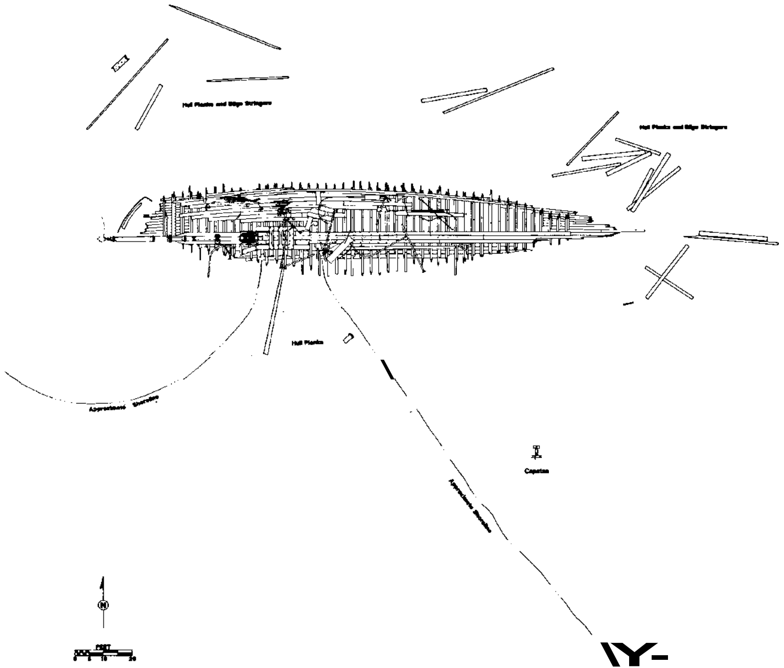
Figure 5.27. Plan view of E. C. Waters ' site (48YE13). Drawing by Jim Bradford and Matt Russell.
