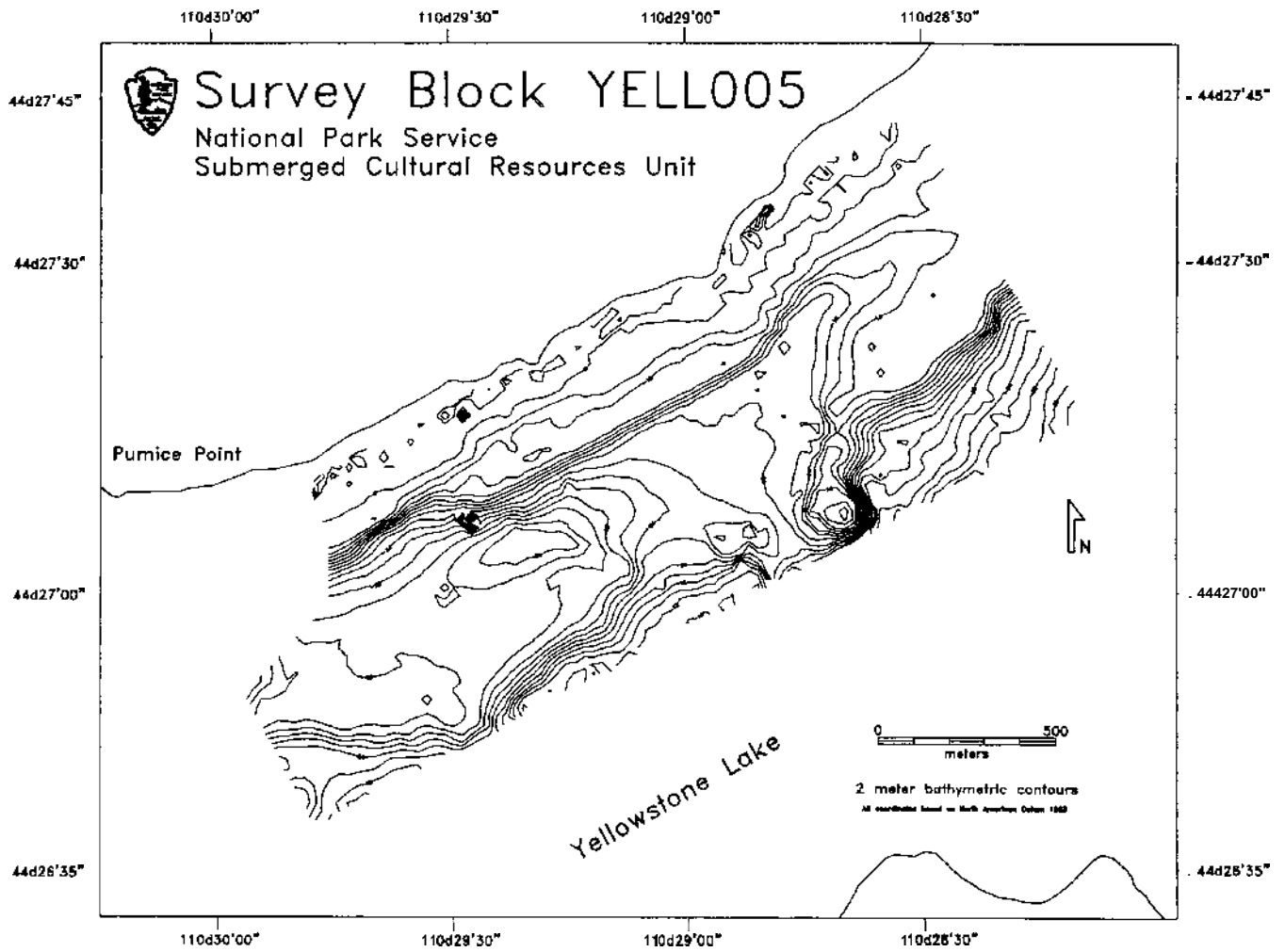
Figure 19. Two meter bathymetric contours, survey block YELL005.
