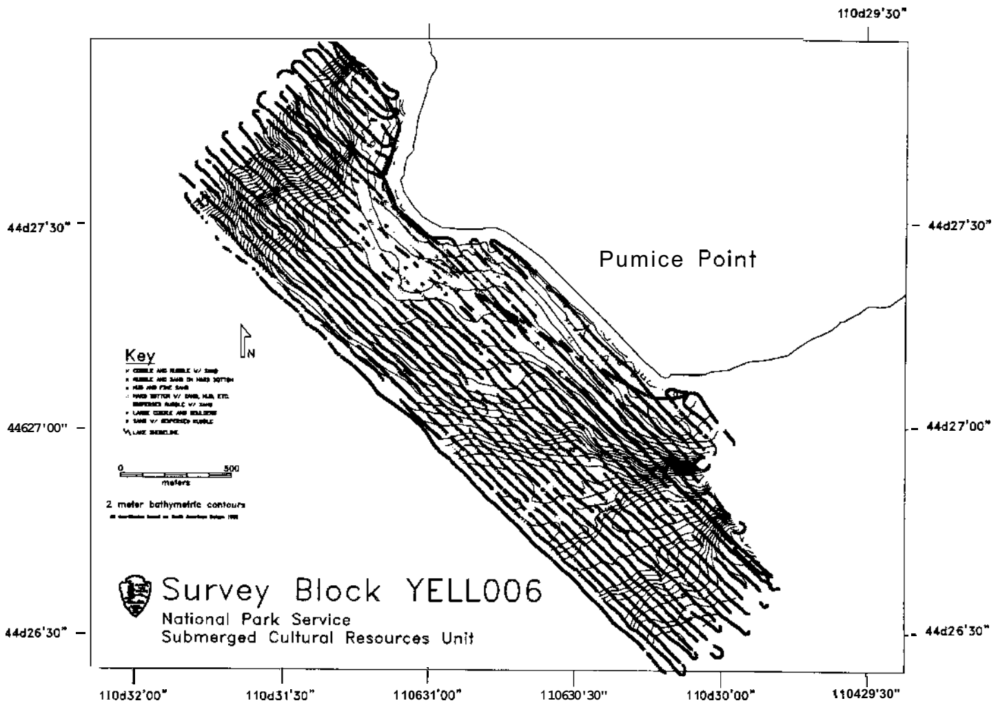
Figure 10. Raw RoxAnn data, survey block YELL006.
