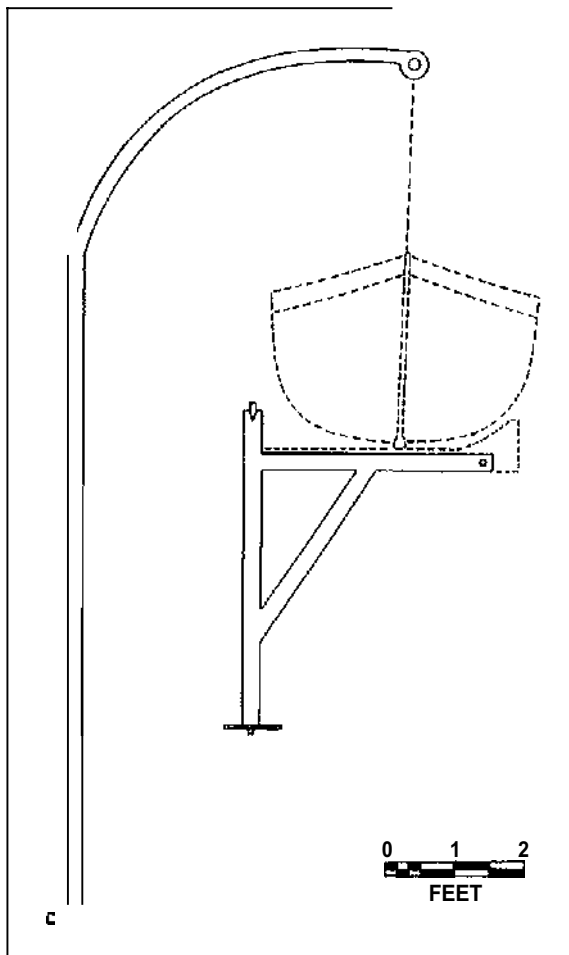
Figure 5.48. Scale drawing of life boat davit and support bracket showing their relative positions in securing a life boat. Drawing by Jim Bradford.
