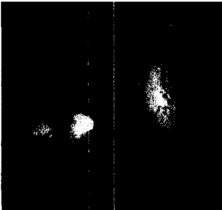
Figure 15. Sonograph of unusual geological feature on lake floor. Most likely this is a hot water vent surrounded by mineral deposition.
