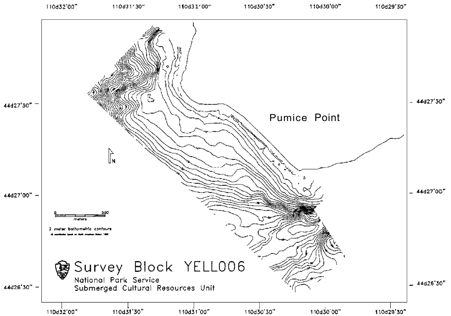
Figure 20. Two meter bathymetric contours, survey block YELL006.
