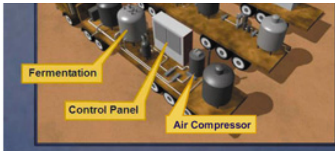
Interior graphic from Secretary Powell's speech showing original three-trailer design.
