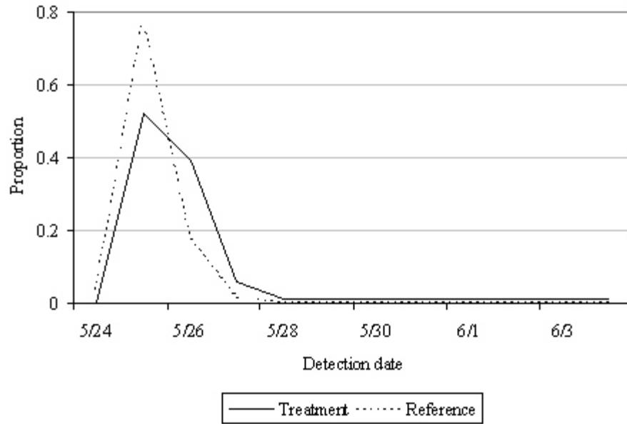
Appendix Figure D11. Passage distribution at McNary Dam for PIT-tagged hatchery yearling chinook salmon released during nighttime operations at Ice Harbor Dam on 23 May 2002.
