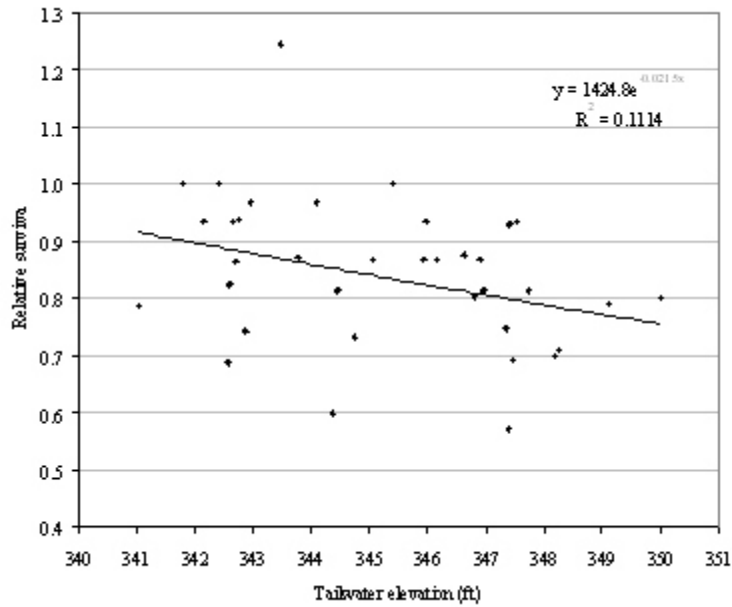
Appendix Figure C9. Estimated relative spillway survival by tailwater elevation (presented as feet above mean sea level) at time of release for radio-tagged hatchery yearling chinook salmon released at Ice Harbor Dam, 2002 ( P = 0.047 ).
