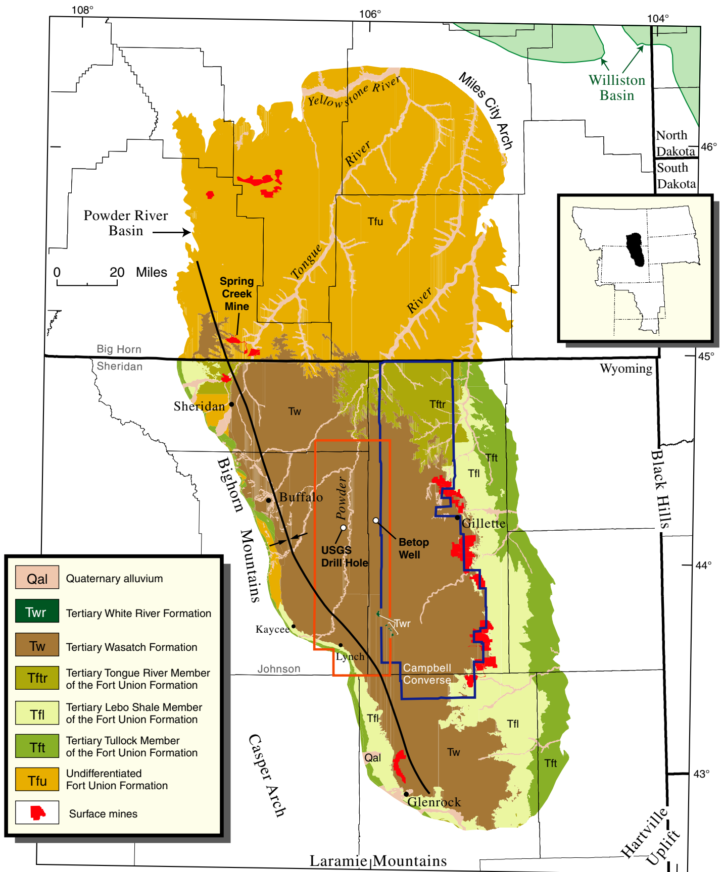
Figure PS-1. Generalized geologic map showing the extent of the Powder River Basin in Wyoming and Montana (adapted from Raines and Johnson, 1996; Green and Drouillard, 1994). Also shown are county boundaries, geological structures, mines, and cities. Coal-bed methane may be targeted for exploration in the eastern (shallow) and southwestern (deep) parts of the basin (Bureau of Land Management, 1999).
