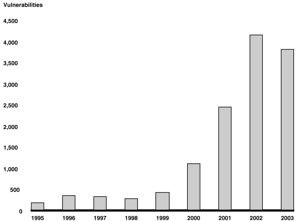
Figure 1: Security Vulnerabilities, 1995–2003
