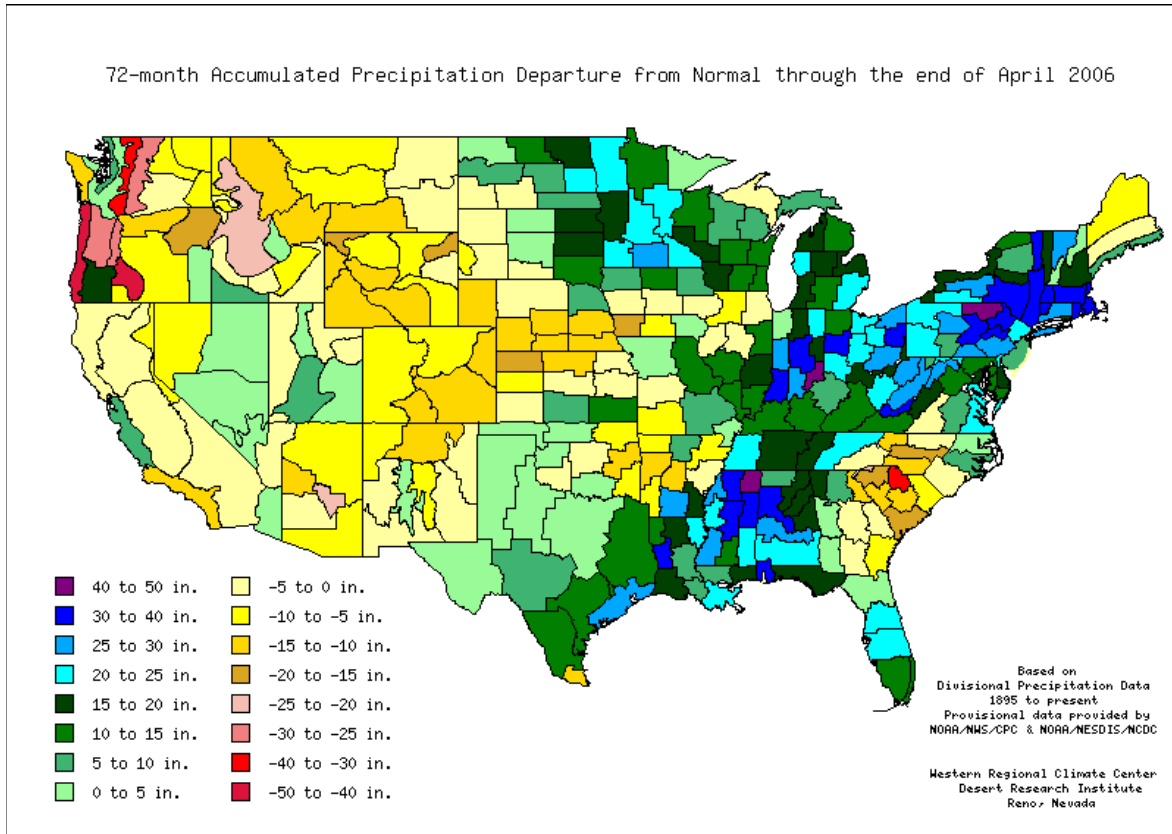
Figure 1 – 72 month Precipitation Departure From Normal
