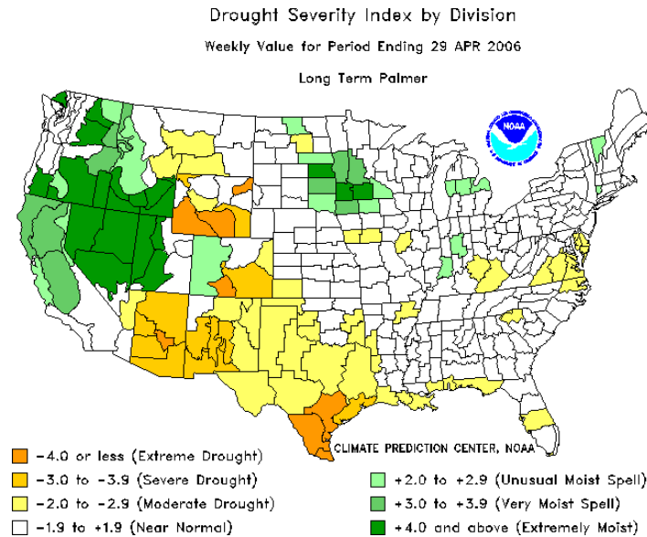
Figure 5 – Long-Term Palmer Drought Indicator Ending 29 APR 2006
