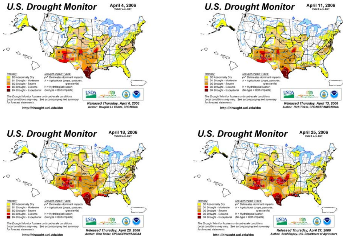
Figure 6 – U.S. Drought Monitor – April 4, 2006 through April 25, 2006 http://www.drought.unl.edu/dm/monitor.html
