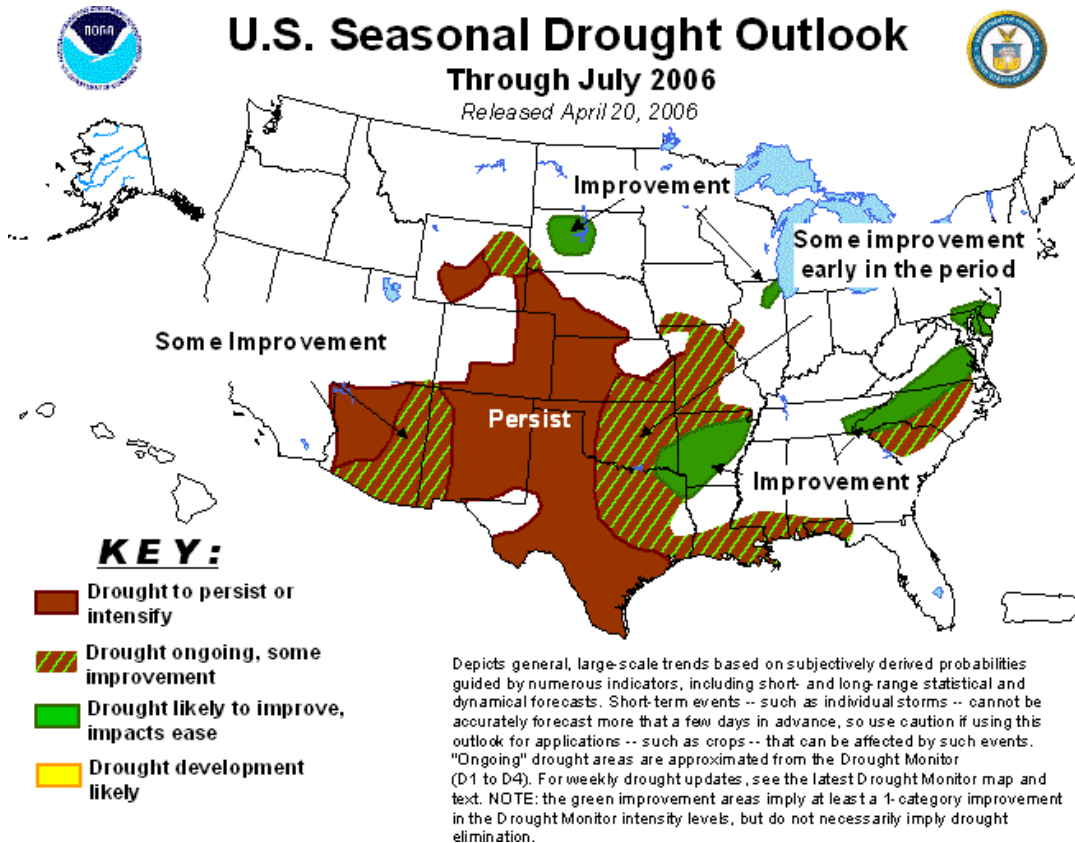
Figure 7 – Three-Month Seasonal Drought Outlook through July 2006
