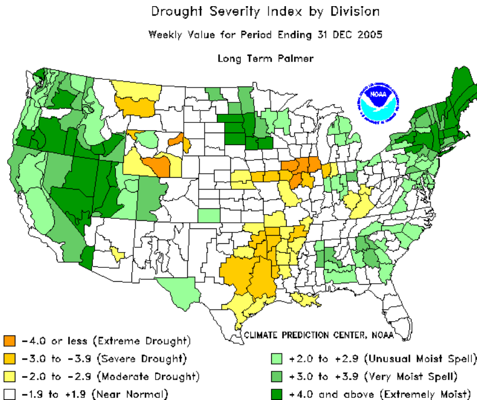
Figure 5 – Long-Term Palmer Drought Indicator Ending 31 DEC 2005
