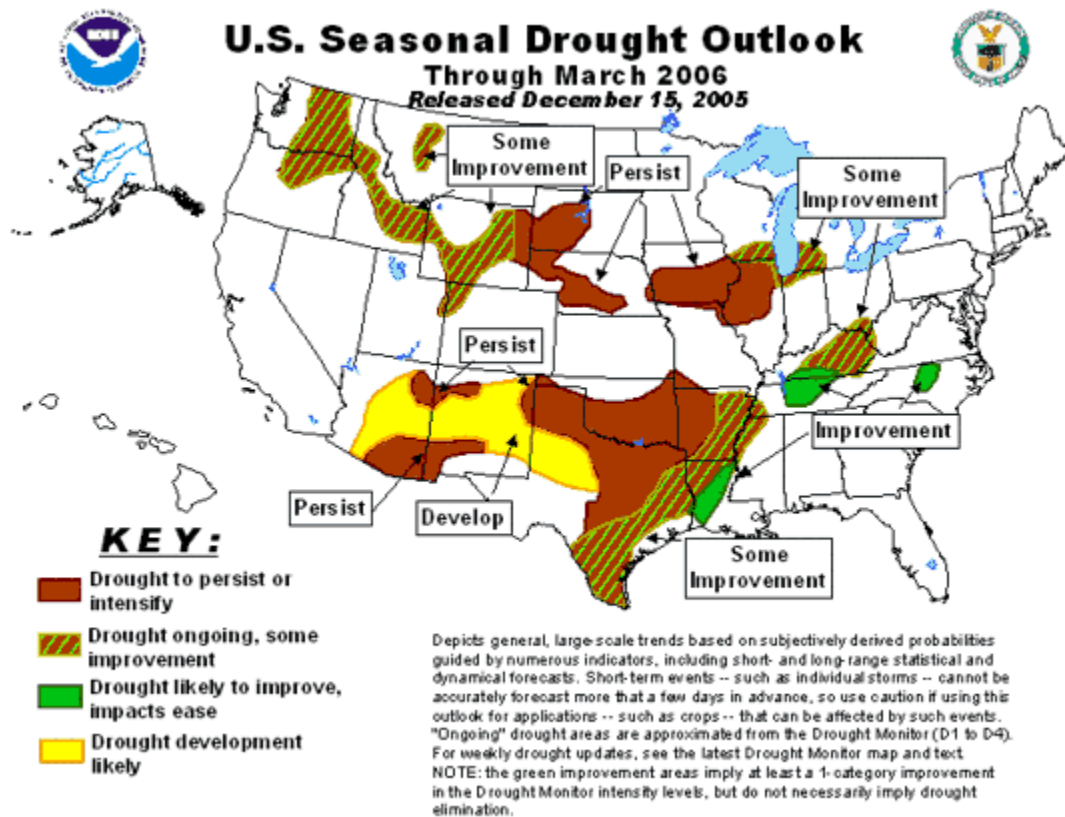
Figure 7 – Three-Month Seasonal Drought Outlook through March 2006
