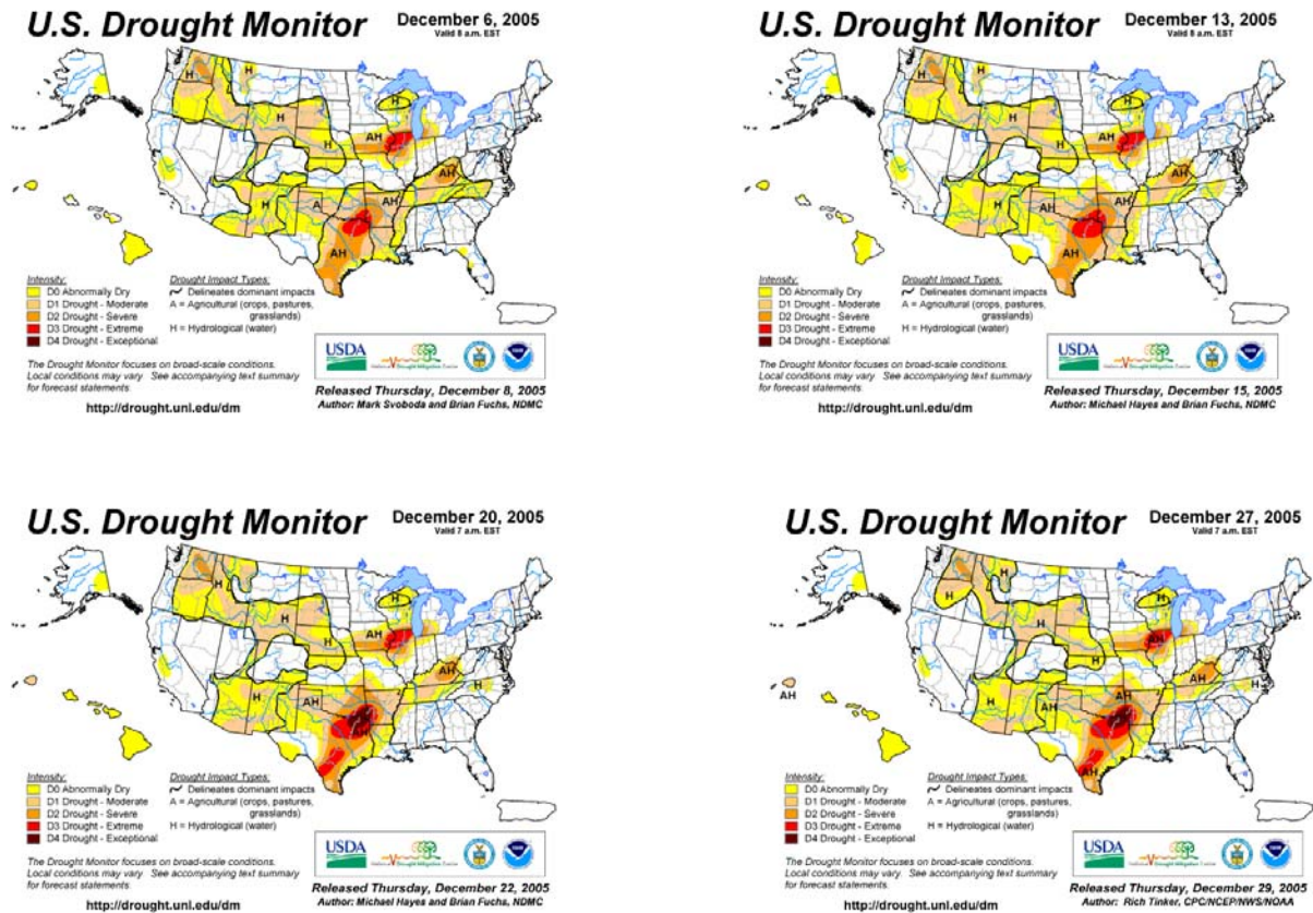
Figure 6 – U.S. Drought Monitor – December 6, 2005 through December 27, 2005 http://drought.unl.edu/dm/monitor.html
