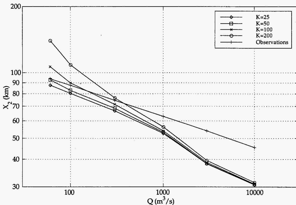
FIG. 12. Steady-state X_2 - Q relations computed numerically using different values of K_B and keeping \gamma constant compared with observed values.
