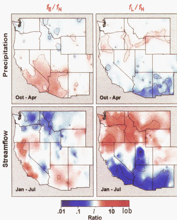
FIG. 8. (a) and (b) Precipitation and (c) and (d) stream flow ratio of frequencies of daily values exceeding 90th percentile, (a) and (c) f_E/f_N , SOI-/neutral and (b) and (d) f_L/f_N , SOI+/neutral. Red denotes ratios >1.0, blue denotes ratios <1.0. Dashed lines denote regions where frequency ratio exceeds 90% of confidence level via Monte Carlo trials.
