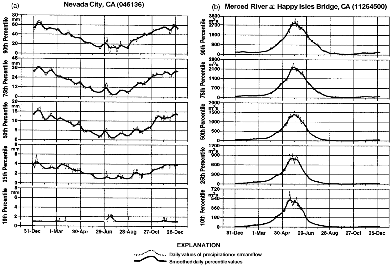
FIG. 4. Smoothed percentiles of (a) daily precipitation, Nevada City, CA, and (b) nearby daily stream flow on the Merced River at Happy Isles Bridge, CA, based on 1948–95 data.
