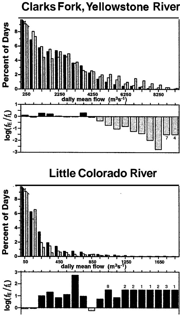
FIG. 6. Frequency distribution of daily mean stream flow for SOI- and SOI+ for (a) Clark's Fork River of the Yellowstone River, near Belfry, MT, and (c) for the Little Colorado River above Lyman Lake, AZ. Based on Jan-Jul, 1948-95, the lowest category of flow in (a) and (c) is truncated in order to display higher flow categories. (b) and (c) Graph of each pair shows ratio of frequency, SOI-/SOI+; when ratio is infinite (one category has no occurrences), the value plotted is 1.5, and the number of occurrences in the other category is labeled at top of bar.
