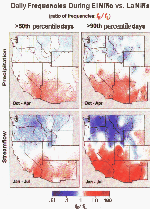
FIG. 7. (a) and (h) Precipitation and (c) and (d) stream flow f_E/f_L ratio of frequencies (SOI–/SOI+) of daily values exceeding (a) and (c) 50th percentile and (b) and (d) 90th percentile. Precipitation during Oct–Apr, stream flow during Jan–Jul, 1948–95. Red denotes ratios >1.0 (SOI– cases have more frequent events than SOI+ cases), blue denotes ratios <1.0 (SOI+ cases have less frequent events than SOI– cases). Dashed lines denote regions where frequency ratio exceeds 90% confidence levels via Monte Carlo trials.
