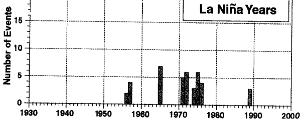
FIG. 2. Number of days with precipitation exceeding daily 90th percentile in SOI- (El Niño) and SOI+ (La Niña) years, San Diego, CA, Oct-Apr, 1931-95. Approximately six P90 events per year are expected, on average, over the entire record.
