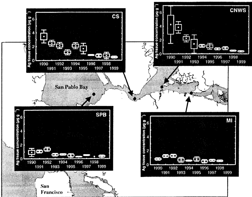
Figure 4. Annual mean silver concentrations ( \mu\text{g g}^{-1} dry weight) in the tissues of Potamocorbula amurensis from 1990 to 1999 at each site. The boxes represent 1 standard error and the whiskers represent 1.96 standard error.
