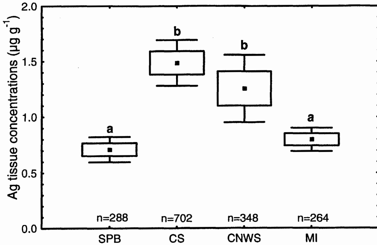
Figure 3. Grand mean silver tissue concentrations in Potamocorbula amurensis at each site. The points represent the grand means of all data from 1990 to 1999 in µg g -1 dry weight, with number of samples (n) per mean shown at the bottom of the graph. The boxes represent 1 standard error and the whiskers represent 1.96 standard error. The letters a and b designate significant differences among means ( p \leq 0.05 ).
