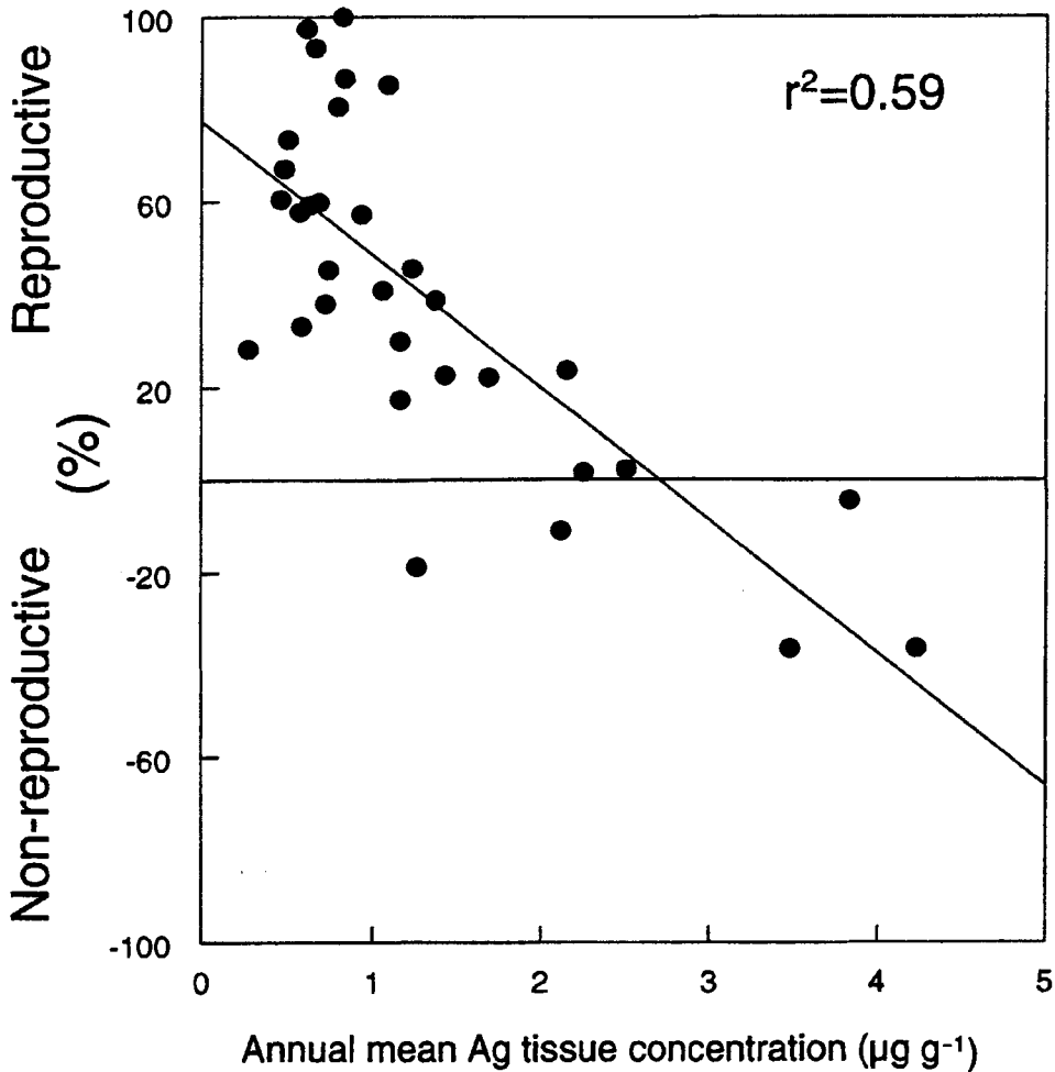
Figure 10. Correlation between the annual proportions (%) of reproductive clams ( Potamocorbula amurensis ) with the annual mean silver concentrations ( \mu\text{g g}^{-1} dry weight) at the four sites. Y-axis represents the central tendency of the reproduction data: the proportion of clams that were reproductively active (% active + % ripe + % spawned) minus the proportion of clams that were non-reproductively active (% inactive + % spent) collected each month.
