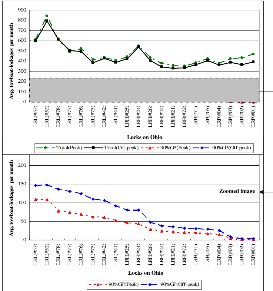
Figure 10. Ohio Towboat Lockages during the UMR Peak and Off-peak (2000-2004)
