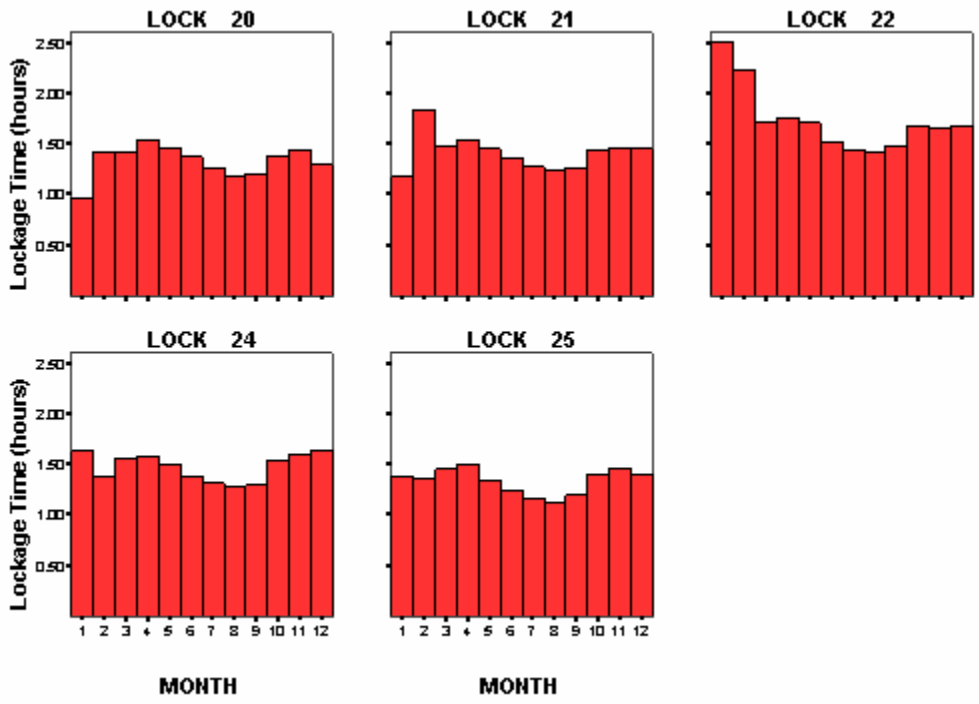
Figure 8. Mean Lockage Times for UMR Locks 20 through 25 by Month, 2000 through 2003
