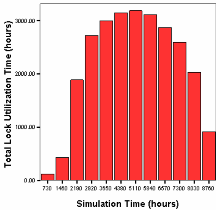
Figure 14. Mean Simulated Values of the Total Aggregated Lock Utilization Times for UMR Locks 20 through 25 for Twelve Equal Periods
