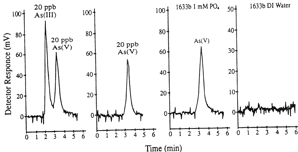
FIGURE 7. HPLC-HGAAS chromatograms of a mixed As(III) + As(V) standard, a single-ion As(V) standard, and the DI water and 1 mM PO 4 extracts of coal fly ash (NBS-1633b).
