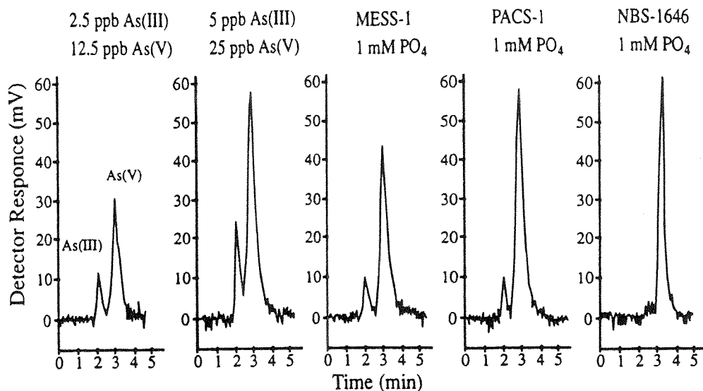
FIGURE 5. HPLC-HGAAS chromatograms using the OmniPac PAX-500 column showing two As(III) + As(V) mixed standard solutions and the 1 mM PO 4 extracts of MESS-1, PACS-1, and NBS-1646 estuarine sediments. Standards and extracts were diluted with 1 mM PO 4 .
