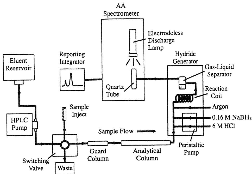
FIGURE 1. Schematic diagram of the high-performance liquid chromatography-hydride generation atomic absorption spectrophotometry (HPLC-HGAAS) system.
