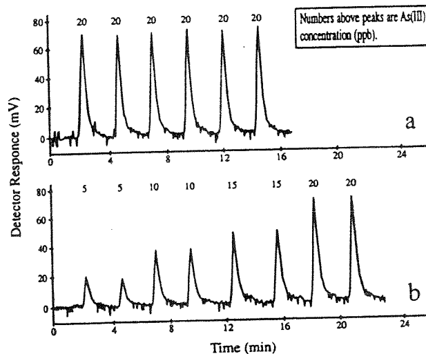
FIGURE 2. HPLC-HGAAS chromatograms using the OmniPac PAX-500 column showing multiple injections of 20 ppb As(III) standard solution (a) and duplicate injections of 5, 10, 15, and 20 ppb As(III) standard solutions (b). See Table 1 for run parameters.
