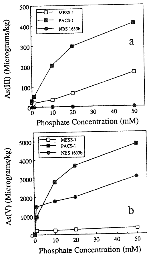
FIGURE 8. Effects of PO 4 extract solution concentration on extractable As(III) (a) and As(V) (b) from estuarine sediments (MESS-1 and PACS-1) and coal fly ash (NBS-1633b).
