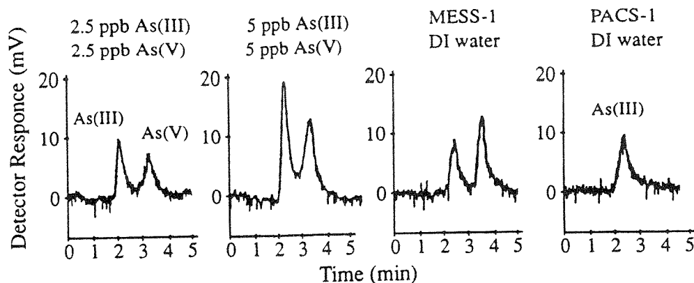
FIGURE 4. HPLC-HGAAS chromatograms using the OmniPac PAX-500 column of two As(III) + As(V) mixed ion standard solutions and the DI water extracts of MESS-1 and PACS-1 estuarine sediment. The DI water extracts were spiked with 100 mM \text{PO}_4 solution to make 1 mM \text{PO}_4 final concentration in the extracts. For these injections, the 3393A integrator attenuation (ATT 2 \wedge ) was set at 6.
