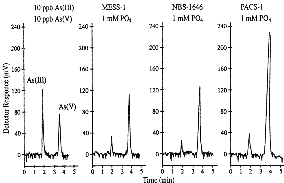
FIGURE 6. HPLC-HGAAS chromatograms using the IonPac AS11 column showing one As(III) + As(V) mixed standard solution and the 1 mM PO 4 extracts of MESS-1, PACS-1, and NBS-1646 estuarine sediments. Retention times for As(III) and As(V) were 1.9 and 3.8 min, respectively. Standards and extracts were diluted with 1 mM PO 4 .
