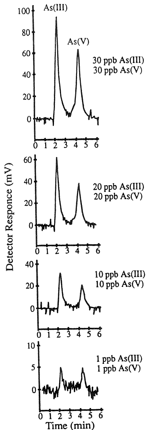
FIGURE 3. Representative HPLC-HGAAS chromatograms using the OmniPac PAX-500 column showing injections of As(III) + As(V) mixed standard solutions. Retention times for As(III) and As(V) were 2.2 and 4.2 min, respectively. All run parameters are those given in Table 1, except for 1 ppb As(III) + 1 ppb As(V) where the 3393A integrator attenuation (ATT 2 \wedge ) was set at 5.
