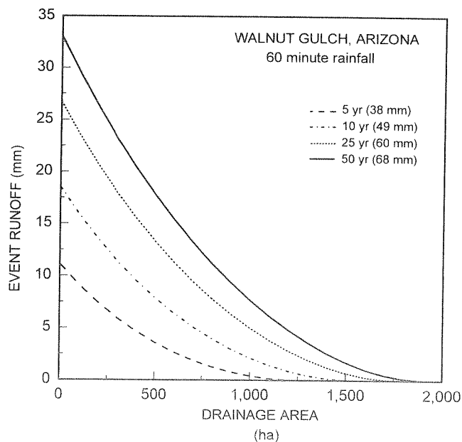
Figure 3—Variation in runoff depth (mm) with drainage area for various return period 60-min rainfall for the Walnut Gulch watershed.
