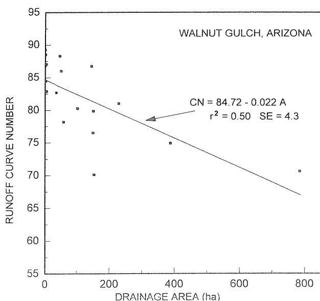
Figure 2—Plot of data-defined Curve Numbers with drainage area. The fitted line is CN = 84.72 - 0.022 \times A , where A = \text{ha} , r^2 = 0.50 , Std. Err. = 4.3 CN.
