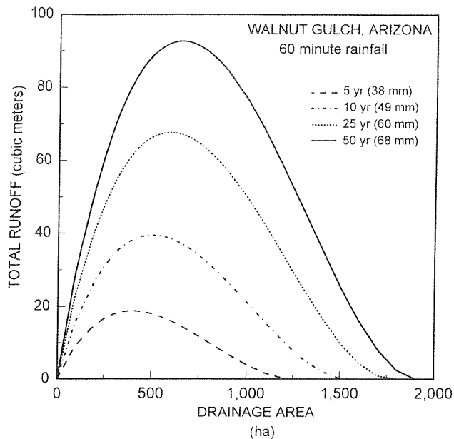
Figure 4—Runoff volume ( \text{m}^3 ) of drainage areas for various return period 60-min rainfall for the Walnut Gulch watershed.
