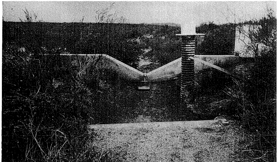
Fig. 5. Sediment trap above Walnut Gulch runoff-measuring station 104 (looking downstream).
