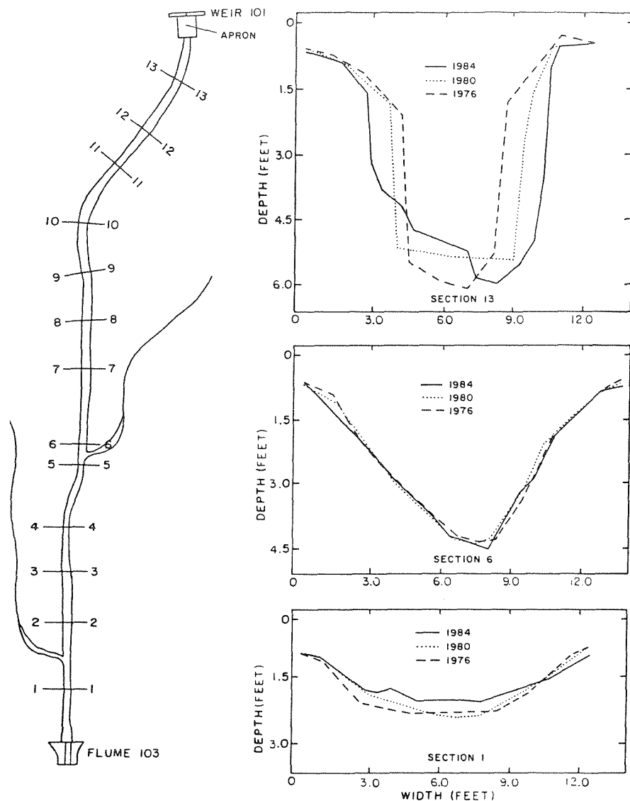
Fig. 7. Location of cross sections and selected cross sections above flume 103.
