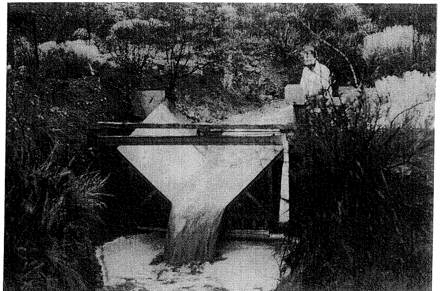
Fig. 6. Flume and total load sampler at runoff measuring station 103, Walnut Gulch.
