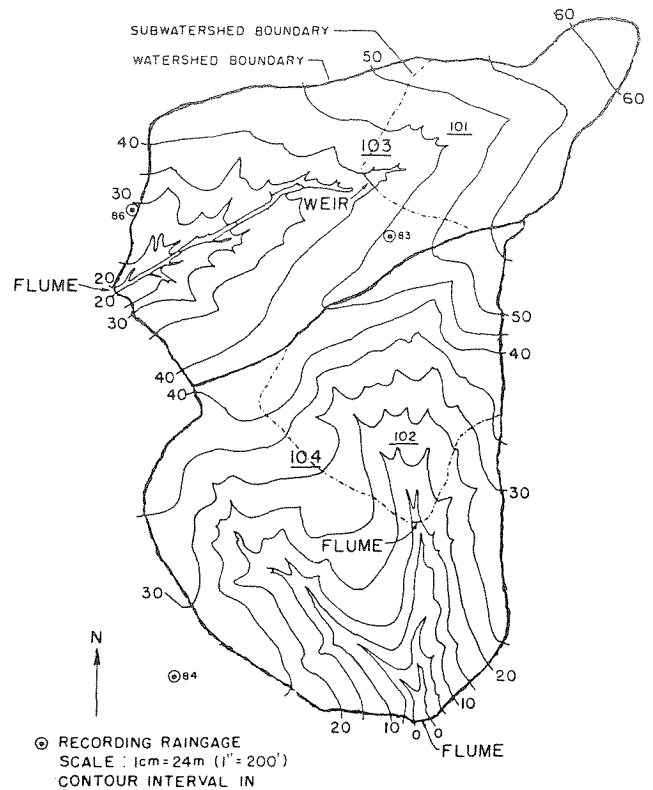
Fig. 2. Subwatersheds 101, 102, 103, and 104, Walnut Gulch.
