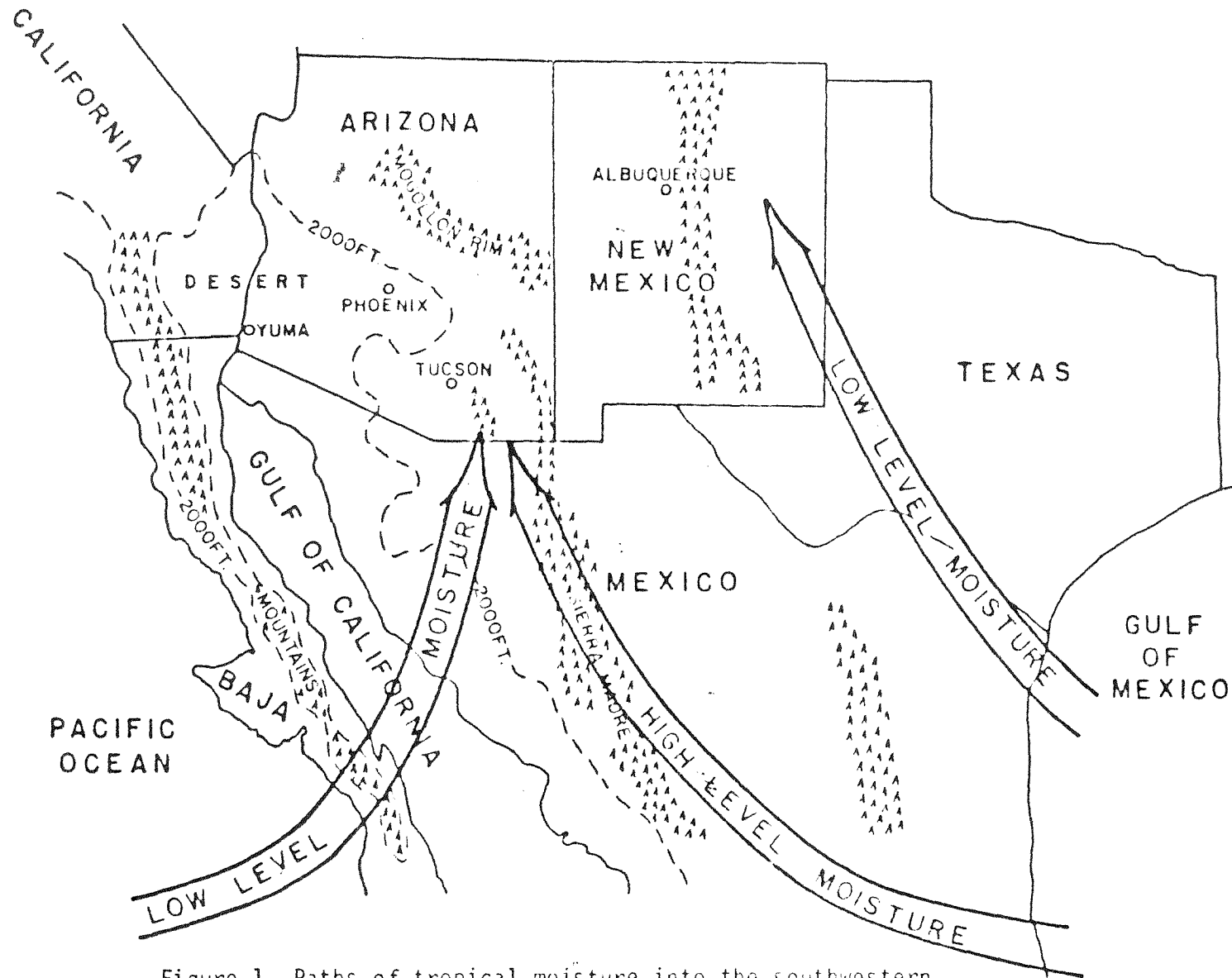
Figure 1. Paths of tropical moisture into the southwestern United States and northern Mexico.
