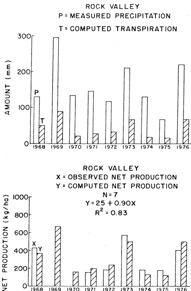
Fig. 5. Annual values of precipitation, computed transpiration, and net production of perennial vegetation at Rock Valley, Nevada, 1968-1976.
