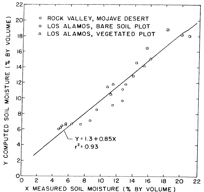
Fig. 4. Relationship between measured and computed monthly soil moisture for Rock Valley, Nevada and Los Alamos, New Mexico.
