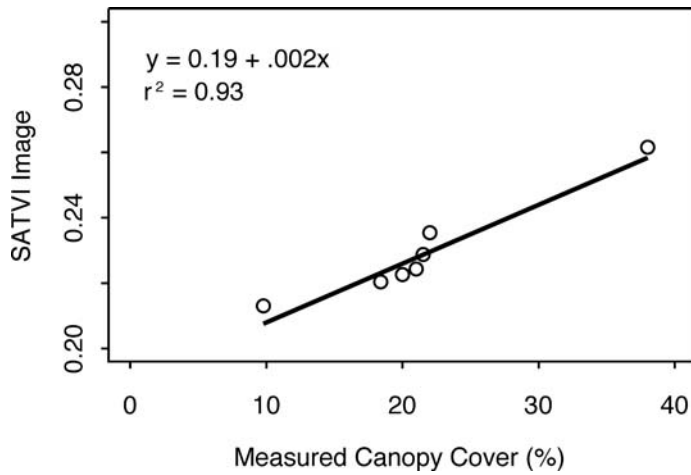
Figure 5. Soil Adjusted Total Vegetation Index (SATVI) compared to measured cover for the Spring 2004 image in southeastern Arizona.
