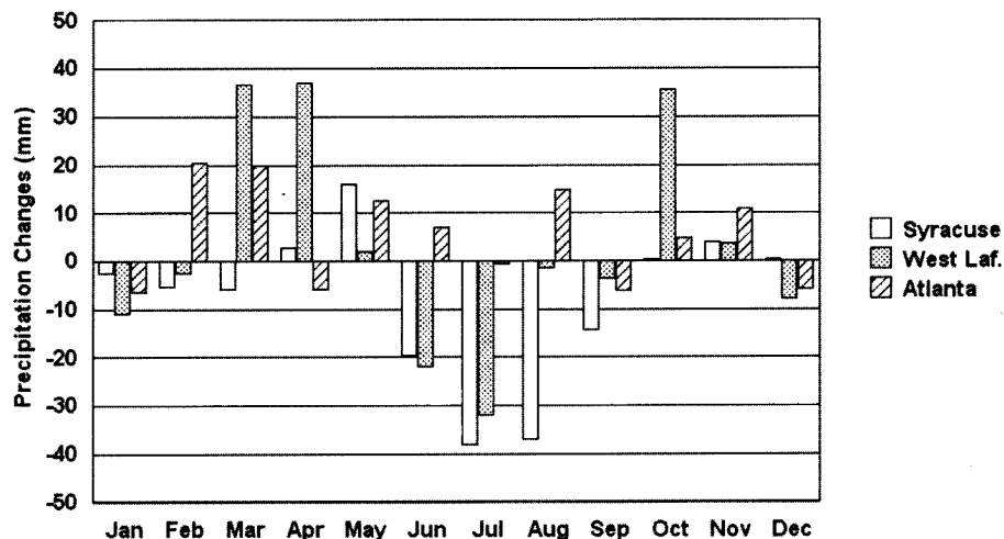
Figure 1. Changes predicted in the precipitation, by month, over the period of 1990–2099 for three locations.
