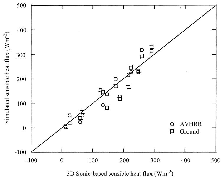
Fig. 3. Cross-plot of 3D Sonic-based estimates of sensible heat flux and those simulated using ground-based and AVHRR-based surface temperature (in \text{Wm}^{-2} ).
