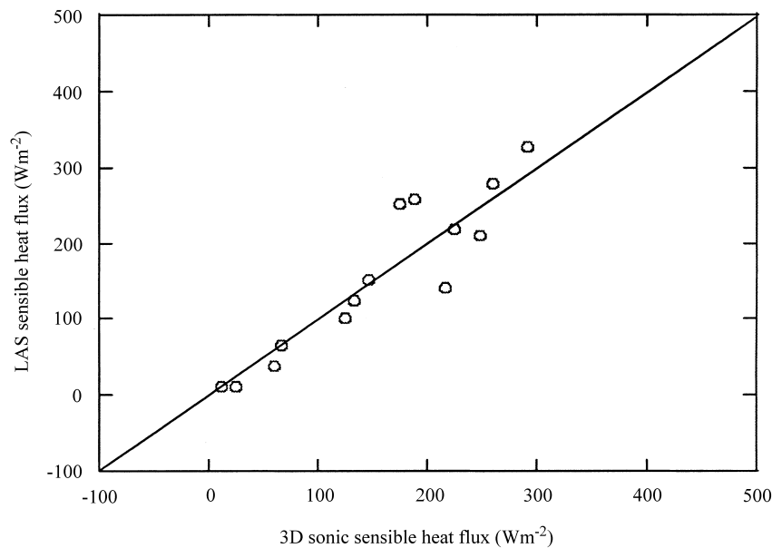
Fig. 1. Comparison between sensible heat flux values obtained from the 3D sonic and those obtained from the scintillometer (LAS) (in \text{W m}^{-2} ).
