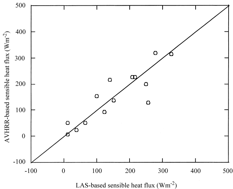
Fig. 4. Comparison of scintillometer- and AVHRR-based estimates of sensible heat flux values (in \text{W m}^{-2} ).
