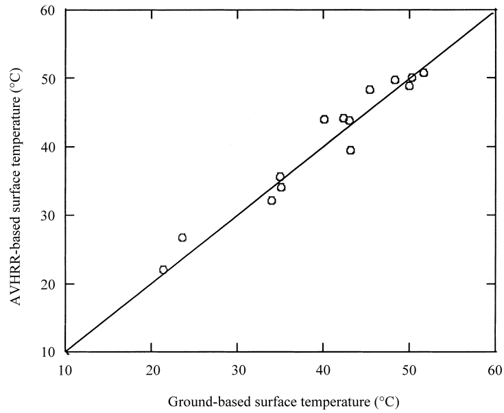
Fig. 2. Comparison of ground-based and AVHRR-based estimates of surface temperature (in °C).
