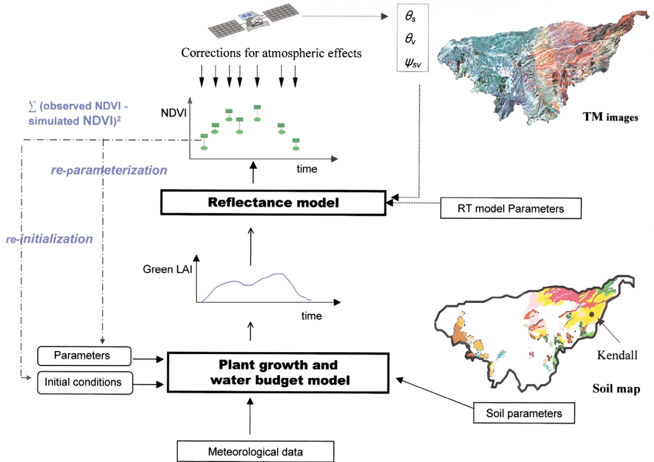
Fig. 2. Synoptic view of the approach used to refine the plant growth/soil water budget model to work on a spatially distributed basis using time series of Landsat TM and ETM+ images.
