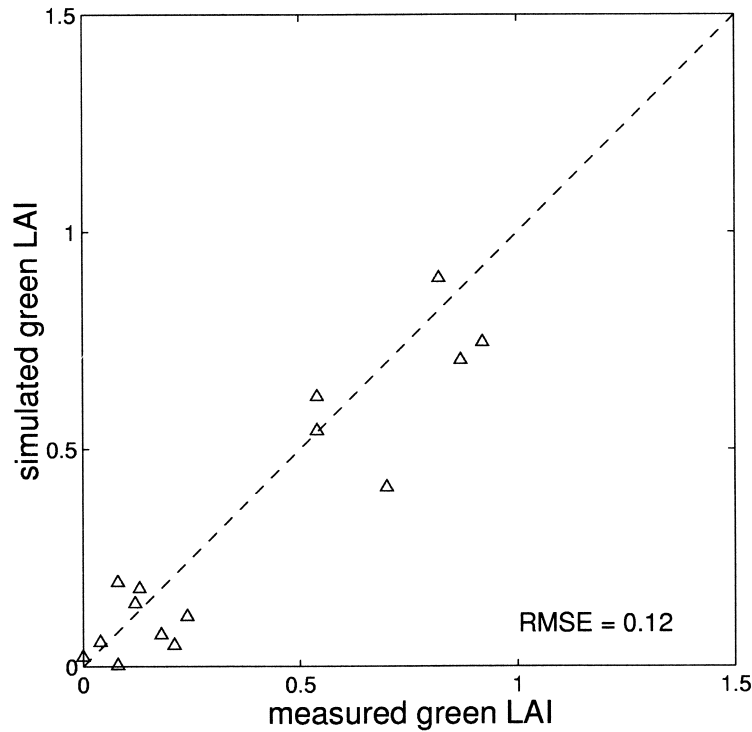
Fig. 7. Comparison of the GLAI simulated after model calibration and the GLAI measured at Kendall site.
