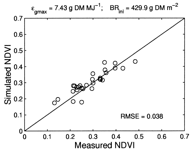
Fig. 8. Comparison of the NDVI simulated after model calibration and the NDVI measured by TM and ETM+ sensors.
