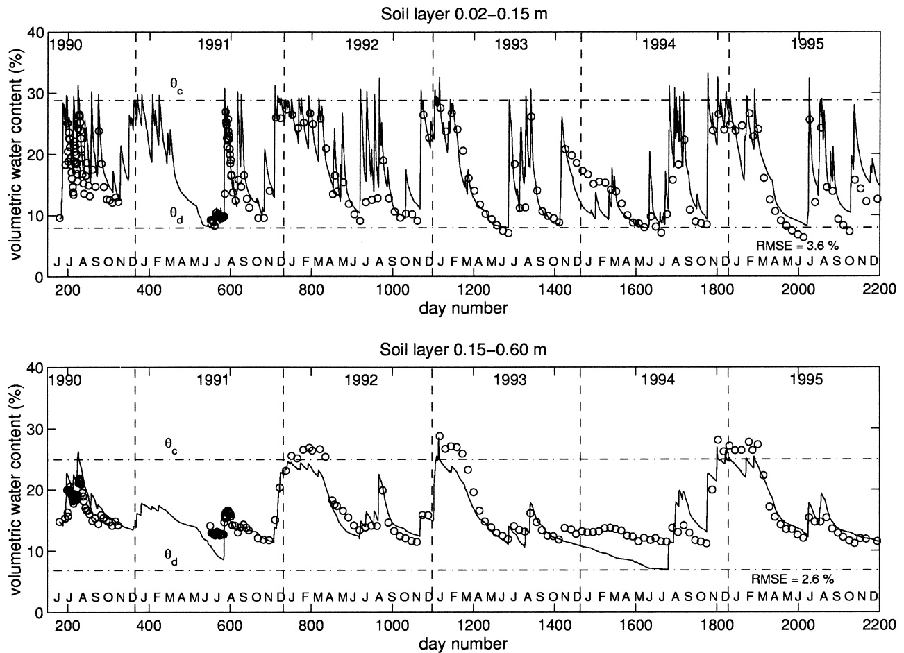
Fig. 9. Volumetric soil water content of layers 0.02–0.15 and 0.15–0.60 m. Solid lines refer to simulations and circles refer to measurements. Broken lines show field capacity and soil water content at air dryness.
