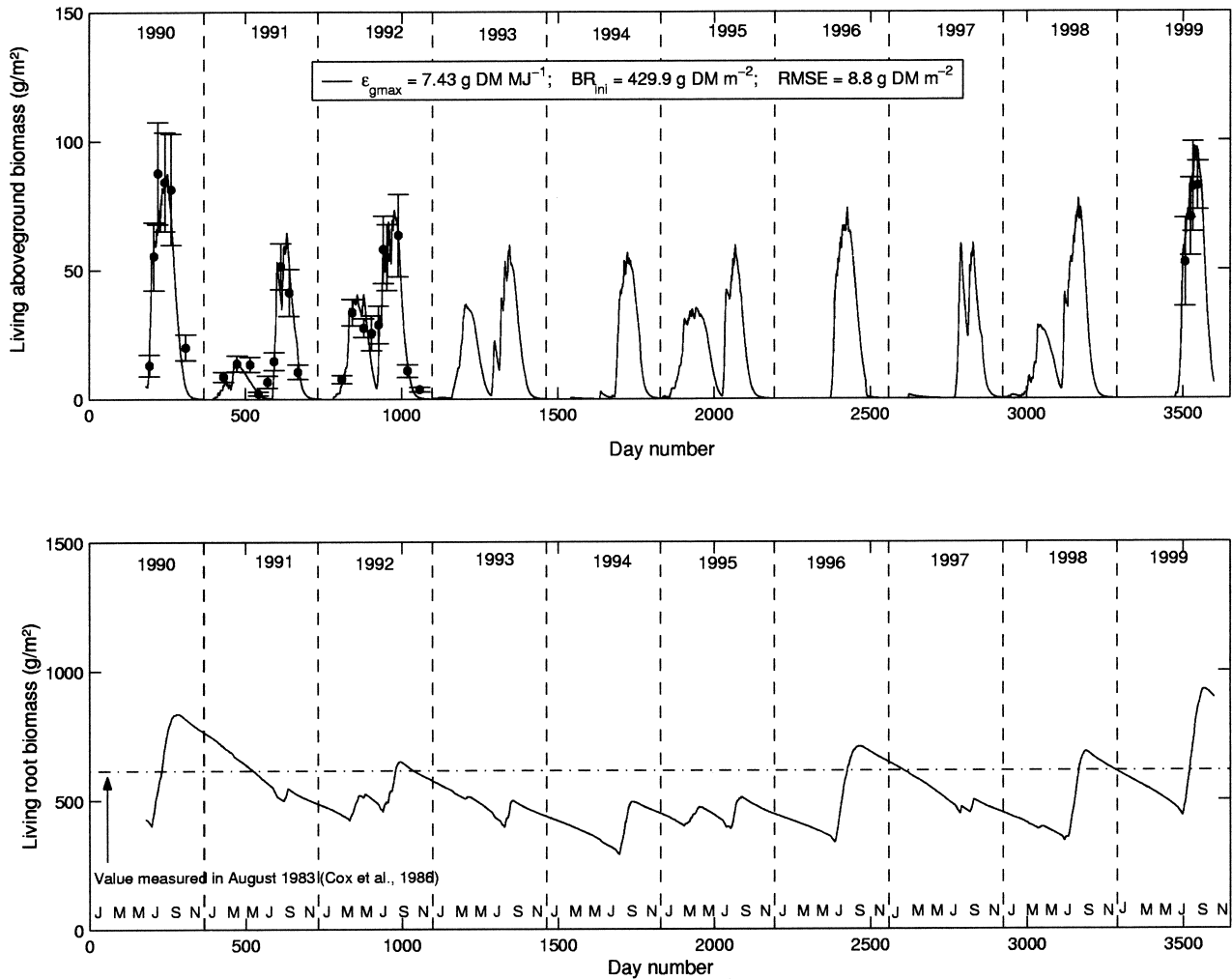
Fig. 6. Simulation results obtained at the Kendall site after model calibration using TM and ETM+ images (continuous lines). The retrieved values of \epsilon_{gmax} and BR_{ini} are indicated on the figure. In the top graph, solid circles with error bars show aboveground biomass measurements. In the bottom graph, the horizontal broken line show the value of root biomass measured by Cox et al. (1986) in August 1983.
