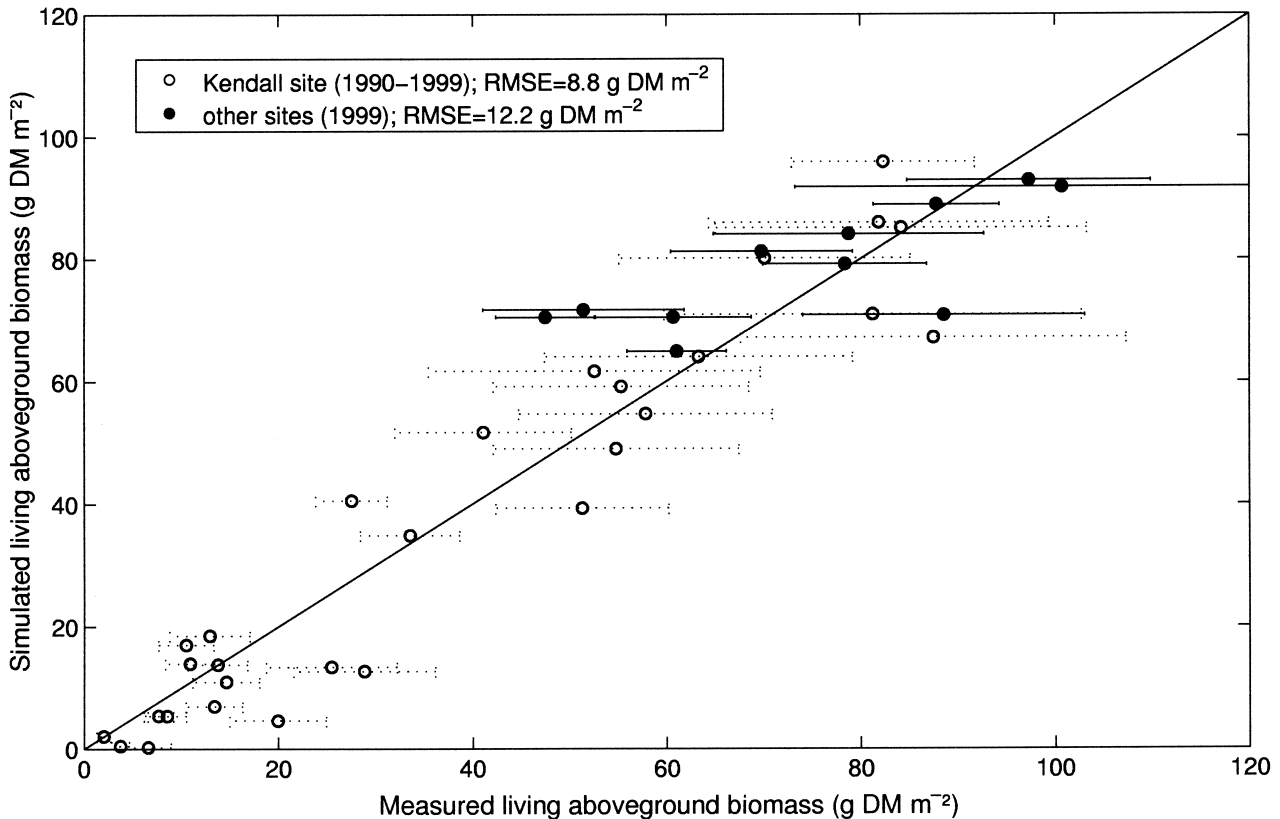
Fig. 10. Comparison of simulated and measured living aboveground biomass.
