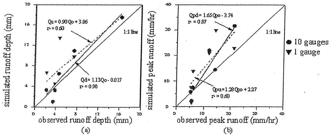
Figure 3. Simulation results for six runoff events on Watershed 11 with linear regression models between simulated and observed values superimposed for (a) total runoff depth, and (b) peak runoff rate, where Q_o =observed runoff depth, Q_d =simulated runoff depth with distributed rainfall, Q_u =simulated runoff depth with uniform rainfall, Q_{pu} =simulated peak runoff rate with uniform rainfall. Simulations were performed using distributed (10 gauges) and uniform (1 gauge) rainfall; solid lines represent regressions for distributed rainfall; dashed lines for uniform rainfall.
