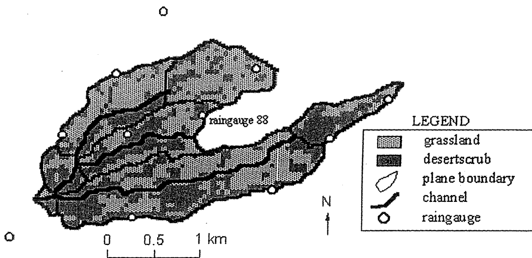
Figure 2. Configuration of Watershed 11 used to parameterize SWAT and KINEROS. Note that there are 17 elements; 2 upland, 10 lateral, and 5 channel elements. The 10 raingauges used to distribute rainfall are overlain with special emphasis placed on gauge 88, which was used to simulate uniform rainfall. The uppermost section of the watershed is excluded because it drains to a retention pond that did not yield runoff during the simulation period.
