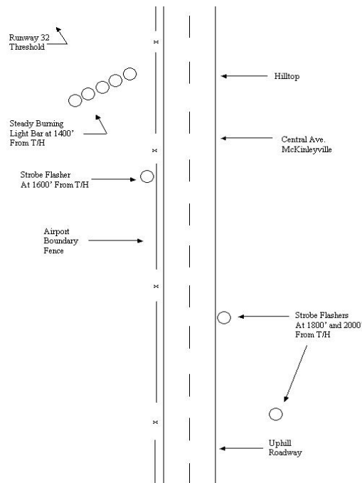
FIGURE 1. PLOT PLAN OF THE RUNWAY 32 APPROACH AREA
