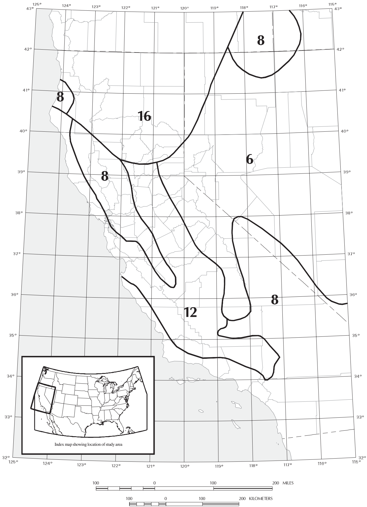
FIGURE 3.3-17 LONG-PERIOD TRANSITION PERIOD, T_L (sec), FOR REGION 1
