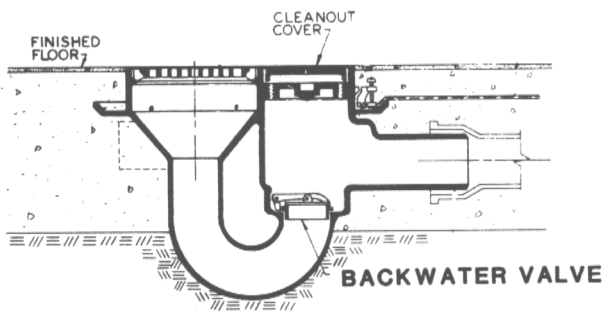
FLOOR DRAIN WITH INTEGRAL BACKWATER VALVE
