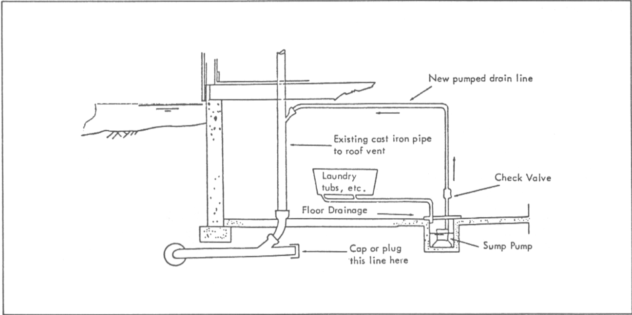
Figure IV-8. Elimination of Gravity Flow Basement Drains
