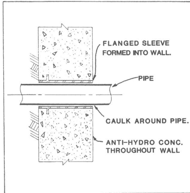
Figure IV-11. Waterproof Sleeve for Pipe Penetrations
