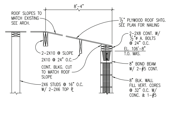
6 ROOF FRAMING AT BLOCK WALL 3/4"=1'-0"
