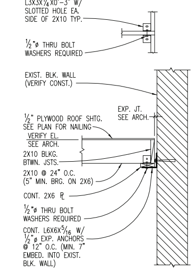
8 FRAMING AT EXIST. MAS. WALL 3/4"=1'-0"
