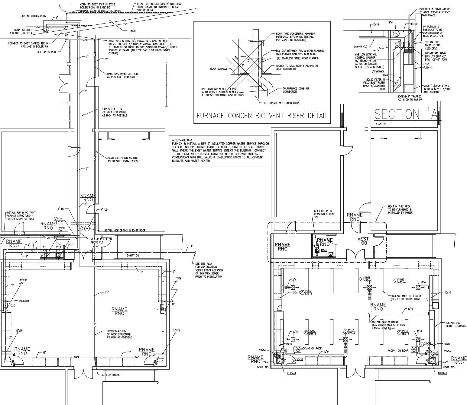
PLUMBING PLAN
