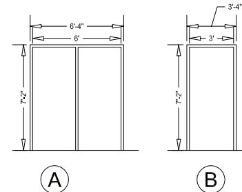
204 DOOR TYPE SCALE: 3/4" = 1'-0"
