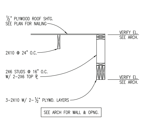
7 BEAM ABOVE GLASS FRAMING 3/4"=1'-0"
