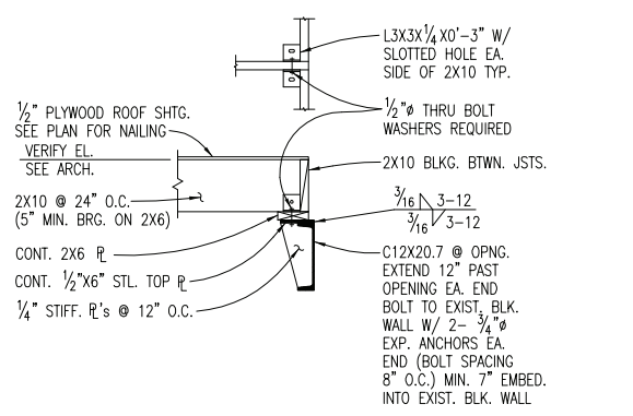
9 FRAMING AT STEEL BEAM 3/4"=1'-0"
