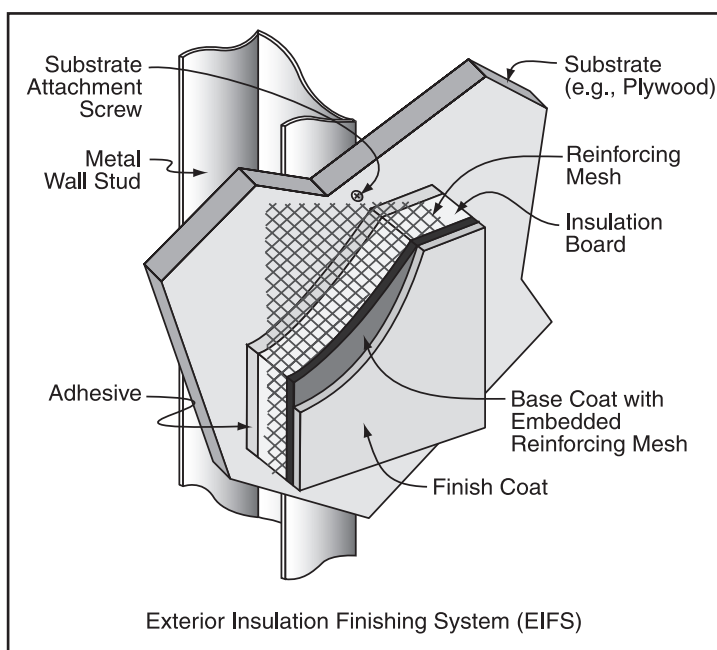
Figure 4. EIFS wall construction
