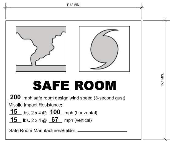
201 BUILDING I.D. SIGN N.T.S.
