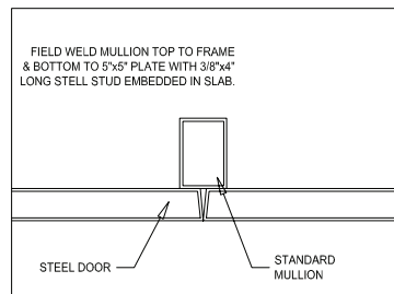
B MULLION
