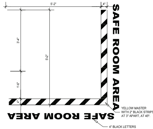
203 FLOOR SIGNAGE SCALE: 3/4" = 1'-0"
