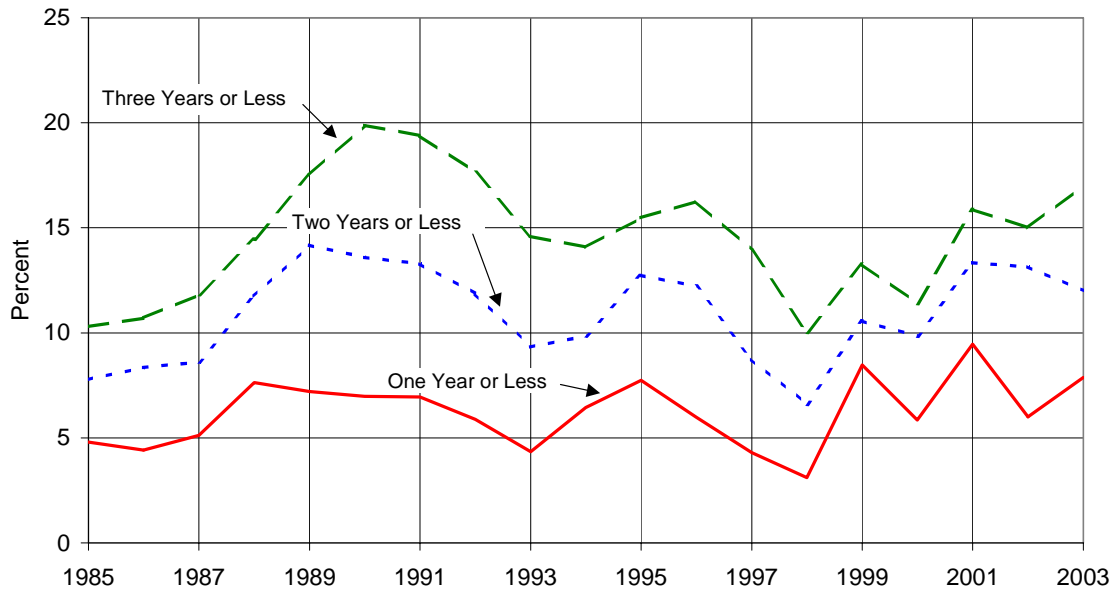
Figure 10c. Percent of Total Wellhead Capacity of Kansas Gas Wells by Age (Base Case)
