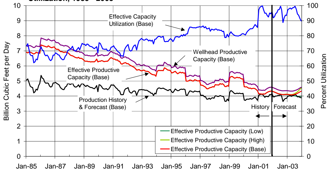
Figure 8a. Louisiana Monthly Dry Gas Production Rate, Wellhead Productive Capacity, and Effective Productive Capacity and Utilization, 1985 - 2003
