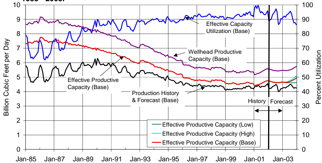
Figure 7a. Oklahoma Monthly Dry Gas Production Rate, Wellhead Productive Capacity, and Effective Productive Capacity and Utilization, 1985 - 2003.
