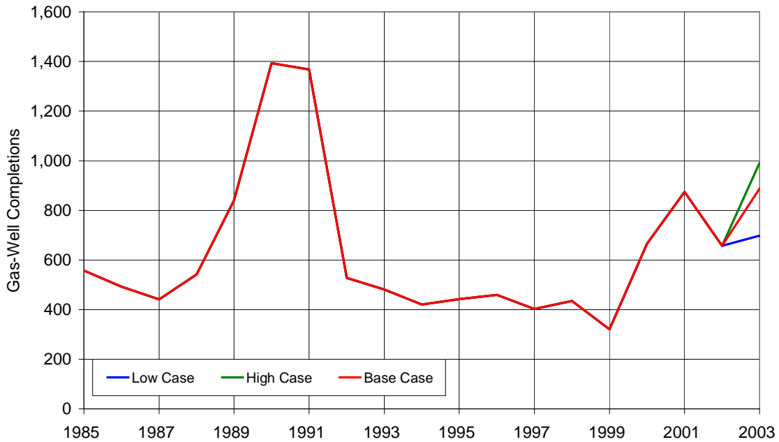
Figure 13b. Southeast Gas-Well Completions Added During Year, 1985-2003
