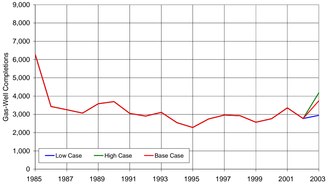
Figure 14b. Eighteen States Gas-Well Completions Added During Year, 1985-2003
