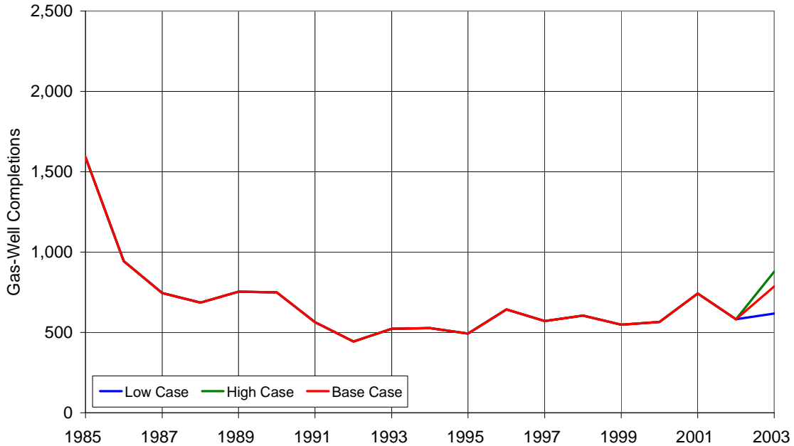
Figure 8b. Louisiana Gas-Well Completions Added During Year, 1985-2003
