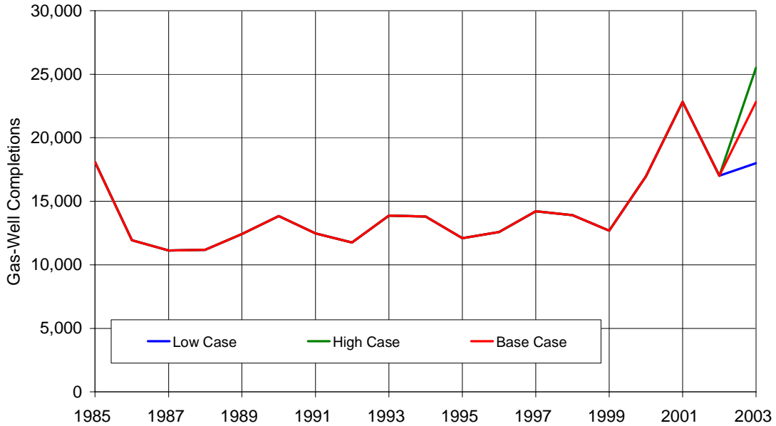
Figure 4b. Lower 48 States Gas-Well Completions Added During Year, 1985-2003
