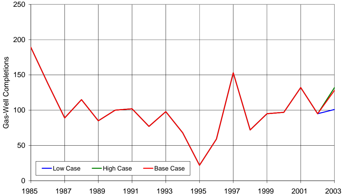
Figure 9b. California (Including Pacific OCS) Gas-Well Completions Added During Year, 1985-2003
