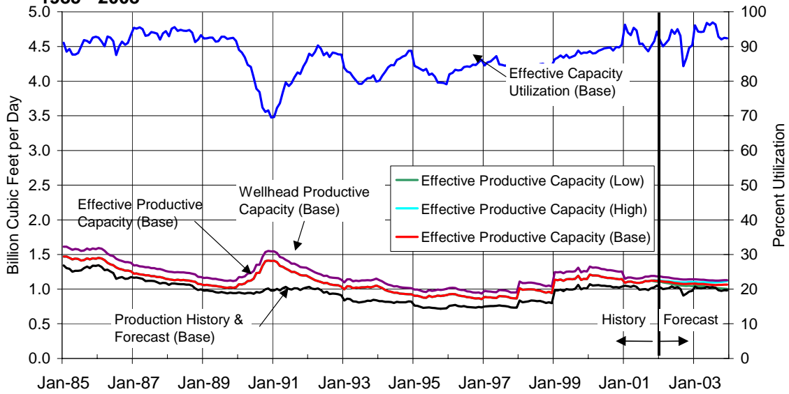
Figure 9a. California Monthly Dry Gas Production Rate, Wellhead Productive Capacity, and Effective Productive Capacity and Utilization, 1985 - 2003
