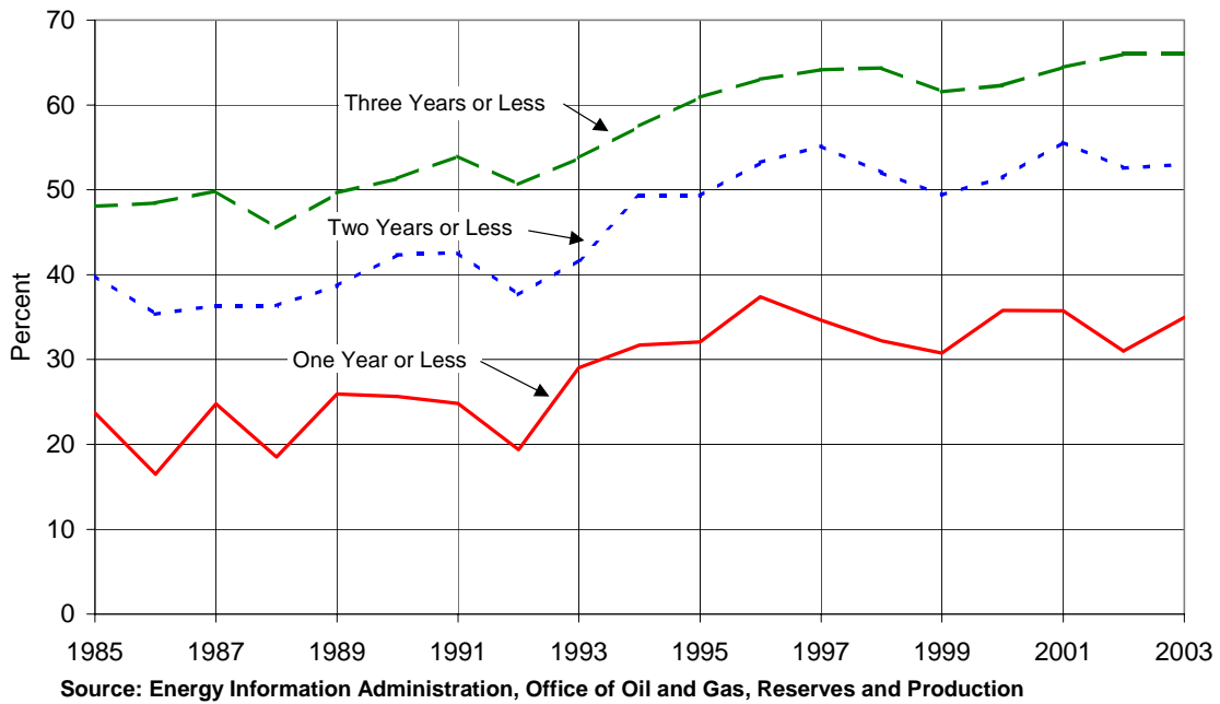
Figure 5c. Percent of Total Wellhead Capacity of Gulf of Mexico OCS Gas Wells by Age (Base Case)
