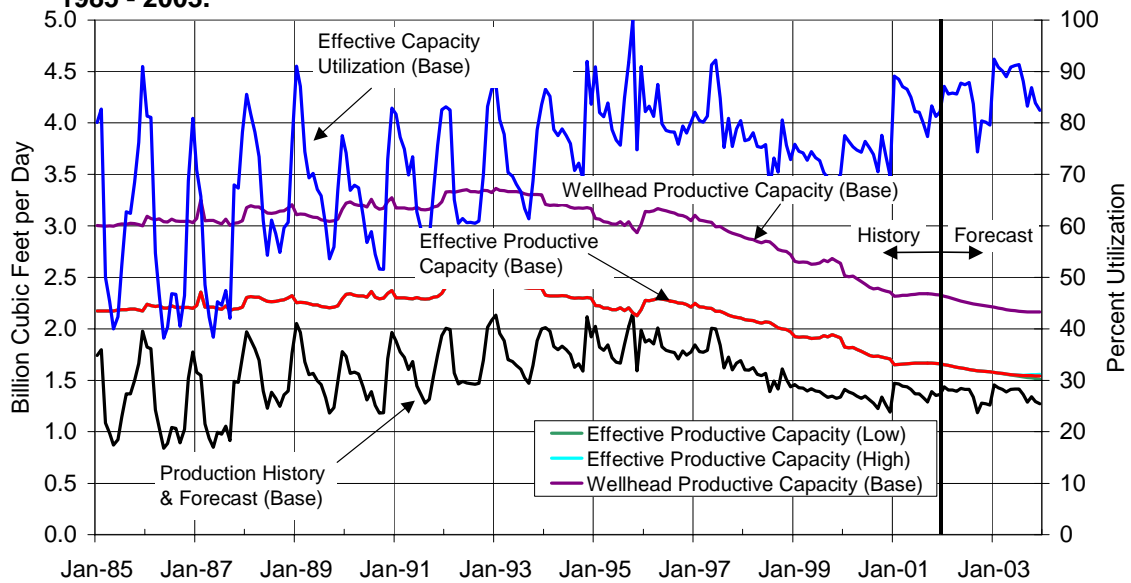
Figure 10a. Kansas Monthly Dry Gas Production Rate, Wellhead Productive Capacity, and Effective Productive Capacity and Utilization, 1985 - 2003.
