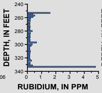
Core Hole 17, Peabody Natural Gas, Inc. PNG 31-1 core hole major, minor, and trace element determination [ppm, parts per million].
