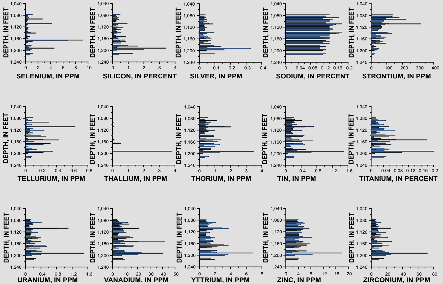
Core Hole 2, MichiWest Energy, Inc., Pilot 16-32 core hole major, minor, and trace element determination [ppm, parts per million].
