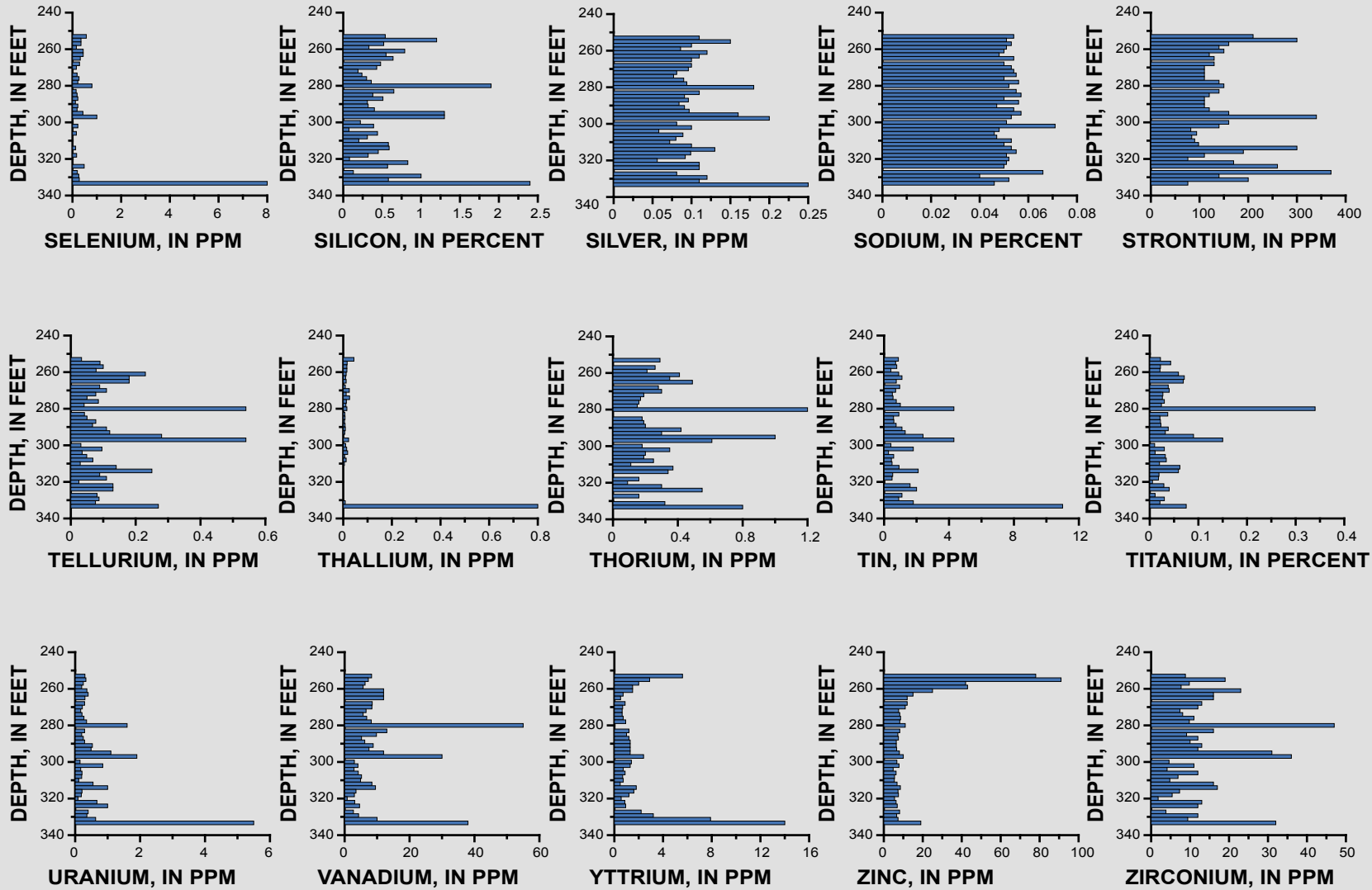
Core Hole 17, Peabody Natural Gas, Inc. PNG 31-1 core hole major, minor, and trace element determination [ppm, parts per million].
