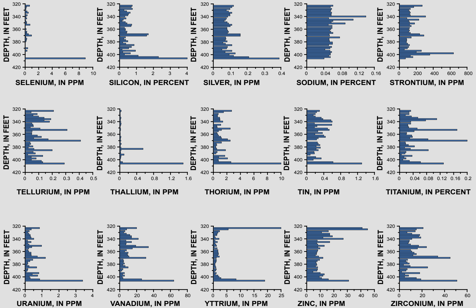
Core Hole 18, Peabody Natural Gas, Inc. PNG 35-1 core hole major, minor, and trace element determination [ppm, parts per million].
