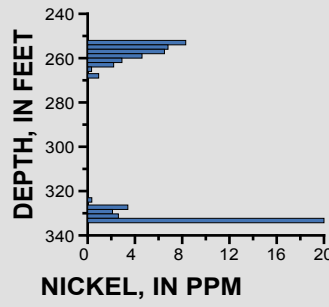
Core Hole 17, Peabody Natural Gas, Inc. PNG 31-1 core hole major, minor, and trace element determination [ppm, parts per million].
