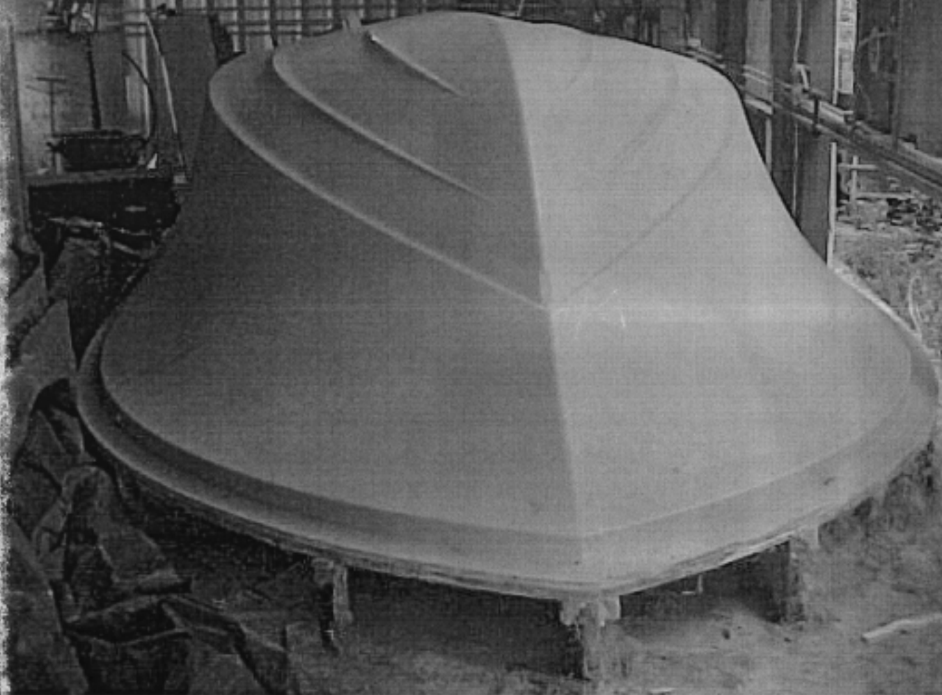
POLAR 1810 V BAY BOAT HULL PLUG FWD VIEW
