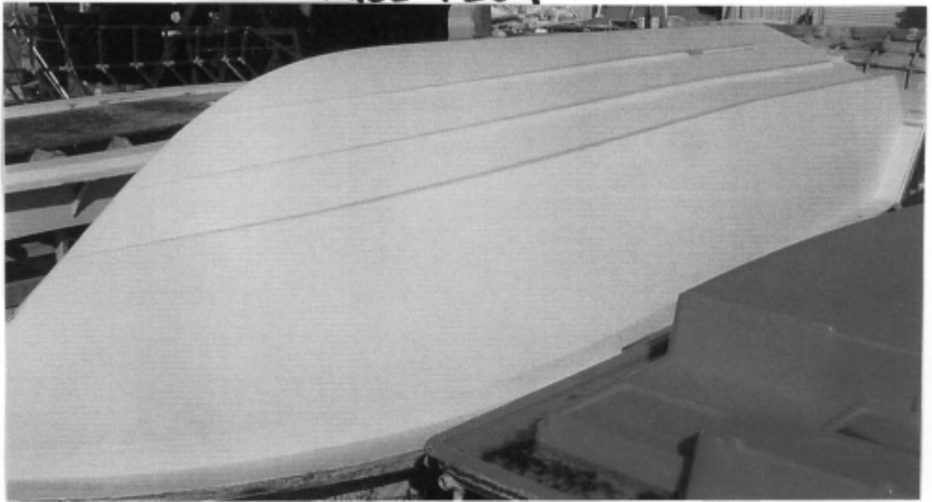
HULL PLUG
