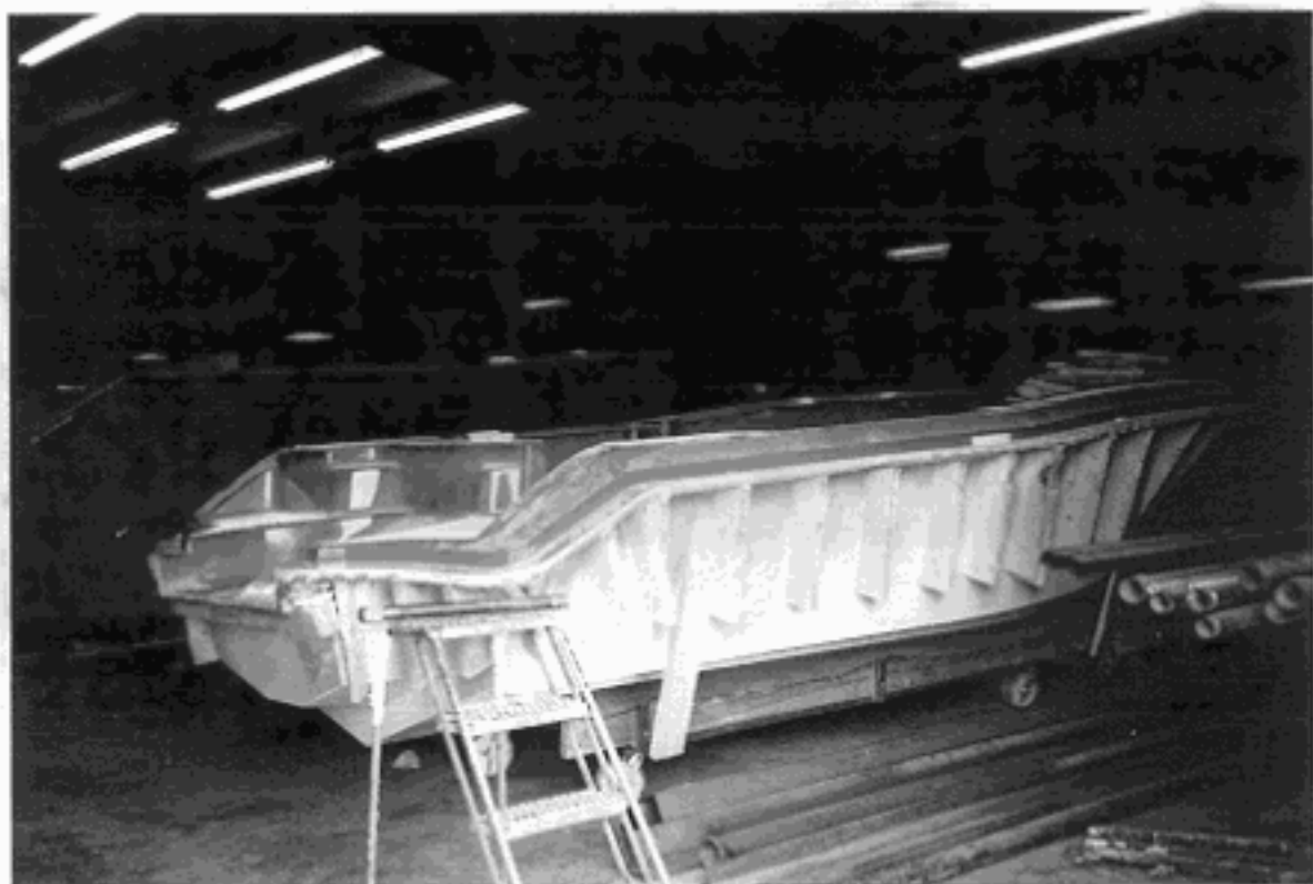
STBD SIDE DECK PLUG BUSSEEL AND DECK PROFILE VIEW ORIGINAL DECK PLUG
