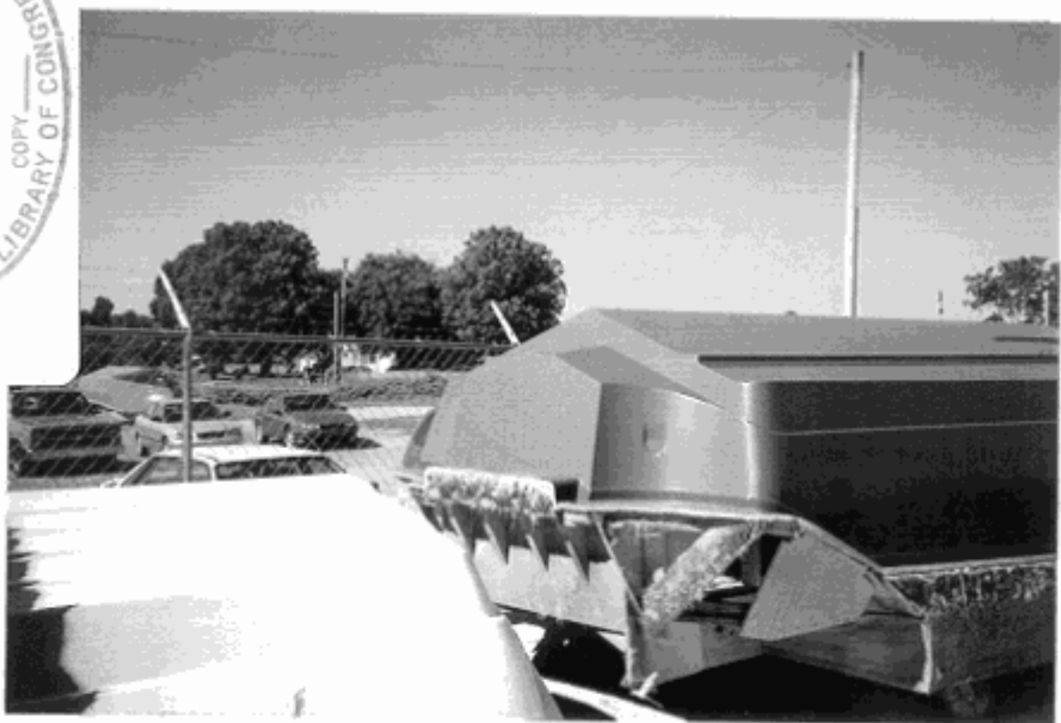
PLUG PORT SIDE QUARRING VIEW STERN BUSSEL ORIGINAL HULL PLUG
