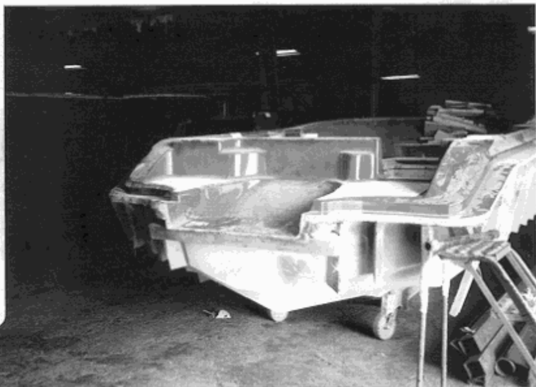
DECK PLUG STERN VIEW BUSSEEL AREA ORIGINAL DECK PLUG .
