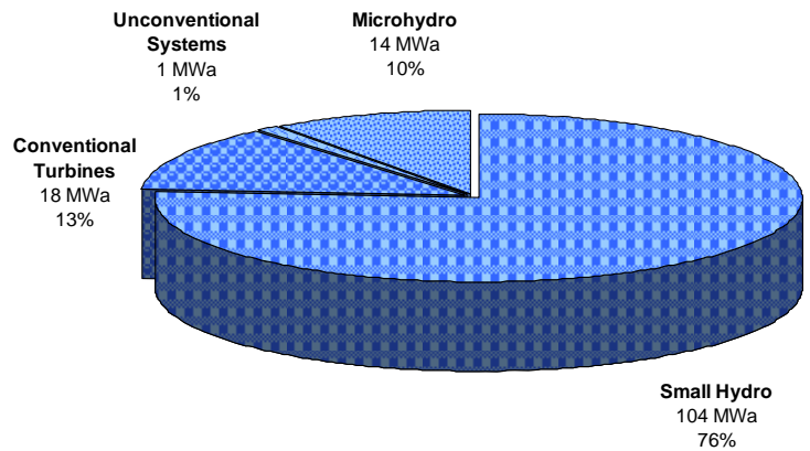
(b) Total Feasible Project Hydropower Potential 136 MWa
