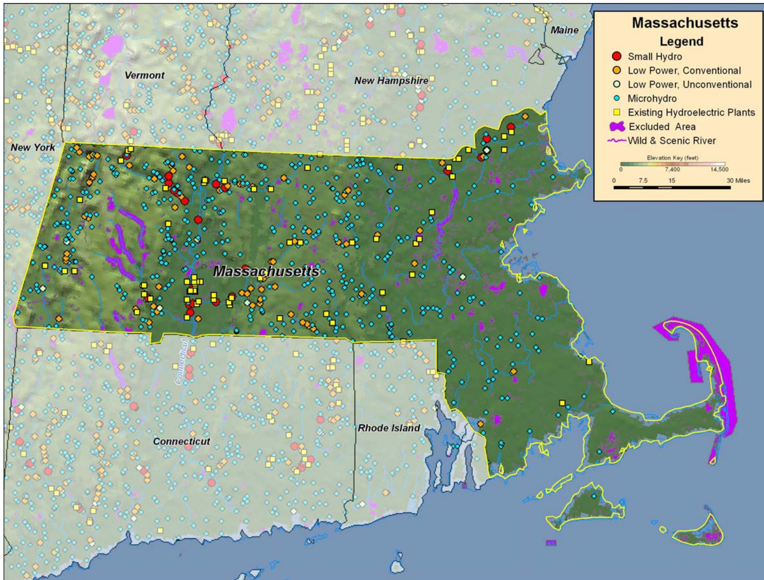
Figure B-105. Low power and small hydropower feasible projects, and existing hydroelectric plants in Massachusetts.
