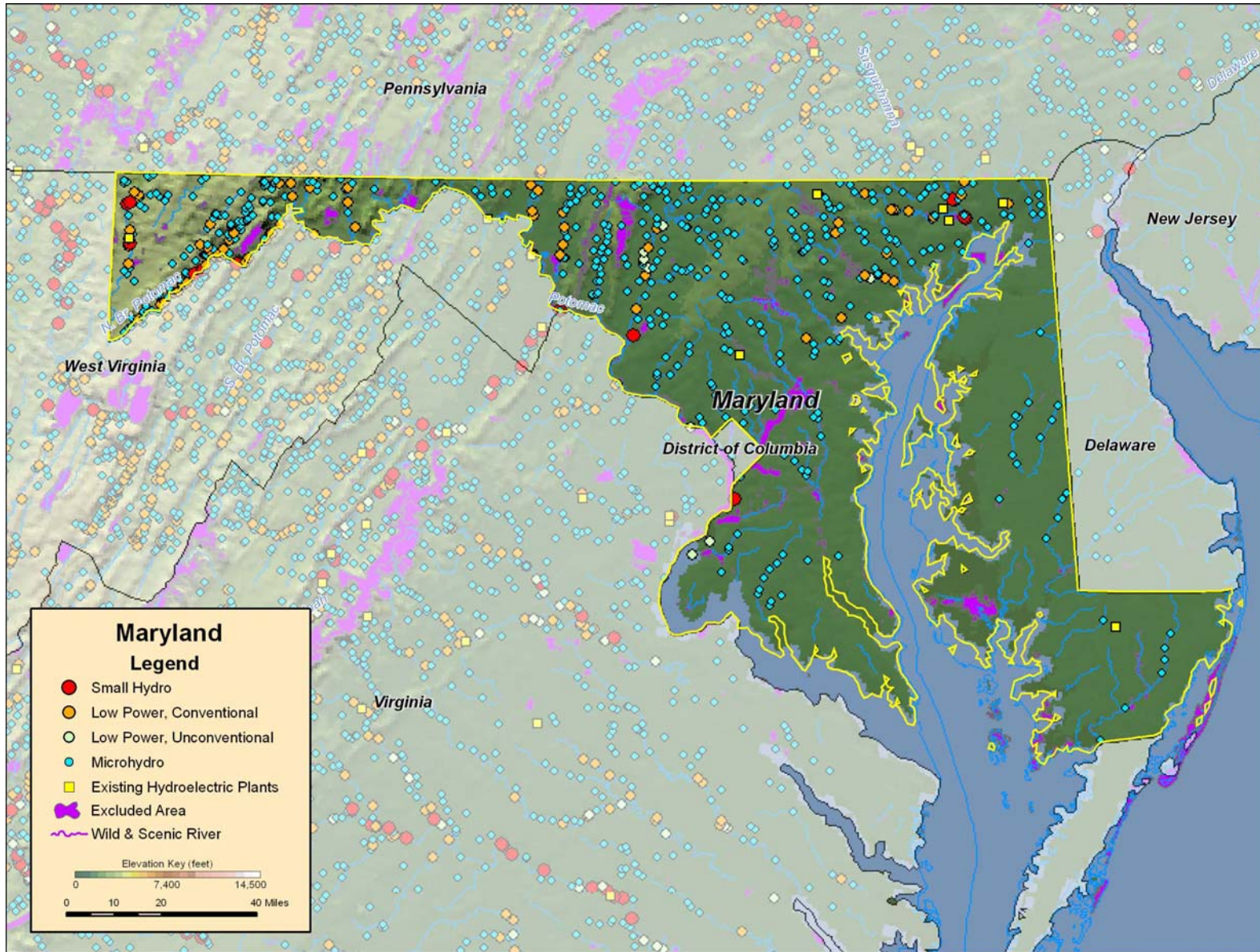
Figure B-100. Low power and small hydropower feasible projects, and existing hydroelectric plants in Maryland.
