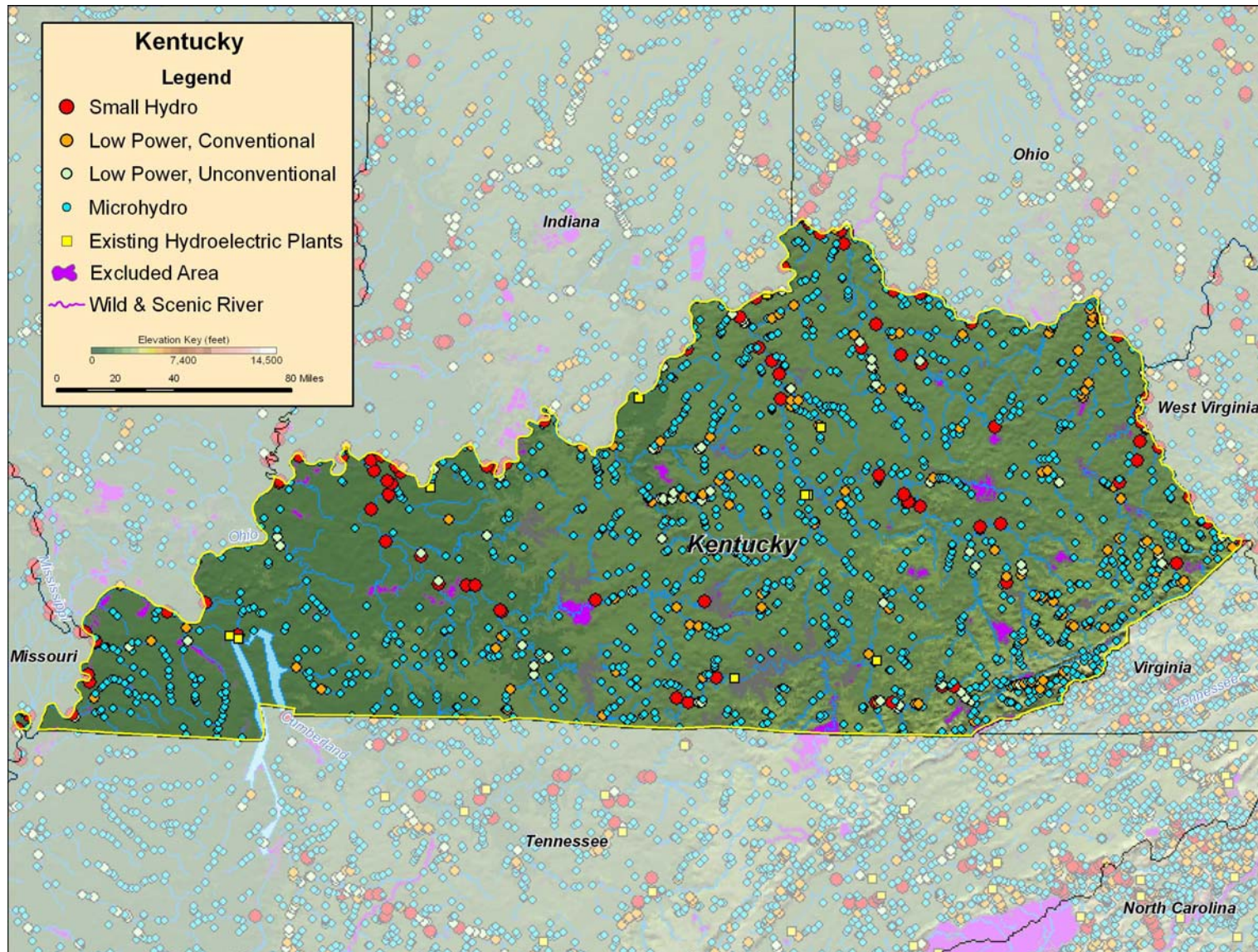
Figure B-85. Low power and small hydropower feasible projects, and existing hydroelectric plants in Kentucky.
