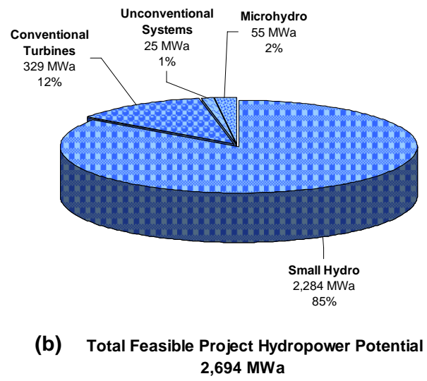
Figure B-7. Distribution of the (a) number and (b) total hydropower potential of the low power and small hydropower feasible projects in Alaska with the low power projects divided into technology classes.
