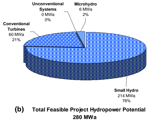
Figure B-52. Distribution of the (a) number and (b) total hydropower potential of the low power and small hydropower feasible projects in Hawaii with the low power projects divided into technology classes.
