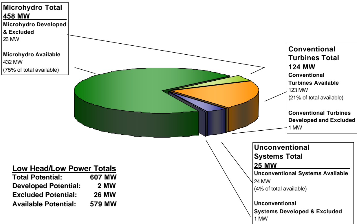
Figure A-79. Distribution of the low head/low power power potential (annual mean power) of water energy resources in the Great Basin Region (HUC 16) among three low head/low power hydropower technology classes.
