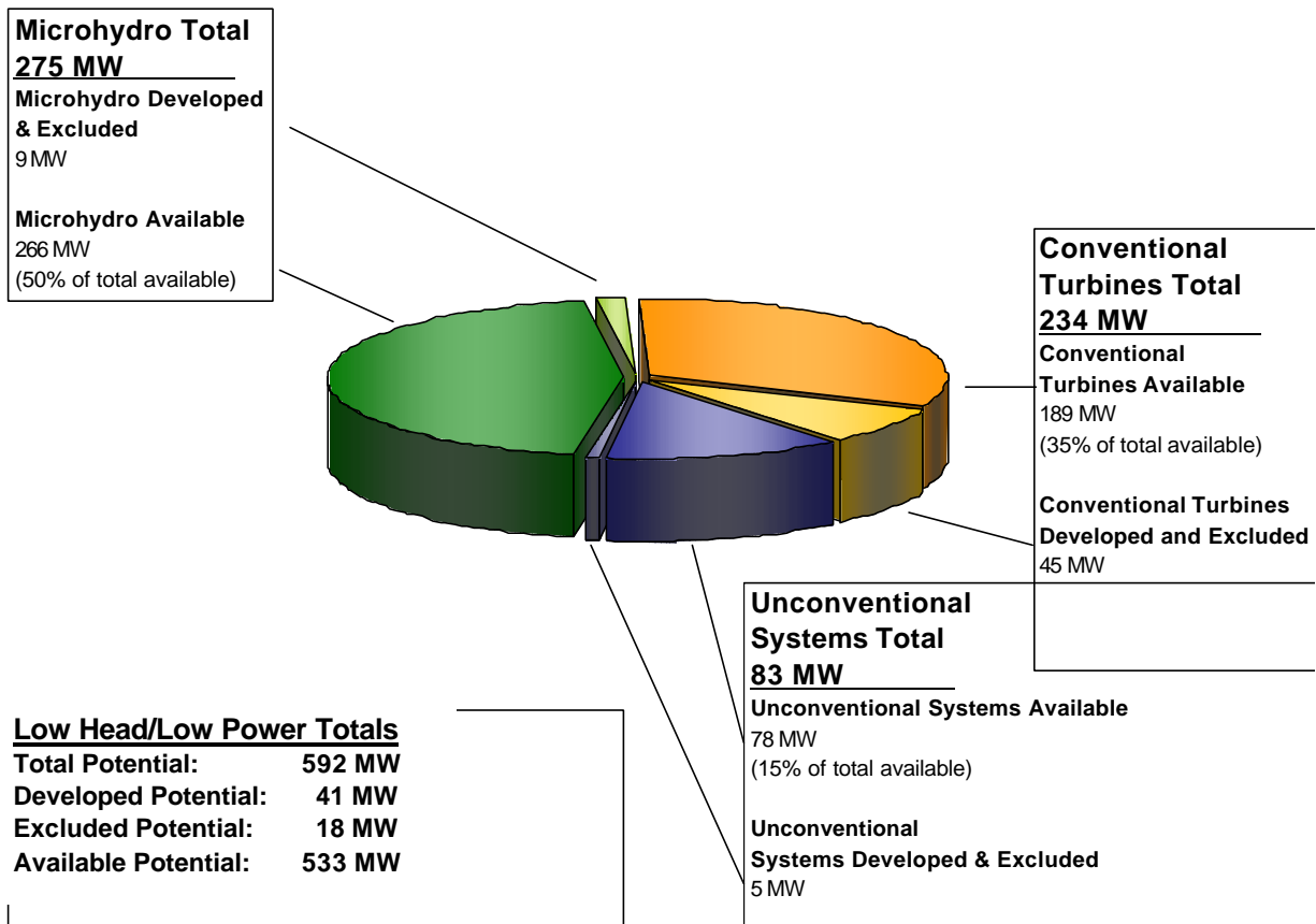
Figure A-4. Distribution of the low head/low power power potential (annual mean power) of water energy resources in the North Atlantic Region (HUC 1) among three low head/low power hydropower technology classes.
