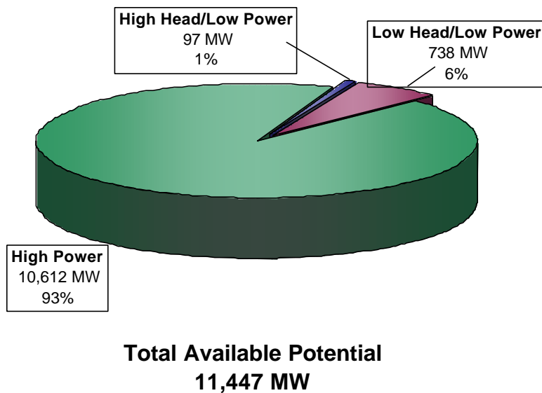
Figure A-38. Power class distribution of the available power potential (annual mean power) of water energy resources in the Lower Mississippi Region (HUC 8).
