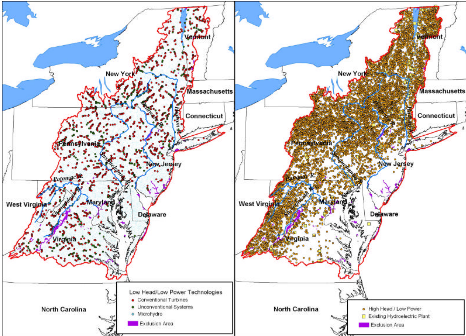
Figure A-10. Low head/low power and high head/low power water energy sites, and existing hydroelectric plants in the Middle Atlantic Region (HUC 2).
