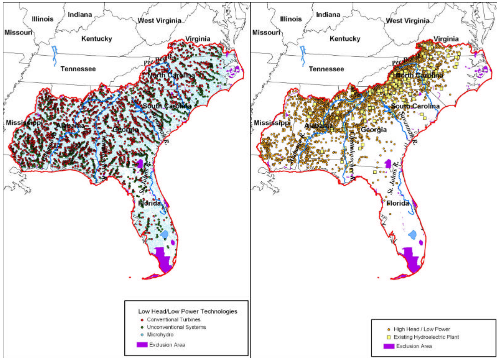
Figure A-15. Low head/low power and high head/low power water energy sites, and existing hydroelectric plants in the South Atlantic-Gulf Region (HUC 3).
