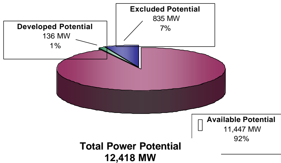
Figure A-37. Power category distribution of the total power potential (annual mean power) of water energy resources in the Lower Mississippi Region (HUC 8).
