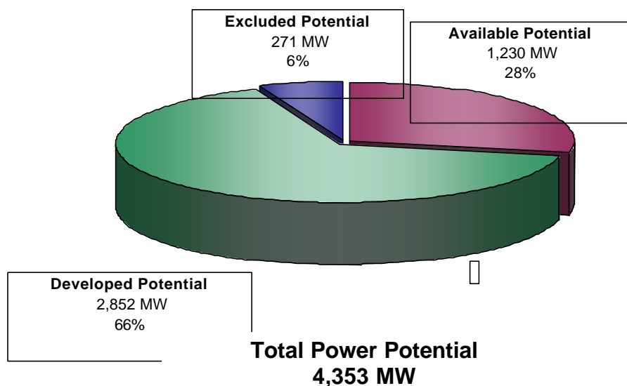
Figure A-17. Power category distribution of the total power potential (annual mean power) of water energy resources in the Great Lakes Region (HUC 4).
