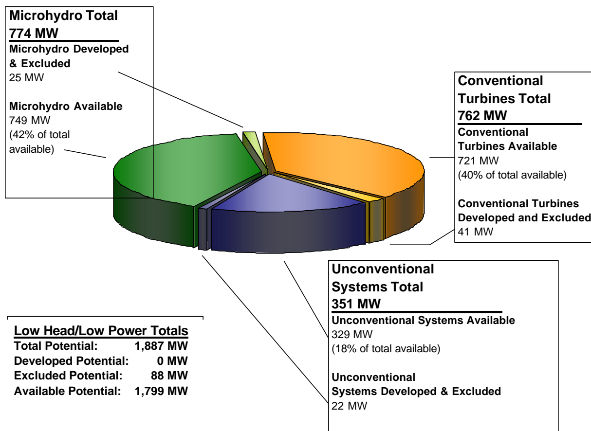
Figure A-54. Distribution of the low head/low power power potential (annual mean power) of water energy resources in the Arkansas-White-Red Region (HUC 11) among three low head/low power hydropower technology classes.
