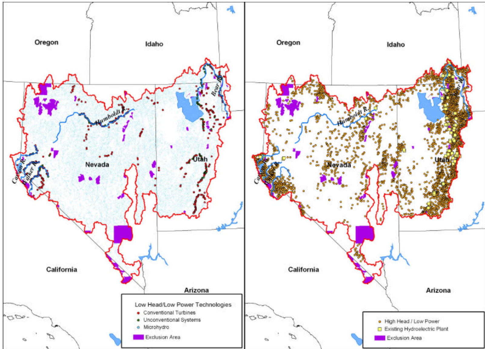
Figure A-80. Low head/low power and high head/low power water energy sites, and existing hydroelectric plants in the Great Basin Region (HUC 16).
