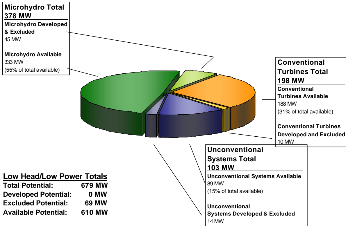
Figure A-69. Distribution of the low head/low power power potential (annual mean power) of water energy resources in the Upper Colorado Region (HUC 14) among three low head/low power hydropower technology classes.
