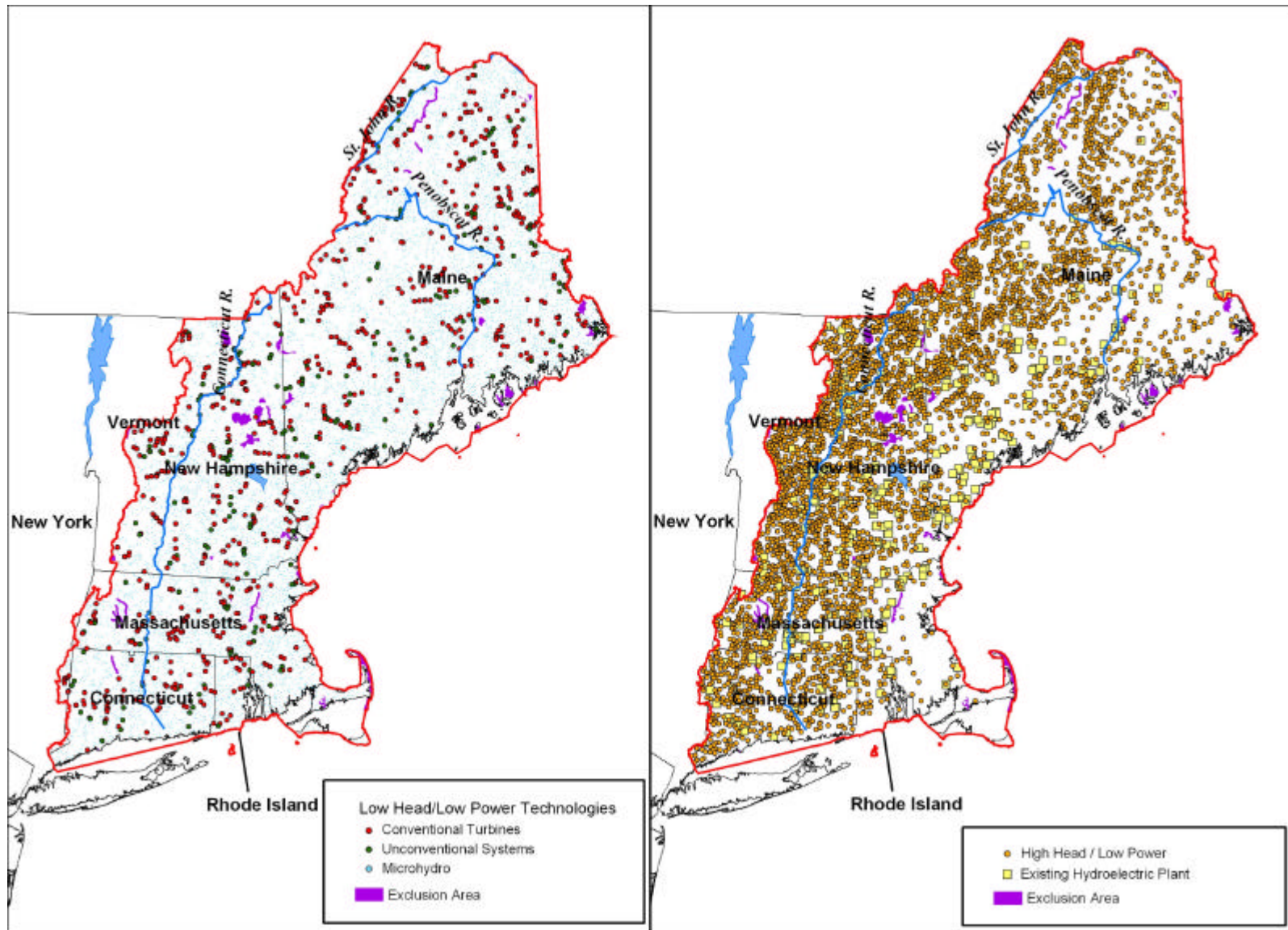
Figure A-5. Low head/low power and high head/low power water energy sites, and existing hydroelectric plants in the North Atlantic Region (HUC 1).
