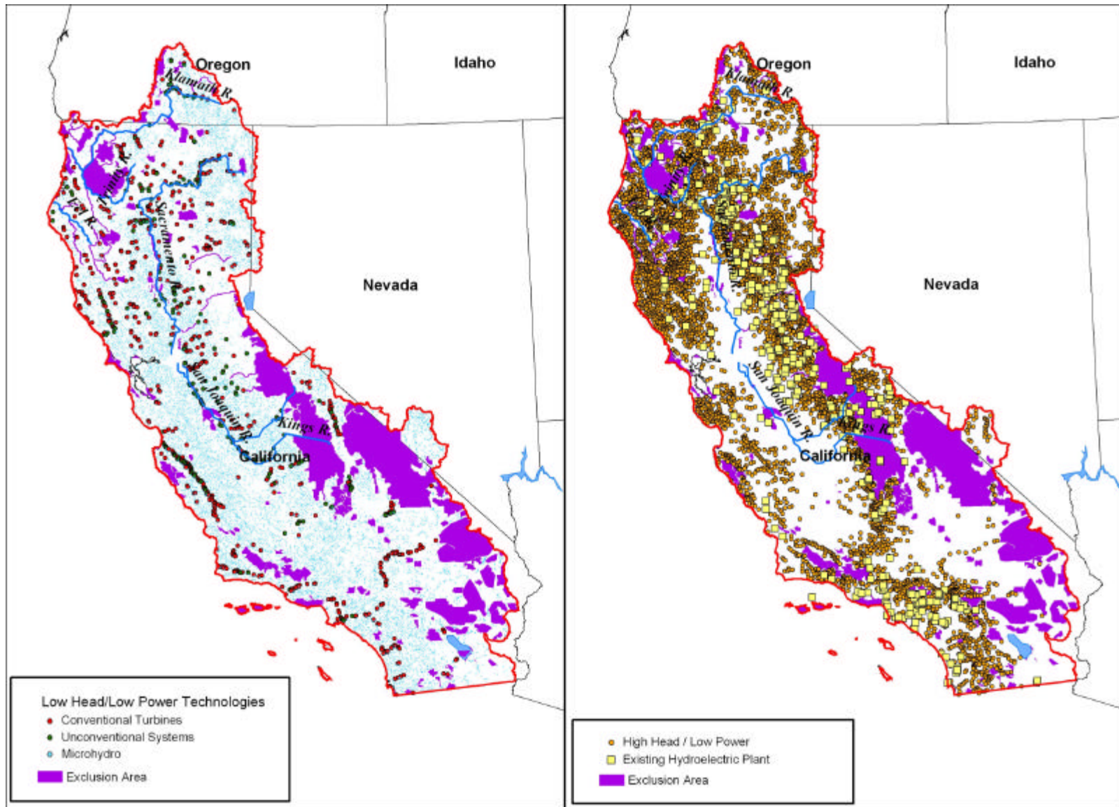
Figure A-90. Low head/low power and high head/low power water energy sites, and existing hydroelectric plants in the California Region (HUC 18).
