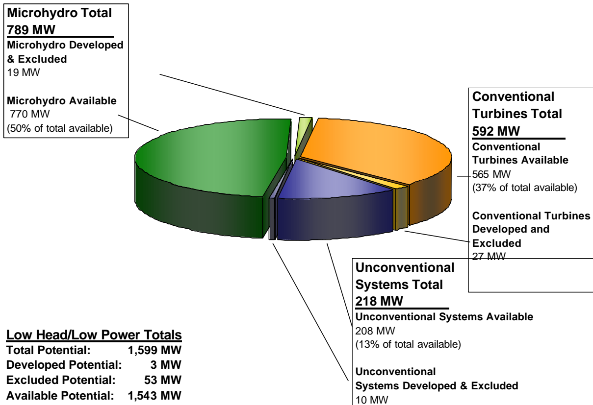
Figure A-24. Distribution of the low head/low power power potential (annual mean power) of water energy resources in the Ohio Region (HUC 5) among three low head/low power hydropower technology classes.
