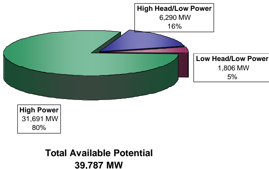
Figure A-83. Power class distribution of the available power potential (annual mean power) of water energy resources in the Pacific Northwest Region (HUC 17).
