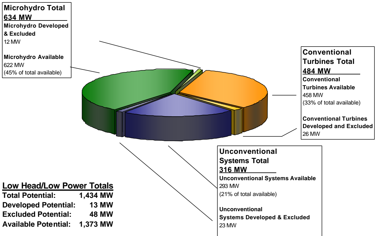
Figure A-34. Distribution of the low head/low power power potential (annual mean power) of water energy resources in the Upper Mississippi Region (HUC 7) among three low head/low power hydropower technology classes.
