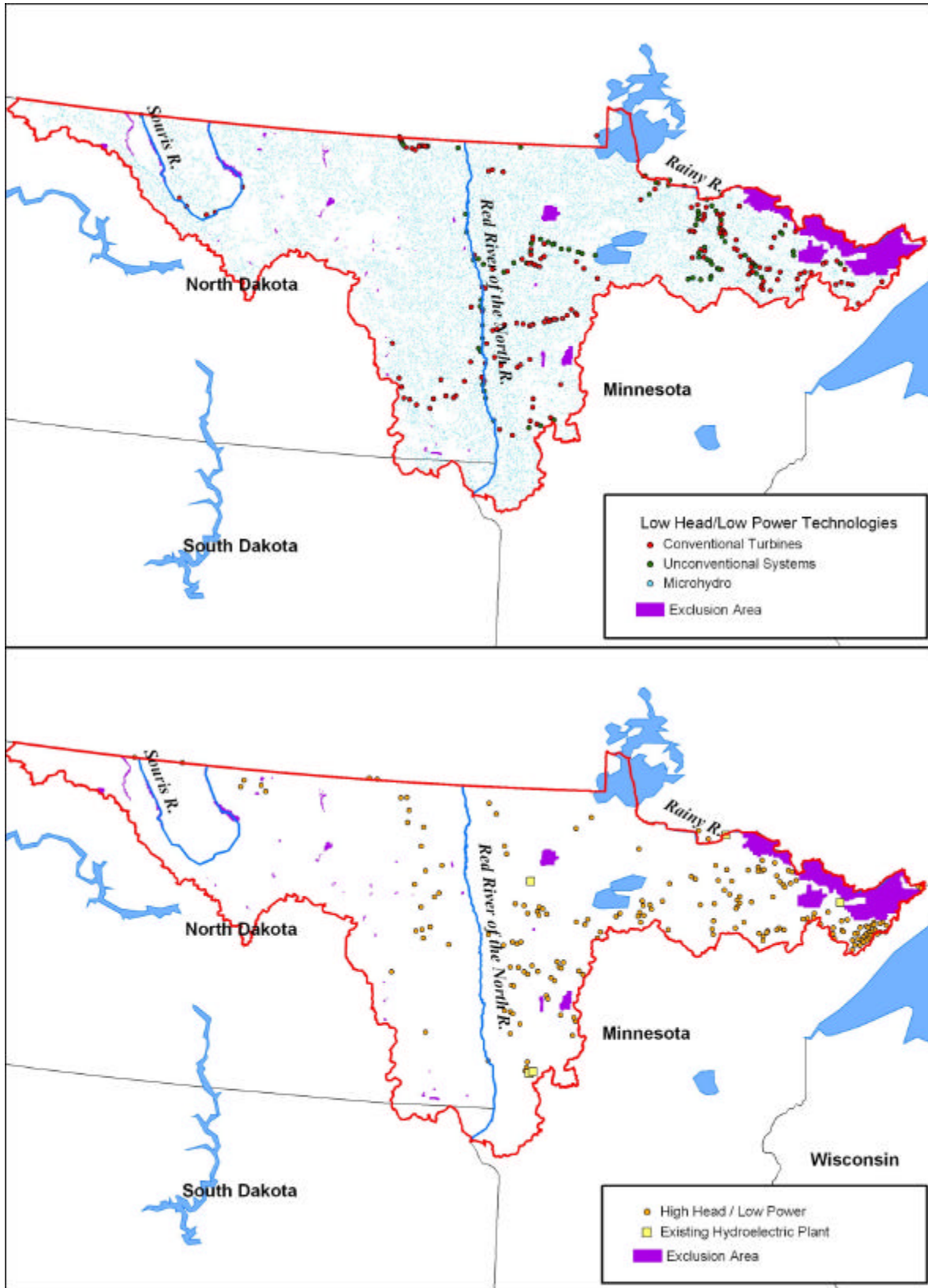
Figure A-45. Low head/low power and high head/low power water energy sites, and existing hydroelectric plants in the Souris Red-Rainy Region (HUC 9).
