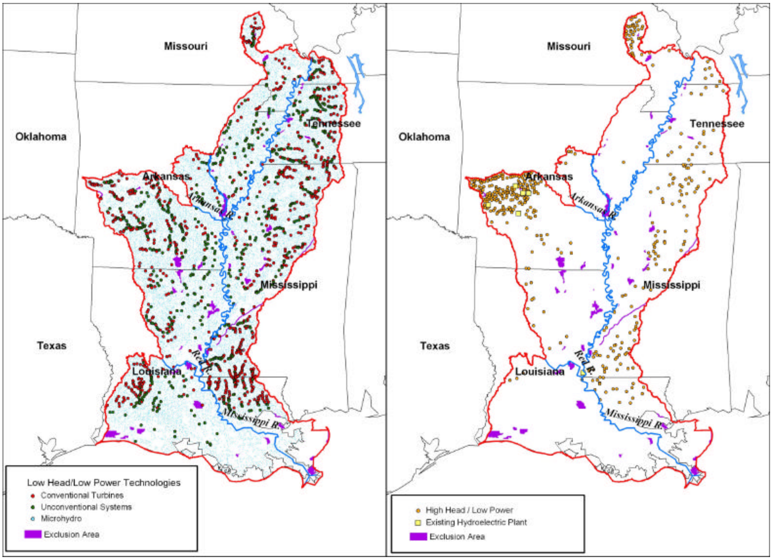
Figure A-40. Low head/low power and high head/low power water energy sites, and existing hydroelectric plants in the Lower Mississippi Region (HUC 8).
