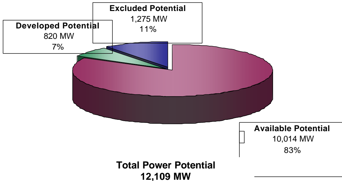
Figure A-22. Power category distribution of the total power potential (annual mean power) of water energy resources in the Ohio Region (HUC 5).
