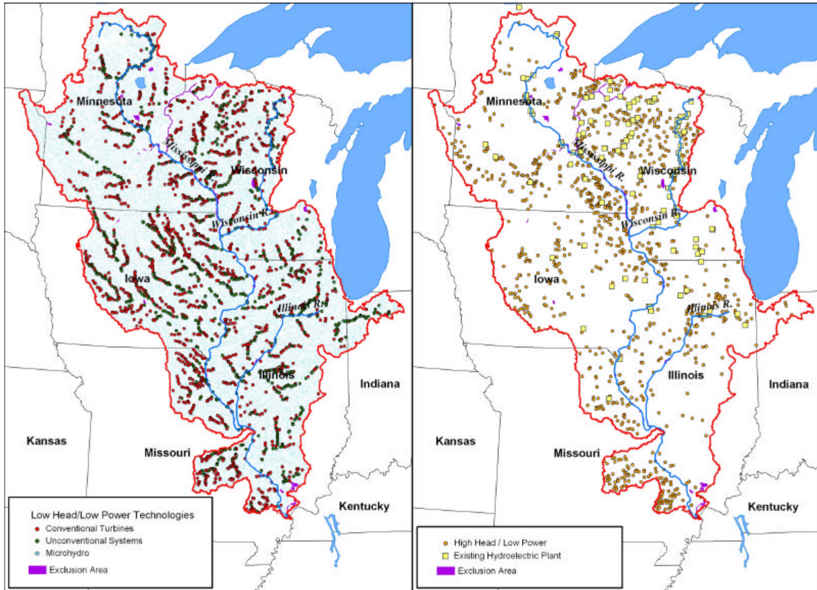
Figure A-35. Low head/low power and high head/low power water energy sites, and existing hydroelectric plants in the Upper Mississippi Region (HUC 7).
