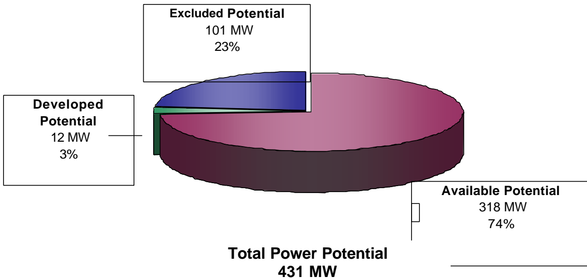
Figure A-42. Power category distribution of the total power potential (annual mean power) of water energy resources in the Souris Red-Rainy Region (HUC 9).
