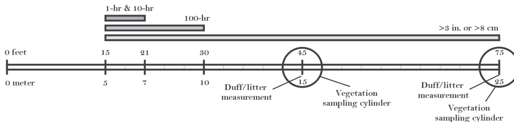
Figure FL-2 —Dead fuels, duff/litter, and vegetation data are recorded at specific locations on or along each sampling plane. The 1-hour and 10-hour fuels are sampled from the 15-ft (5-m) to the 21-ft (7-m) marks along the plane, the 100-hr fuels are sampled from the 15-ft (5-m) to the 30-ft (10-m) marks, and pieces 3 inches (8 cm) and larger are sampled between the 15-ft (5-m) and 75-ft (25-m) marks along the plane. Duff/litter measurements are made in a representative area within a 6-ft (2-m) diameter circular area at the 45-ft (15-m) and 75-ft (25-m) marks. The cover of live and dead vegetation is estimated within an imaginary 6-ft (2-m) diameter by 6-ft (2-m) high sampling cylinder at the 45-ft (15-m) and 75-ft (25-m) marks.
