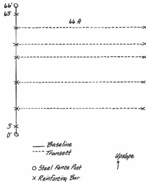
Figure HT-16 —Orient the baseline upslope with the zero end positioned at the lower point. Transects are oriented across the slope to limit the opportunity for erosion.
