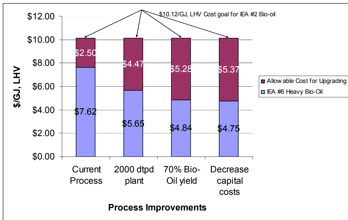
Figure 7. Bio-Oil Production and Upgrading Cost Goals
