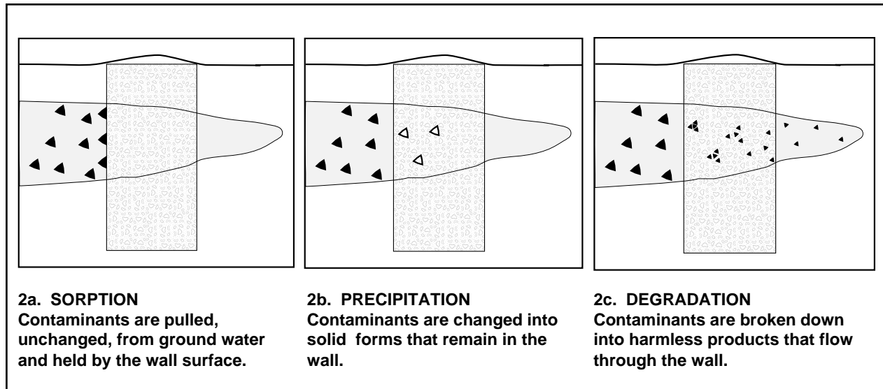
Figure 2. Sorption, Precipitation, and Degradation Treatment Walls
