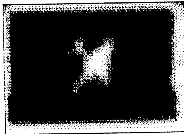
Figure 71- C-scan of AS4/PEEK ( \pm 45 ) 16s laminate at 6.5mm displacement.
