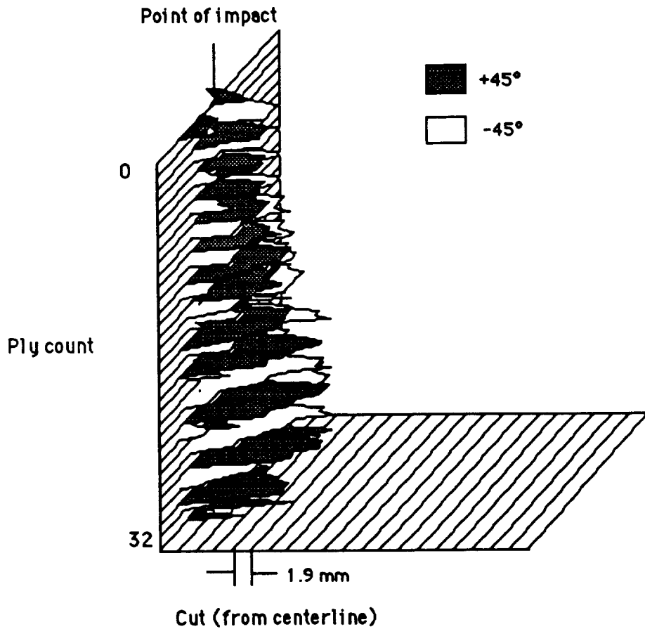
Figure 28 - Damage map of AS4/3501-6, (\pm 45)_{16s} after \Sigma I.E. = 80J.
