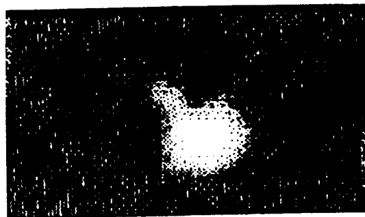
Figure 74 - C-scan of the damage of AS4/polycarbonate(0/90) 16s after 4.8mm displacement.
