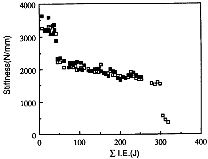
Figure 26- Stiffness vs cumulative impact energy for AS4/3501-6, (±45) 16s
