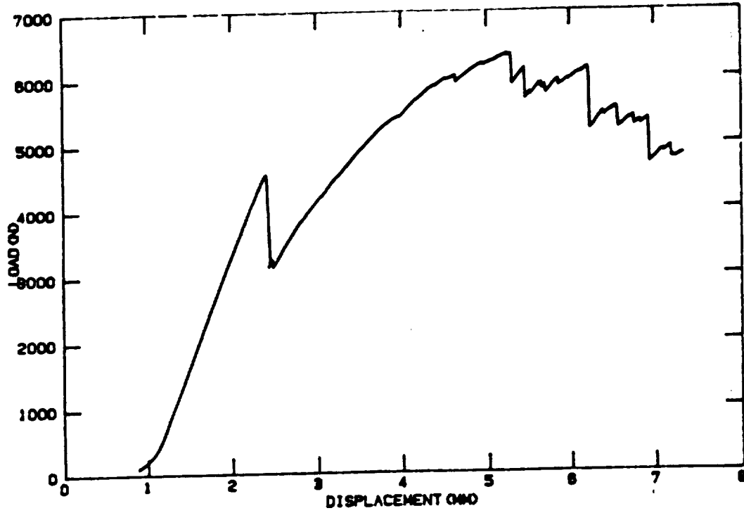
Figure 64 - Static load-displacement plot for AS4/3501-6 (0/90) 16s
