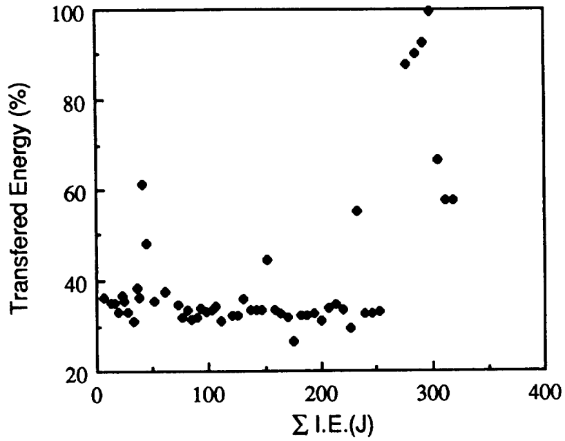
Figure 27 - Percent transferred energy vs cumulative impact energy for AS4/3501-6 (±45) 16s
