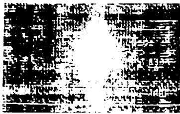
Figure 47 - C-scan of impact damage of AS4/polycarbonate, (0/90) 16s at \Sigma I. E. = 270J
