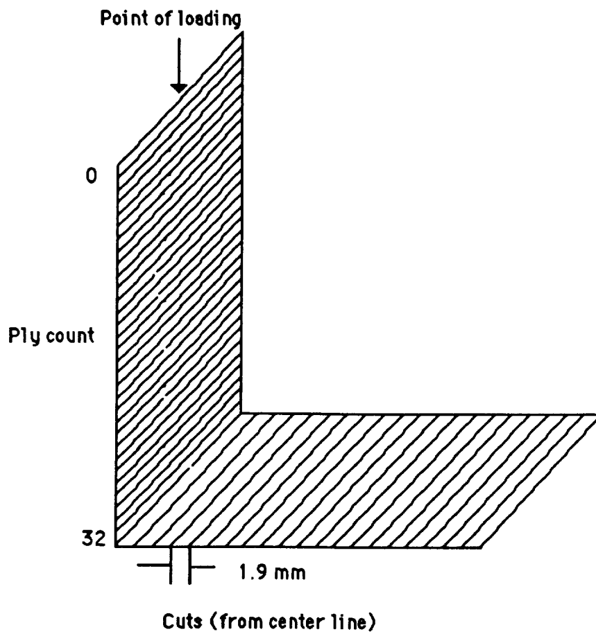
Figure 60 - Damage map of AS4/3501-6,(90/0) 16s laminate loaded to a displacement of ~ 1.5mm
