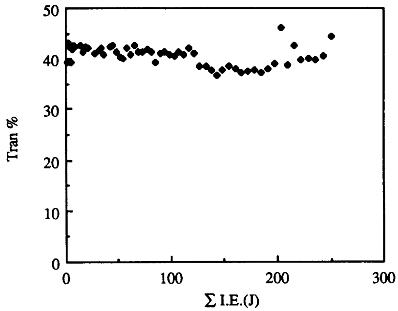
Figure 49B - Percent transferred energy vs cumulative impact energy for AS4/polycarbonate (±45) 16s
