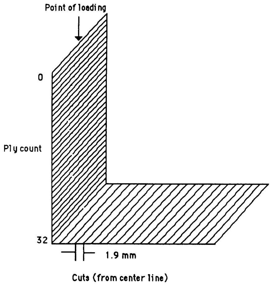
Figure 66 - Damage map for an AS4/PEEK,(90/0) 16s laminate loaded to about 2.5mm displacement
