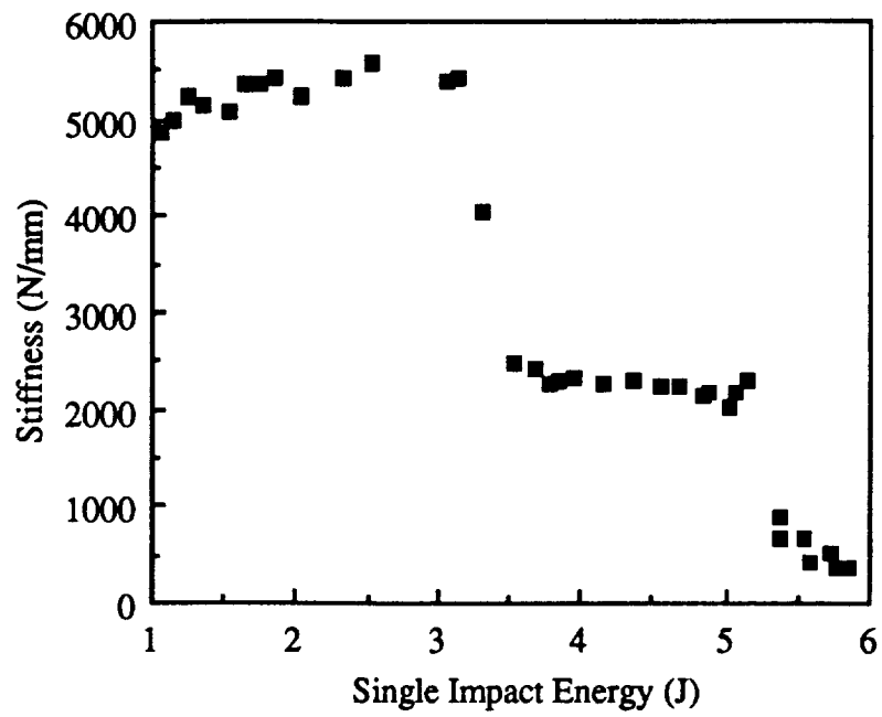
Figure 76 - Stiffness vs single impact energy for AS4/3501-6
