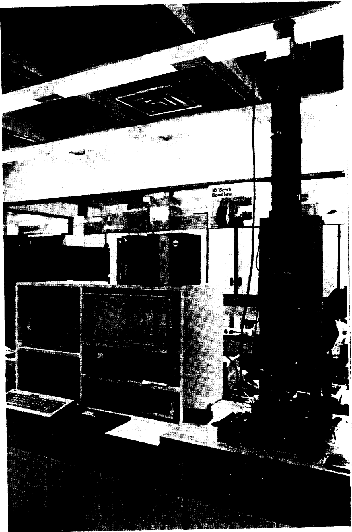
Figure 15 - Drop-weight impact test equipment.
