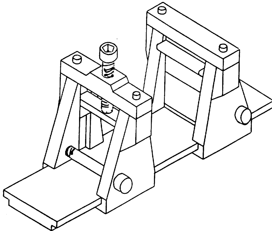
Figure 8 - Flexture load frame for Mode II delamination
