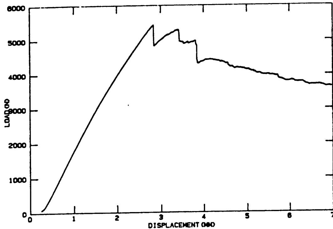
Figure 70 - Static load-displacement plot for AS4/PEEK ( \pm 45 ) 16s
