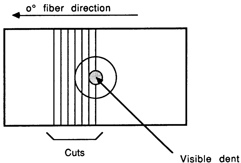
Figure 16 - Schematic of sectioning through the impact damage area.
