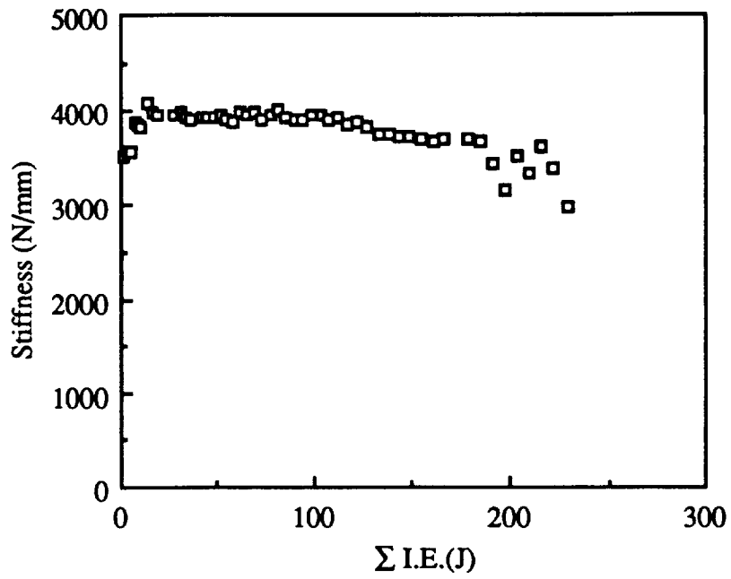
Figure 49A - Stiffness vs cumulative impact energy for AS4/polycarbonate, (±45) 16s
