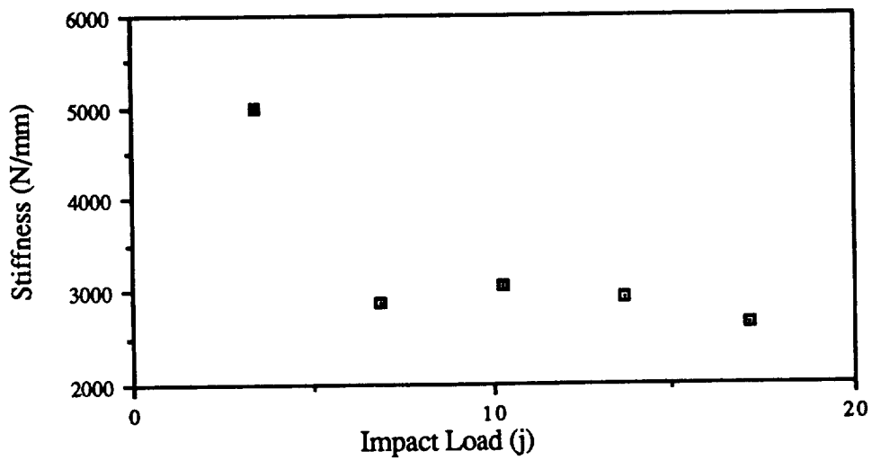
Figure 57 - Stiffness vs impact energy (noncumulative) from fatigue tests for AS4/3501-6, (0/90) 16s .
