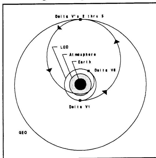
Figure 3.1 Flight Summary
