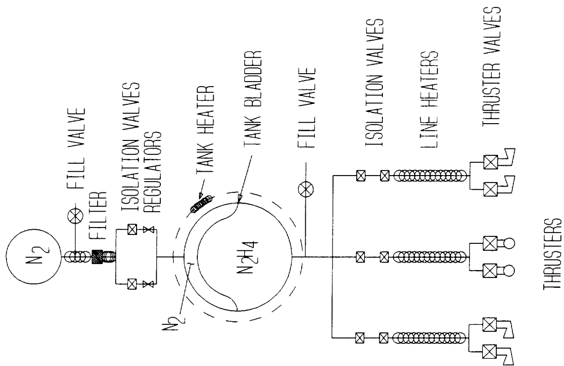
Figure 5.15 Reaction Control System Schematic
