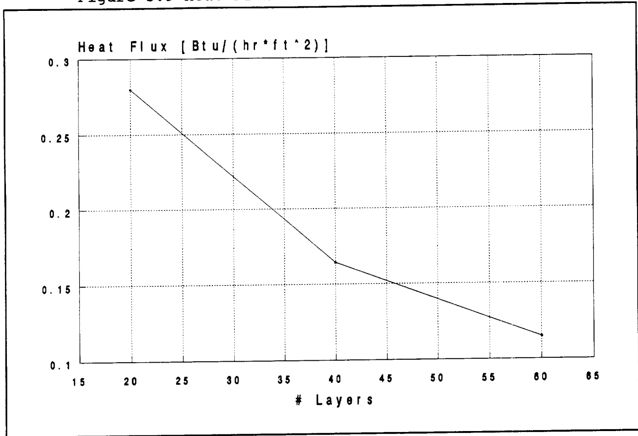
Figure 5.9 Heat Flux versus # of Insulation Layers
