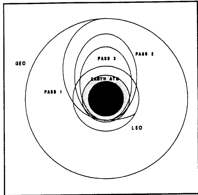
Figure 3.3 3-Pass Senario
