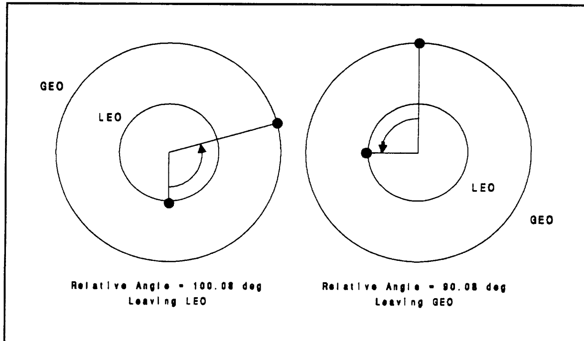
Figure 3.4 Relative Geometry
