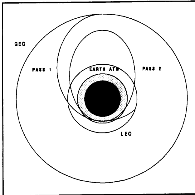
Figure 3.2 2-Pass Senario
