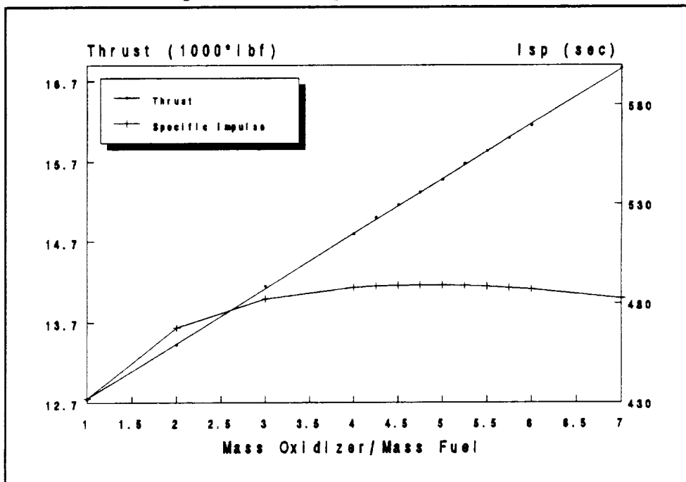
Figure 5.1 Engine Performance
