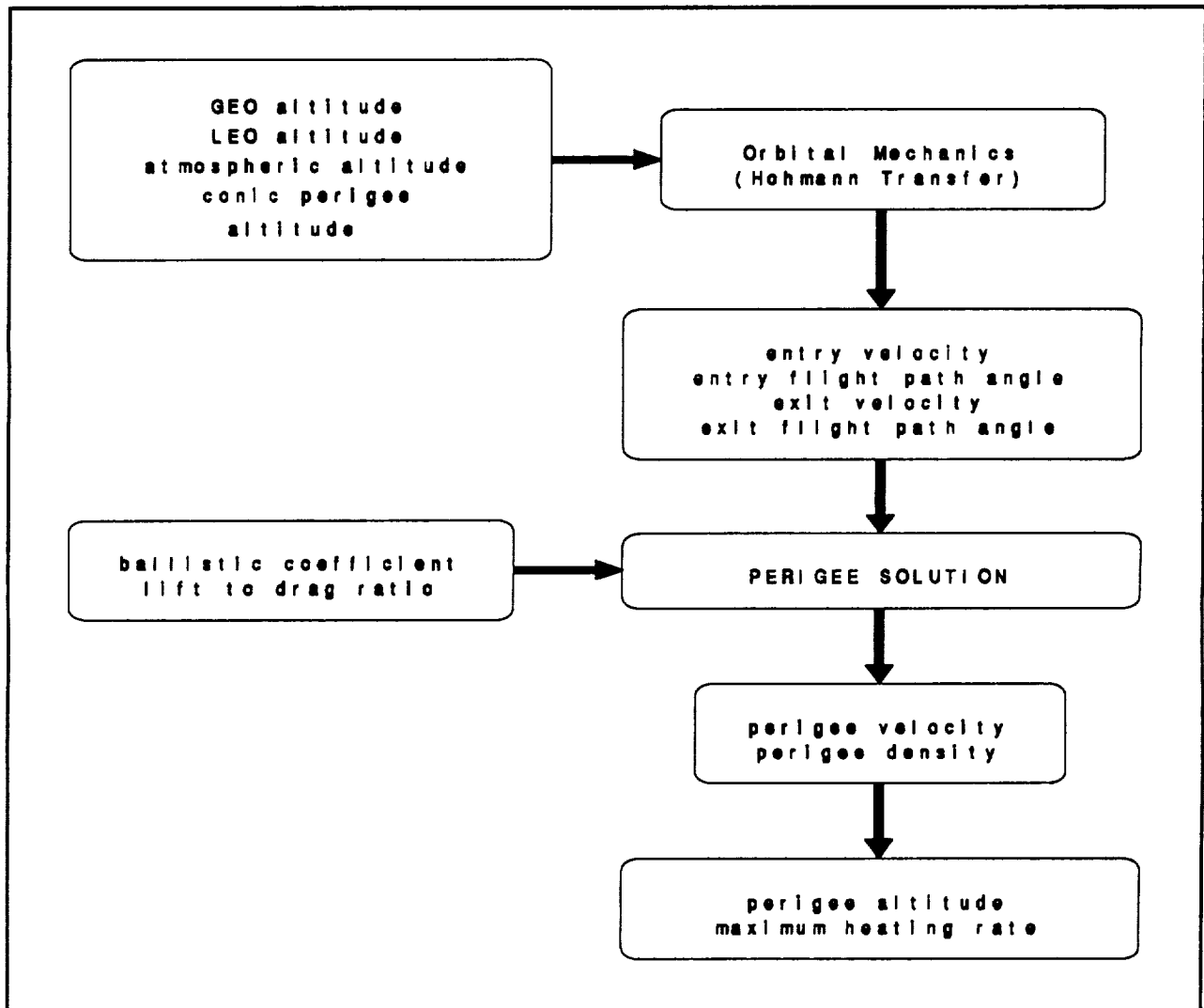
Figure 3.5 Flowchart
